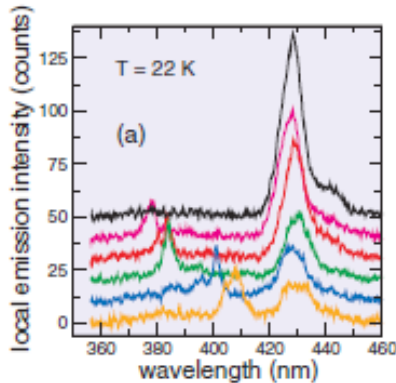
Figure 2-20: Low temperature emission spectra obtained from nm-size areas close to threading dislocations with a near field microscope 63,79 . Besides the main emission at 430 nm (black line – corresponds to the emission from the area in between the V defects) multiple sharp peaks from different locations near V-defects appear in the range 380–410 nm.
