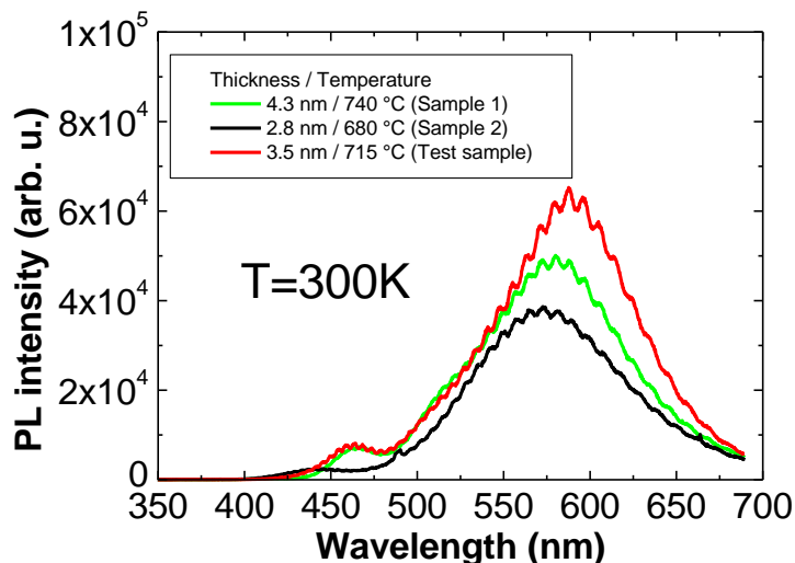
Figure 4-8: Room temperature photoluminescence of sample 1 and 2.
