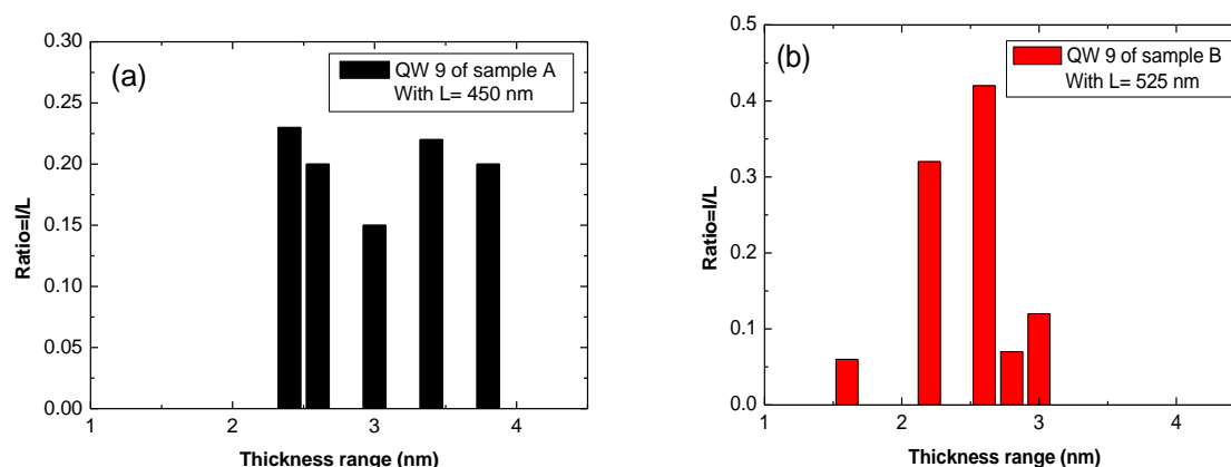
Figure 4-15 (a) Thickness distribution plot of individual quantum well number 9 for (a) sample A and (b) sample B with total observed lateral length L for the plots are 450 nm and 525 nm, respectively.
