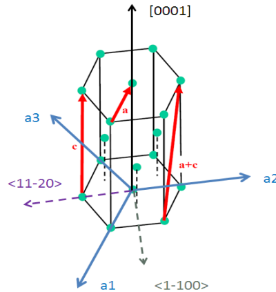
Figure 1-8: Unit cell of wurtzite structure, where the blue arrows (a1, a2 and a3) indicates the primary axes of the unit cell, the colorful dash arrows showing the particular families of direction and the red arrows shows the different types of dislocation as named beside them.
