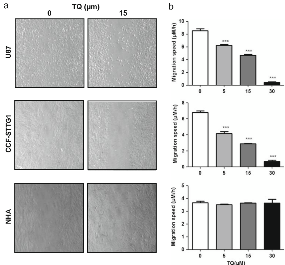
Fig. 2 TQ decreases the migration speed of U-87 and CCF-STTG1 cells but not of normal astrocytes. a Phase contrast microscopy images taken at t024 h of a wound healing assay performed on non-treated cells (0) and cells treated with 15 \mu\text{M} of TQ. Dashed lines represent the border of the lesion made at t00. Of note, the slowed migration rate observed over 24 h of TQ exposure in glioblastoma but not their normal counterpart. b Quantification of migration speed shows a dose-dependent reduction in glioblastoma cell motility after 24 h of TQ treatment
