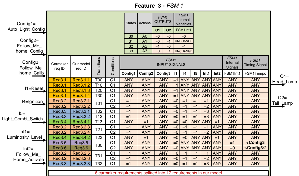
Figure 5.18 – Feature 3 modeled using a Finite State Machine element – States, Transitions and Conditions
