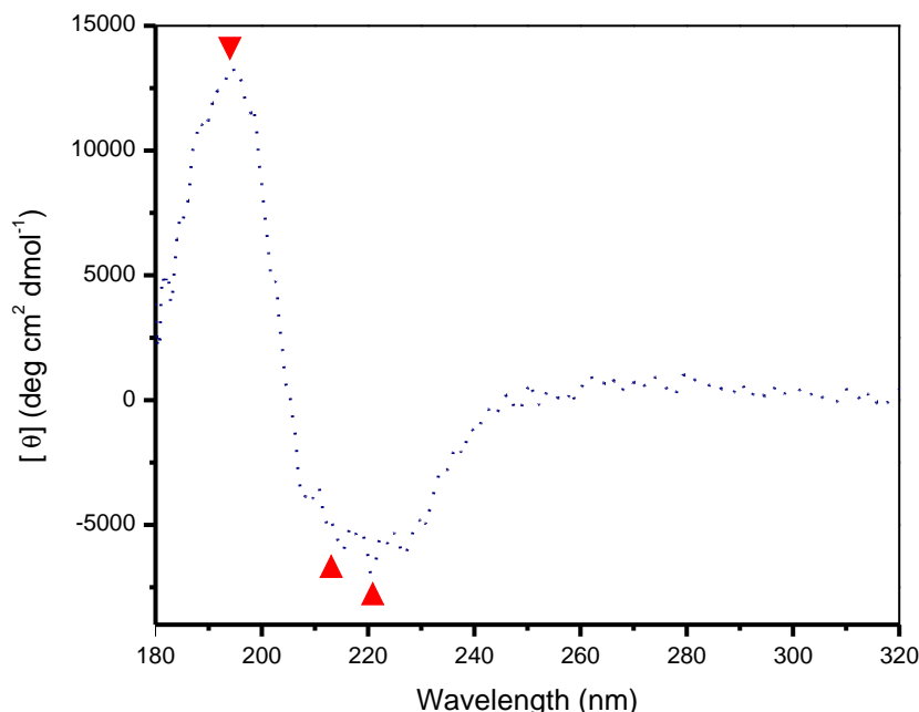
Figure 3.8: CD spectra of the film (chitosan/ \beta -lactamase) 6 on a quartz slide. \blacktriangle \blacktriangledown point out the characteristic adsorption bands.
