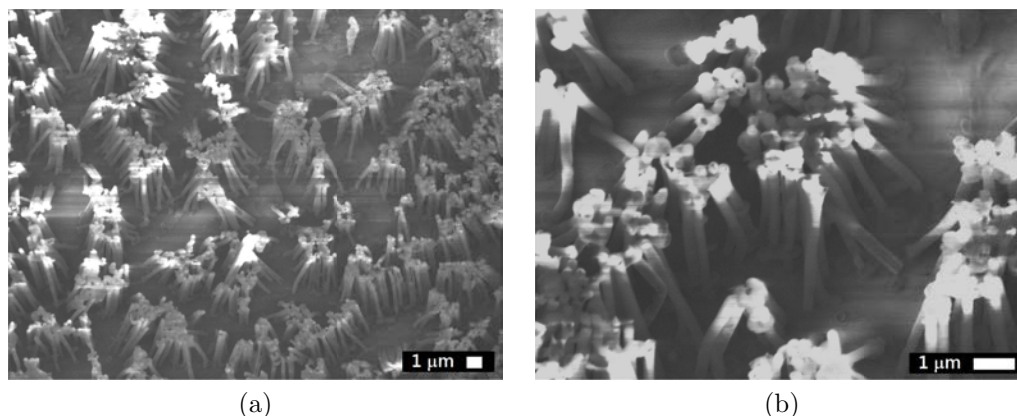
Figure 4.8: SEM images of brushes of nanotubes (\text{PAH/PAA})_{12} prepared by LbL deposition combined with hard-templating and crosslinking. The samples were decrusted by polishing with alumina powder.
