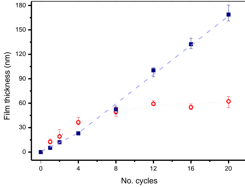
Figure 3.3: Evolution of film thickness as a function of the number of cycles (\text{chitosan}/\beta\text{-lactamase})_n on flat films (■) and filled pores in PCm (○). Error bars correspond to the range of thickness values measured for at least two independent experiments. Dashed and dotted lines are guides to the eye.
