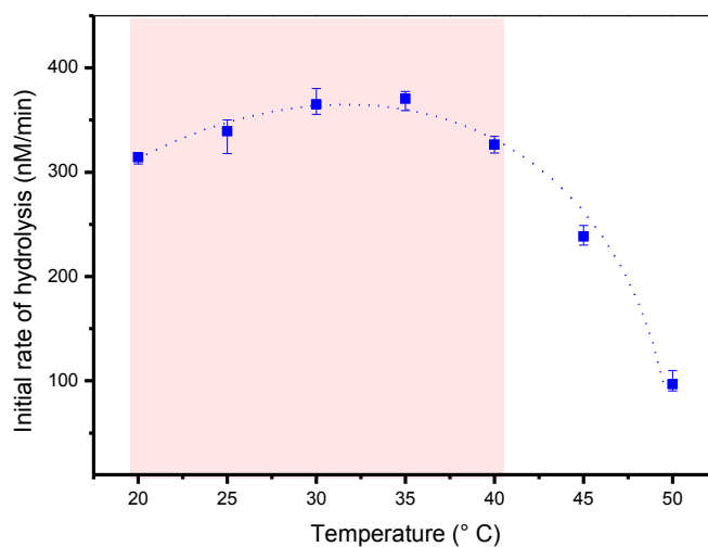
Figure 5.8: Temperature - activity curve of nitrocefin hydrolysis by (chitosan/ \beta -lactamase) 4 films in MES 0.1 M pH 6.5. The red area considers the range of working temperatures for thermo-responsive films. Error bars correspond to the range of values measured on triplicates.
