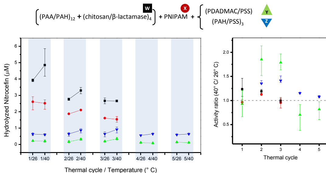
Figure 5.21: Influence of PNIPAM* on the activity of the nanotube brushes at 26 and 40 °C, along 5 thermal cycles. Left: Activity response. Right: Ratio of activity response (Activity at 40 °C/activity at 26 °C). Error bars correspond to the range of values measured on duplicates.
