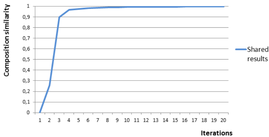
Figure 6.2: Average top 100 shared results among iterations n - 1 and n , monocentric queries
