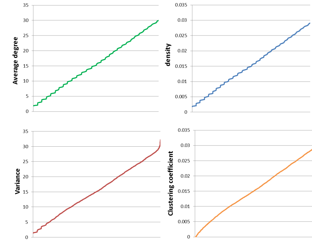
Figure 6.18: Principal metrics of the random graphs
