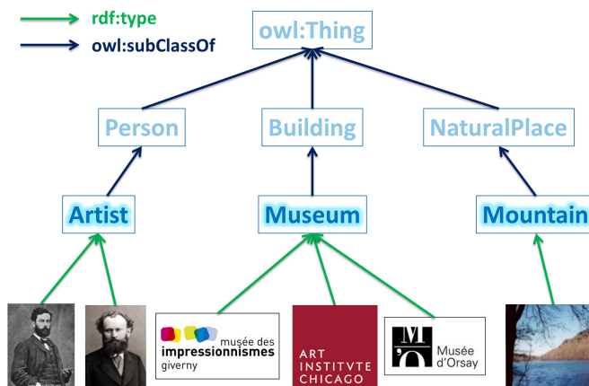
Figure 5.3: During the class propagation domain computation the first step is to identify the neighbors' deepest types
