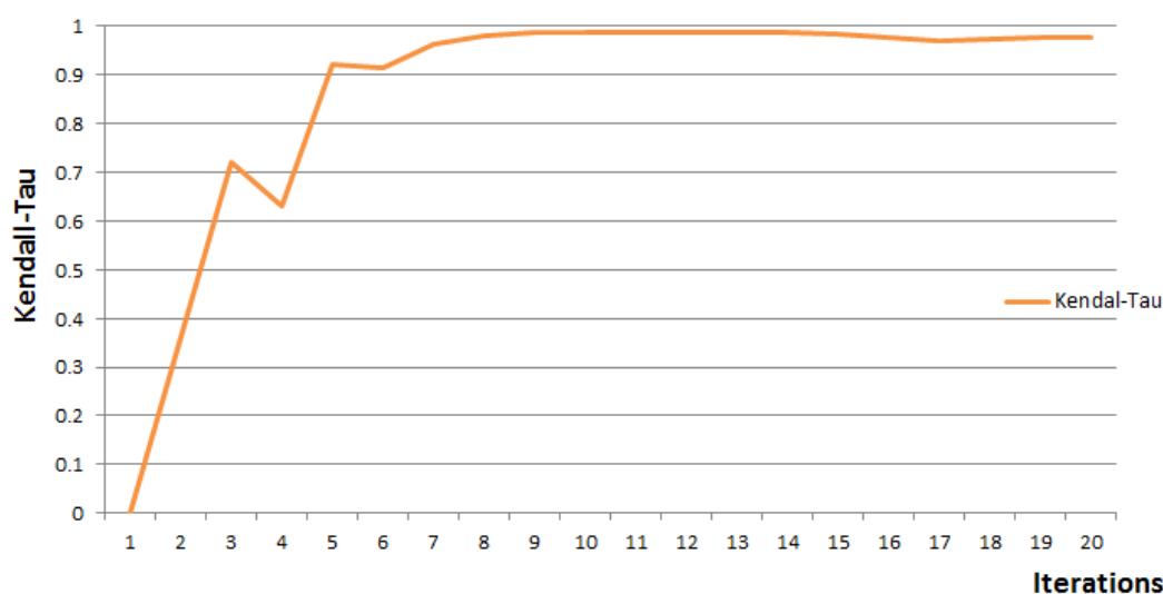
Figure 6.25: Kendall-Tau of the 100 shared result from one iteration to another ( n - 1, n ) according to the graph diameter, Digg analysis-case
