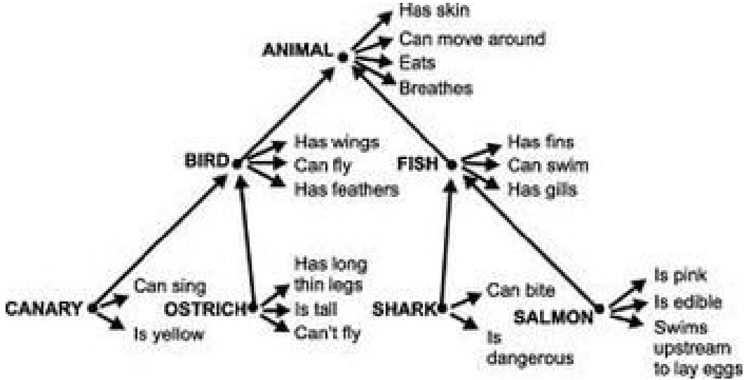
Figure 5.1: Original illustration of the memory semantic network by Collins and Quillian in their Retrieval time from semantic memory article [32]
