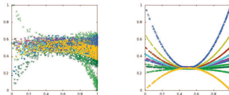
(a) A correlation pattern from beta-cubic distributions (b) A correlation pattern from beta-quadratic distributions
