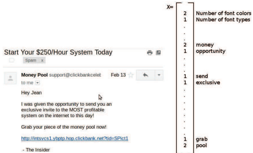
Figure 2.2: Vectorial representation of an email. The image on the left is a screenshot of a spam email and on the right its corresponding feature vector ( x ) is presented.
