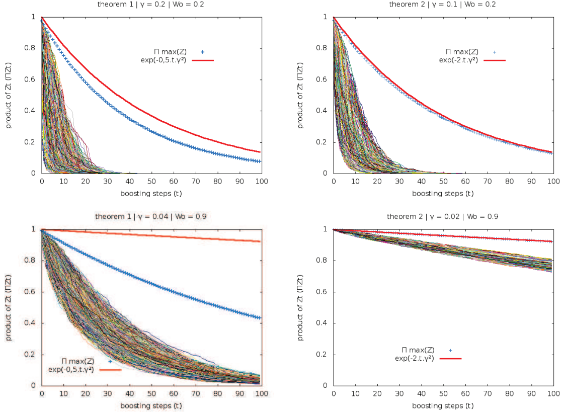
Figure 4.1: Evolution of \prod_{t=1}^T Z_t following the two possible strategies for different values of W_0 : Theorem 4.2 (left) and Theorem 4.3 (right); W_0 = 0.2 (up) and W_0 = 0.9 (down).
