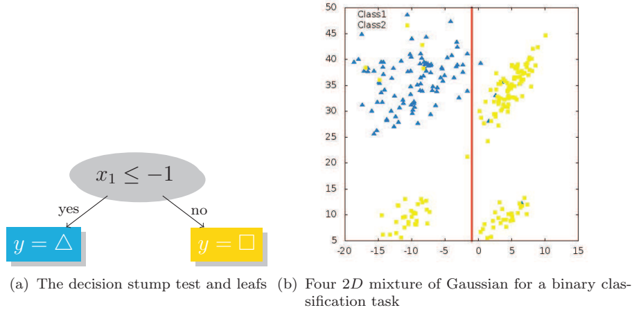
Figure 2.5: An example of a decision stump
