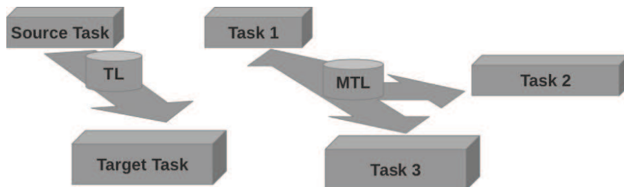
Figure 2.8: Information flow. In transfer learning, the information flow in one direction only. In multi-task learning, information can flow freely among all tasks.
