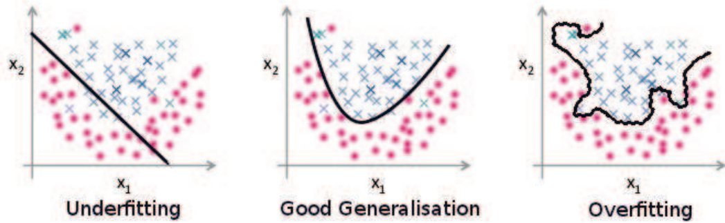
Figure 2.1: Overfitting and Underfitting in binary classification. From the left to the right we allow more and more complex functions to be learned. Left: the function family is too simple to fit the training data. Right: the function family is too complex, the learned function is tailored to the training data. Middle: a good compromise between underfitting and overfitting.
