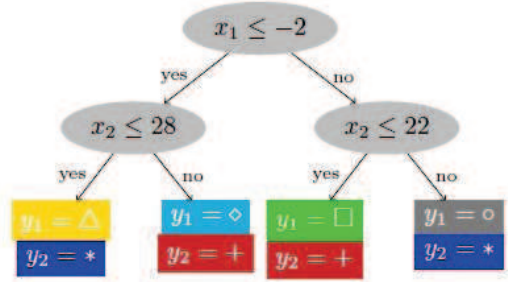
(a) MT-DT with early decision leaf
