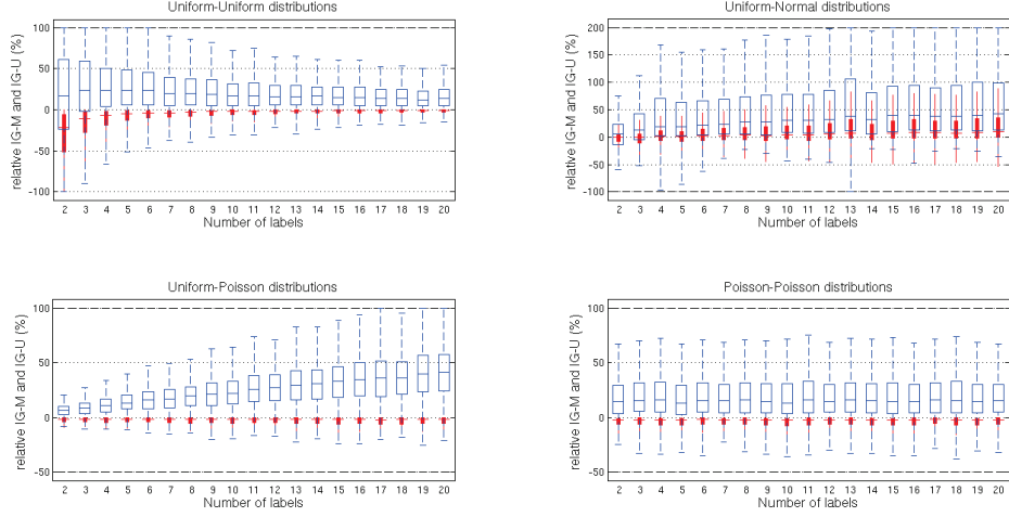
Figure 4.2: Information gain for synthetic two-task datasets. The relative values of IG_M (in blue) and IG_U (in red).
