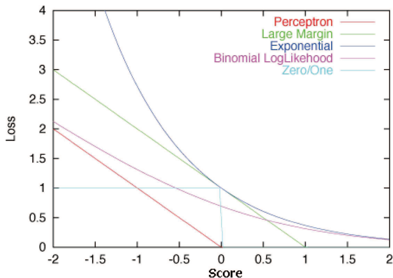
Figure 2.3: Common loss functions used to upper bound the 0\1 loss. Each curve represents a loss function for binary classification, such a function depends on the score y \cdot h(x) that should be positive.
