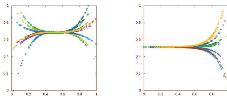
(c) A correlation pattern from gaussian-cubic distributions (d) A correlation pattern from gaussian-exponential distributions
