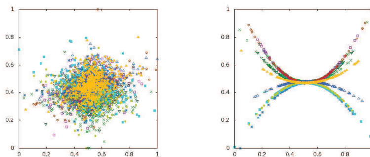
(g) A correlation pattern from laplace-linear distributions (h) A correlation pattern from laplace-quadratic distributions
