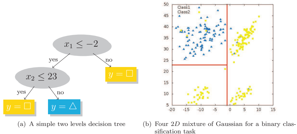
Figure 2.6: An example of a decision tree
