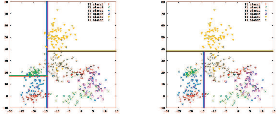
(a) Visualization of the partition defined by the 2T-stump in Figure 3.1(a). It is learned on the synthetic dataset with algorithms WL-Best-K with K = 5 or WL-Best-K with K = 25 . The score W_- + \frac{1}{2}W_0 is equal to 0.134 (b) Visualization of the partition defined by the 2T-stump in Figure 3.1(b). It is learned on the synthetic dataset with a naive greedy algorithm. The score W_- + \frac{1}{2}W_0 is equal to 0.197
