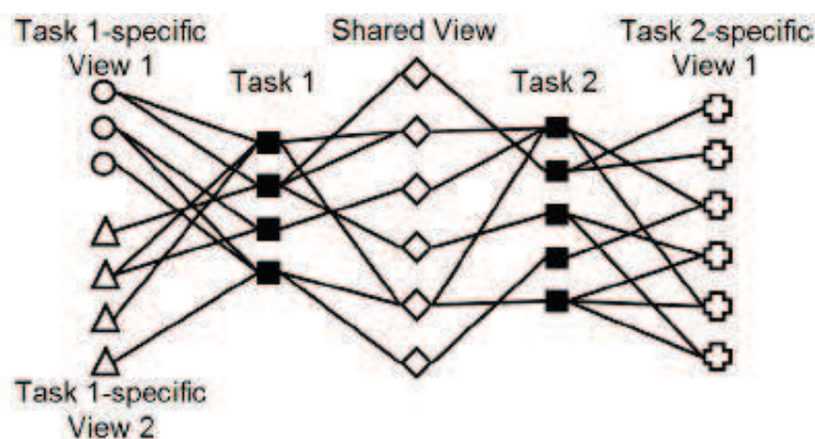
Figure 2.10: Graph-based approach to multi-task. Examples from Task 1 and Task 2 (black squares) have both a shared view (diamonds) and the task specific views (circles and triangles for the 2 views of Task 1, and pluses for the 1 view of task 2). The weight of an edge between an example node and a feature node is set to the feature value.
