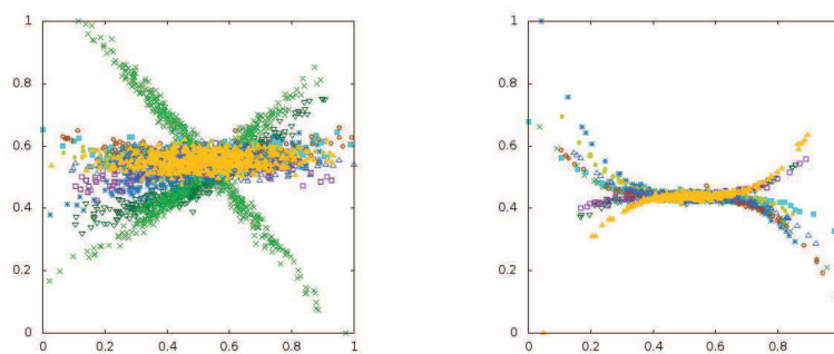
(e) A correlation pattern from gaussian-quadratic distributions (f) A correlation pattern from laplace-cubic distributions
