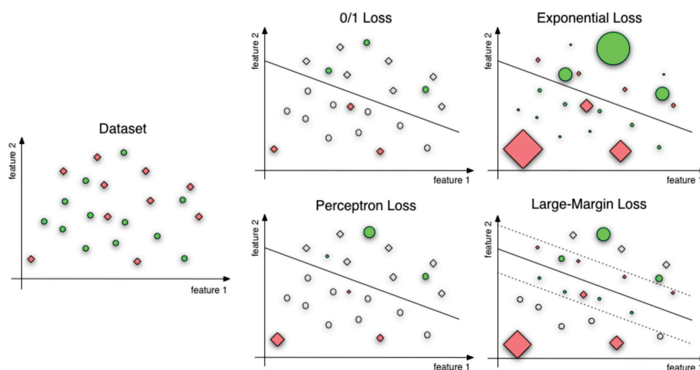
Figure 2.4: Losses illustrated on a binary classification task. Empty shapes correspond to examples with a 0 loss. Otherwise, the size of the filled shapes reflects the amount of loss the examples suffer from. In this example, ideally, all the green circle examples should be below the line and the red square examples should be above
