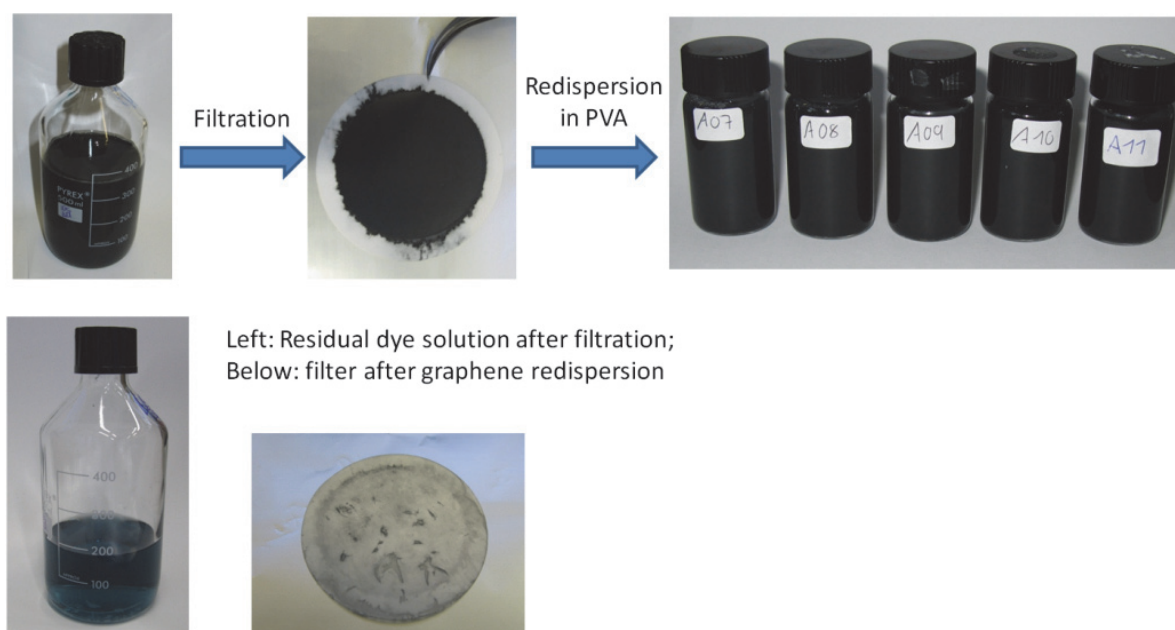
Fig. 7. Process for preparation of graphene/IBS in polymer dispersion with filtration and redispersion in a 4% aqueous Poly(vinyl alcohol) Mw 9,000-10,000, 80%hydrolyzed (PVA10) solution. Below: Aqueous residual containing excess indanthrone. Filter after redispersion.
