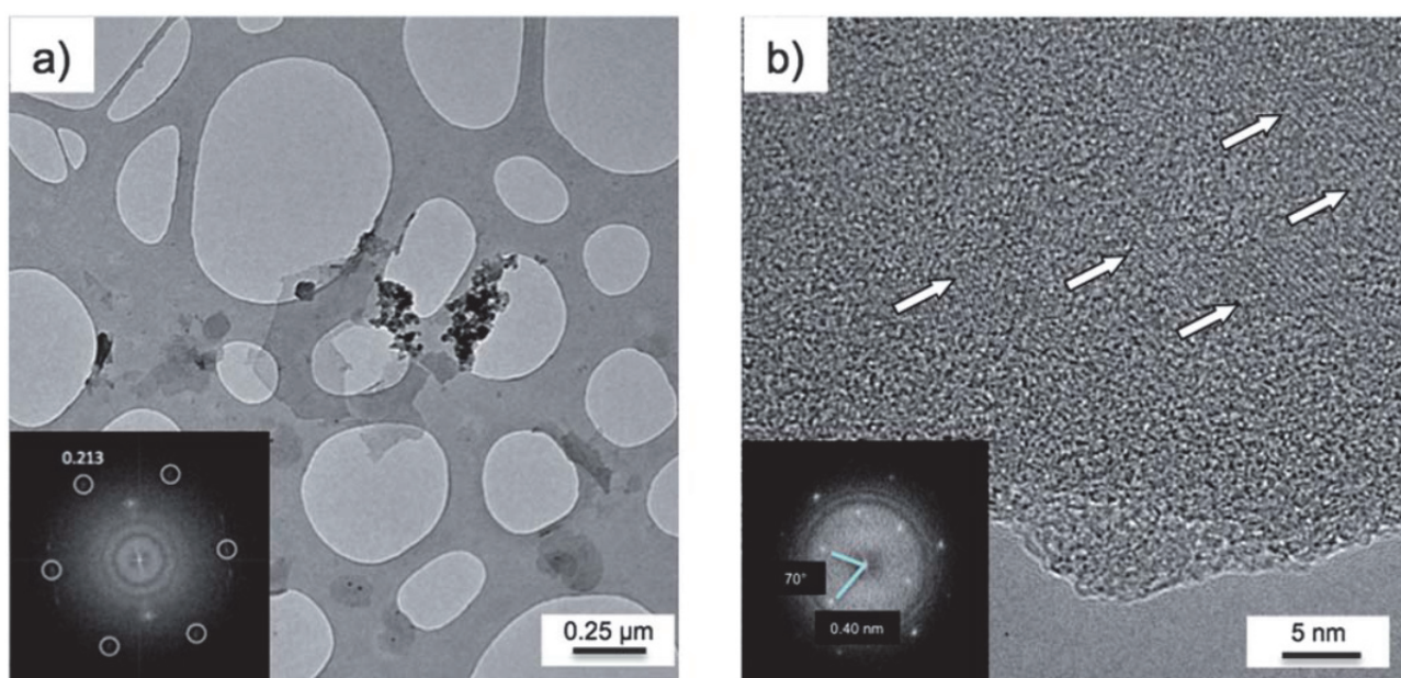
Fig. 4. TEM image of graphene sheets exfoliated with PS2. In the inset, the typical SAED pattern of graphene is shown. (b) Zoom-in on a sheet, showing ordered areas with a packing different from the one observed for graphene (SAED measurements are shown in the inset).
