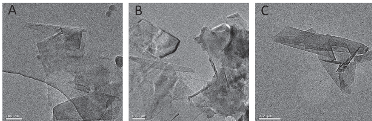
Fig. 4. Selected TEM images of flakes prepared by PS1assisted exfoliation of graphite. (A) A few-graphene layers flake (probably a folded bilayers); (B) A thin (on the left) and thick (on the right) flake. (C) A folded and wrinkled flake: most of our flakes have folded and wrinkled area.
