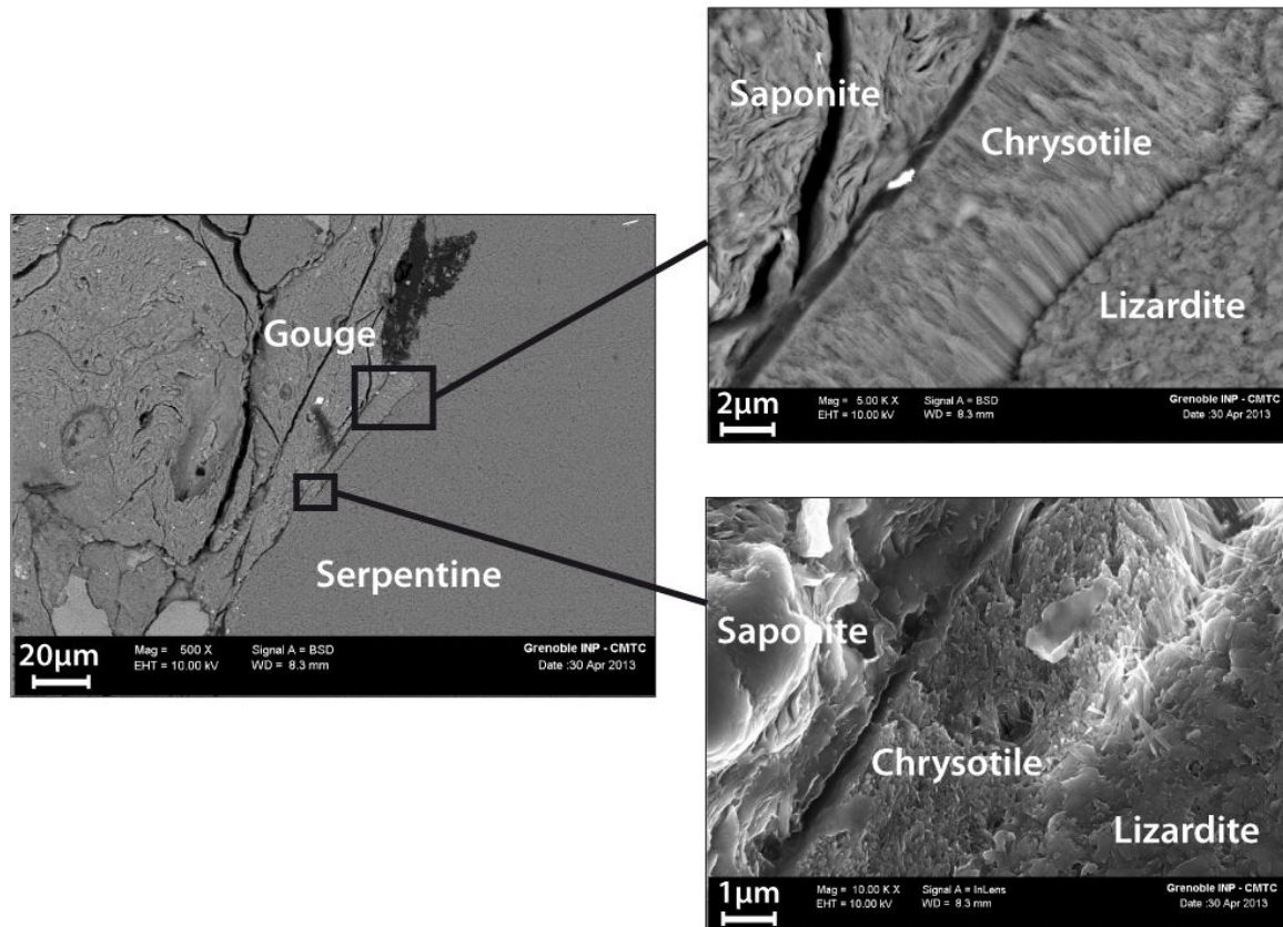
Figure 6: Examples of two different serpentines. The three pictures are FEG-SEM images, taken from sample III-0 at the boundary between an aggregate mainly composed of serpentine and saponite clay. Most of the serpentine forming clasts or present in the aggregates is lizardite. Chrysotile is located mainly along the boundaries of the serpentine aggregates or clasts, as here.
