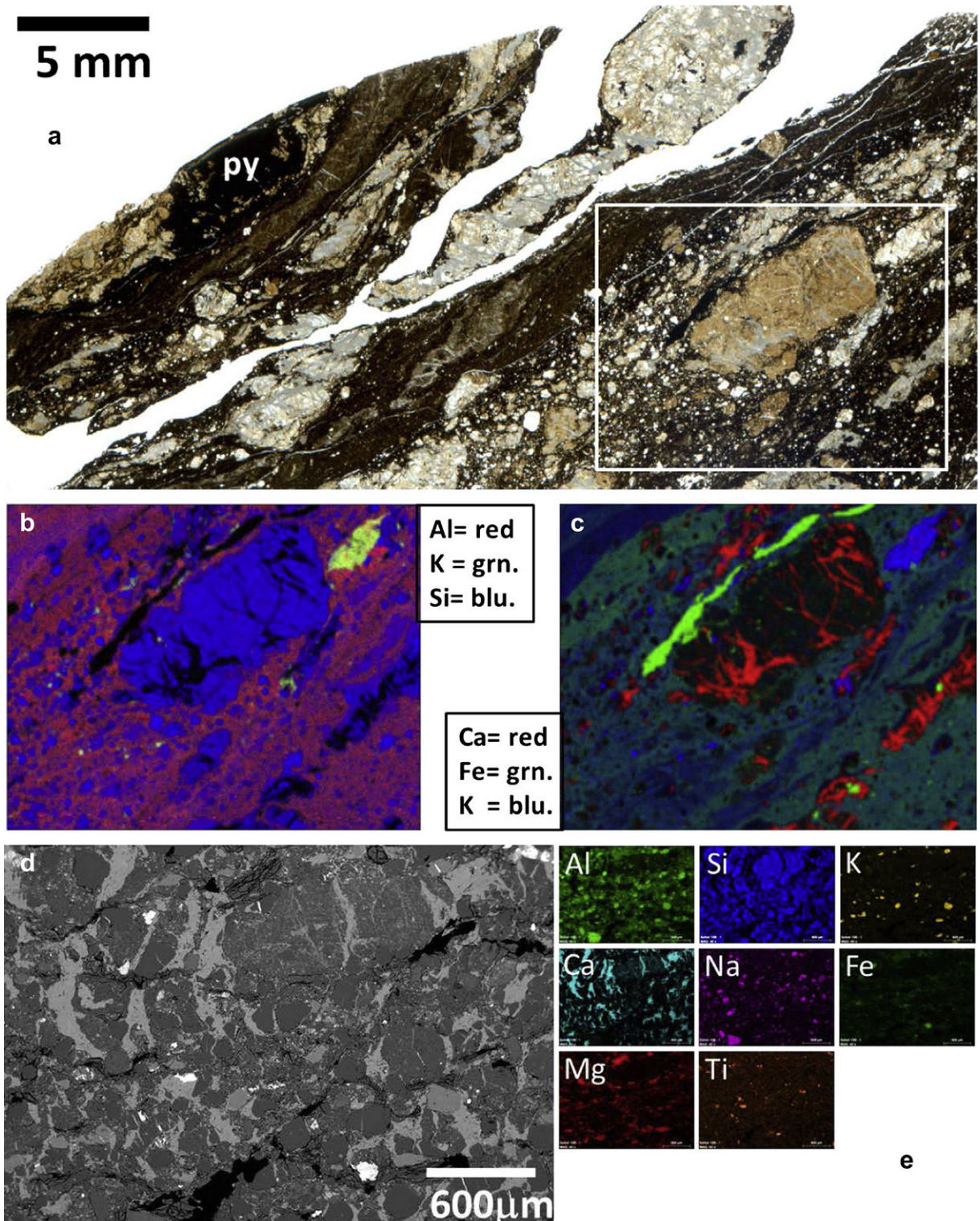
Fig. 5. Well-developed foliation in siltstone-shale cataclasites typical of the core zone rocks. (a) The foliation is defined by interlaced bands of siltstone-rich gouge and dark-colored clay-rich gouge. Siltstone clasts consist of variably healed cataclasites. A mass of deformed pyrite (py) forms an inverted sigma that indicates dextral sense of shear in the sample. (b) Distribution of Aluminum in XRF elemental map for inset area in the foliated gouge indicates pervasive clay mineralization. (c) XRF elemental map from the same area shows pattern of the transverse calcite veins in a quartz-rich band and reveals smearing of pyrite along foliation. Sample G24. (d) SEM backscatter image of fully-developed vein-cleavage pressure solution foliation in the core zone, ~1 m distance from the CDZ boundary. Sample G42. (e). XRF elemental maps of the area shown in d.
