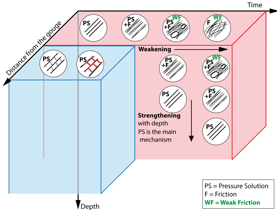
Figure 12: Model of a creeping fault zone showing the change in mineralogy as a function of time, depth and creeping zone distance. The blue domain corresponds to the creep mechanism observed in the damaged zone, in the samples outside the creeping zone. In this domain, pressure solution creep is the main creep mechanism. Healing by calcite precipitation allows this mechanism to be maintained with time as well as at depth. The red domain corresponds to the creep mechanisms observed in the active creeping zone. Pressure solution creep is very efficient at the beginning at all depths. However, because there is no or little healing in this domain because fluids drive away the dissolved materials, the mineralogical composition evolves with time leading to increasing clay content in the upper 3-4 km. The friction coefficient of the creeping domain becomes very low and the sliding of clay layers on top of each other could accommodate a substantial part of the creeping rate. It is completed by stress-driven diffusive mass transfer that accommodates the sliding of grains and clast aggregates. Low friction related to saponite is not operative below 3-4 km because of the transformation of saponite into corrensite then chlorite, which have higher friction coefficients. When saponite starts to transform into harder minerals with the increase in temperature, the entire domain becomes stronger and more difficult to deform by friction. Diffusion-accommodated grain-sliding pressure solution creep remains efficient and is the main creep mechanism at depth.
