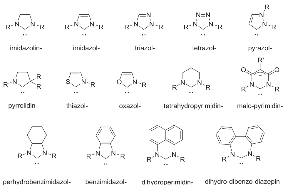
Figure 6. Common families of NHCs (the suffix "ylidene" should be added to obtain the complete name of each family)
