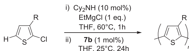
Scheme 44. Ni–NHC-catalyzed polycondensation of thiophenes
