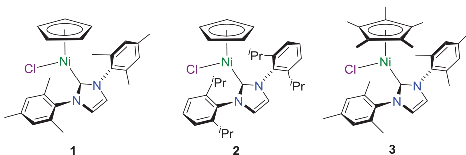
Figure 2. Selected half-sandwich NHC-nickel complexes
