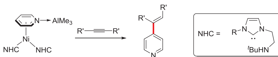
Scheme 34. Ni–NHC–pyridine active intermediate
