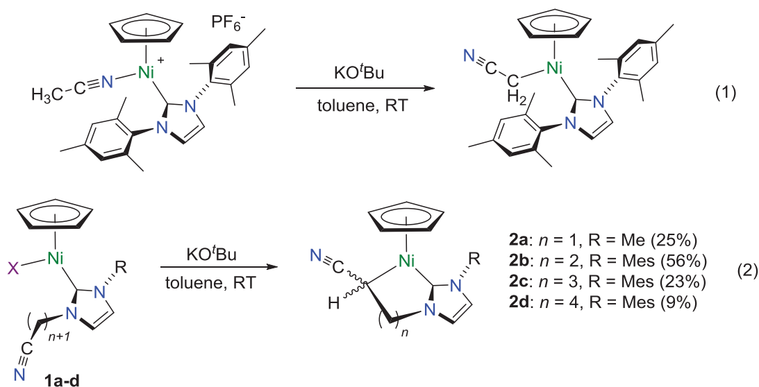
Scheme 1. Base-assisted C–H activation of acetonitrile and alkylnitrile-NHC side arms in CpNi–NHC complexes
