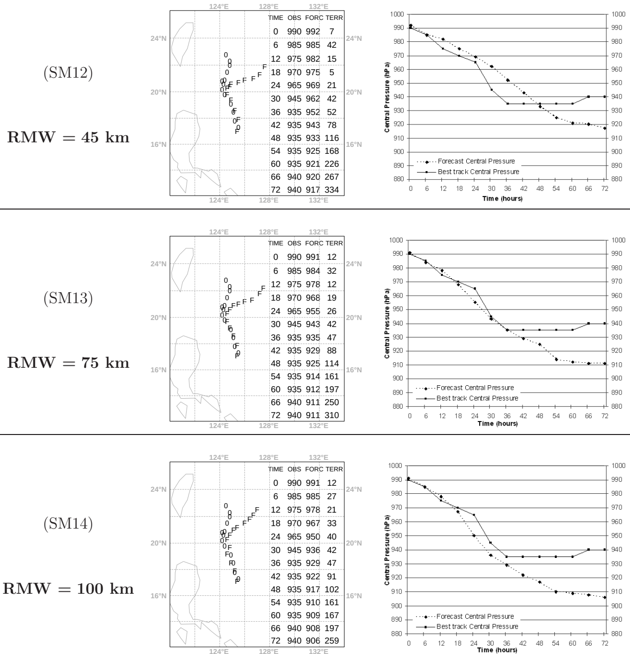
FIG. 5. Typhoon Sinlaku observed (O) and predicted (F) track (left) and central pressures (right) from base time 0000 UTC 9 Sep 2008. The 0.15^\circ -resolution 72-h forecasts (SM12, SM13, and SM14) are initialized with R_{34} = 280 km and different RMW values as indicated. Column values in track panels (at left) display estimated (OBS) and forecast (FORC) central pressures in hPa, as well as track errors (TERR) in km at 6-h intervals. Best track data is obtained from IBTrACS.
