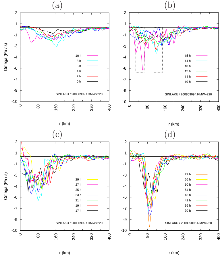
FIG. 15. Radial profiles of mean omega ( \text{Pa s}^{-1} ) at the 0.975 \sigma -level at various lead times into the SS18 forecast (RMW = 220 km). Omega is azimuthally averaged at each radii. Rectangles in panel (b) highlight the two regions of ascent that are present in the boundary layer, the outer one being located around the RMW. These two regions are still evident in panel (c) although closer to each other; they eventually merge in (d).
