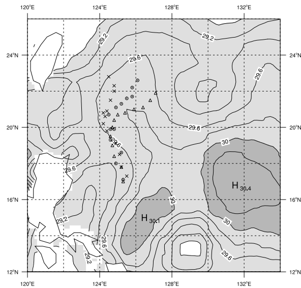
FIG. 11. Sea surface temperature field in TC-LAPS obtained from a weekly collection of satellite and ships observations during the period 1-7 Sep 2008. Contour intervals are 0.2^\circ\text{C} ; light (dark) shading indicate values between 29.0 and 30^\circ\text{C} (greater than 30^\circ\text{C} ). The location of the storm center at 6-h intervals from 0000 UTC 9 Sep to 0000 UTC 12 Sep 2008 is indicated by a marker (a cross for IBTrACS data, a triangle for SS15, an encircled cross for SS18).
