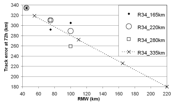
FIG. 7. 72-h forecast track error (km) vs initial RMW (km) for 0.15°-resolution experiments SM6 to SM18 (Table 1). Experiments are classified by groups of initial R34 values as indicated in legend.
