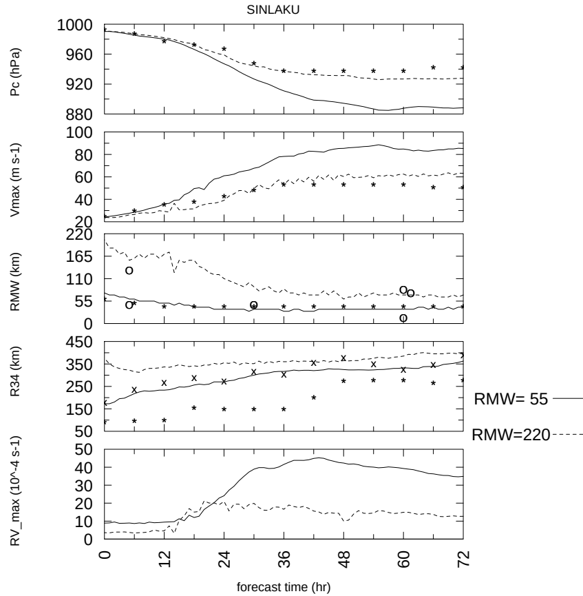
FIG. 12. Time series of storm parameters for experiments SS15 (RMW = 55 km, solid line) and SS18 (RMW = 220 km, dashed line). Asterisks denote estimated values of p_c and VMAX (best track data from Tokyo-Typhoon Center), of RMW (real-time estimates from Darwin Tropical Cyclone Warning Centre), and of R34 (best track data from the Joint Typhoon Warning Center, sole provider) for Typhoon Sinlaku. Circles show RMW estimates from aircraft missions. Crosses indicate R34 values calculated from Weber's statistical model. Predicted values of maximum vertical relative vorticity ( RV\_max , 10^{-4} \text{ s}^{-1} ) are displayed in the bottom panel.
