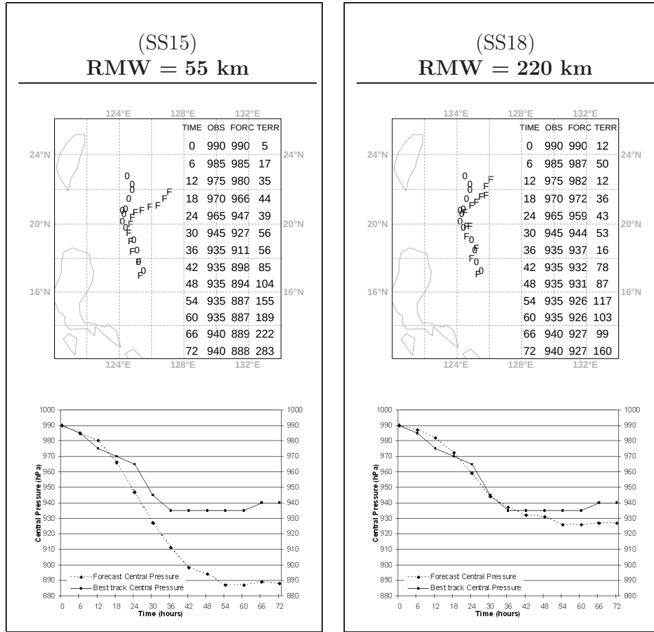
FIG. 10. As in Fig. 5, but for 0.05^\circ -resolution forecasts SS15 and SS18 ( R34 = 335 km and different RMW values as indicated in legend).
