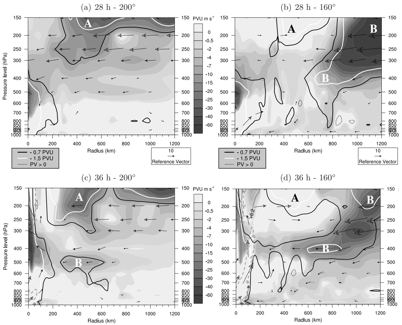
FIG. 8. Radius-pressure cross sections of negative values of PV radial advection -uPV ( PVU \times m s^{-1} , shaded) after (top) 28 h and (bottom) 36 h of simulation and along (left) 200^\circ and (right) 160^\circ azimuth (cross sections are delineated on horizontal maps in Fig. 7). Superimposed are PV contours of -0.7 , -1.5 and 0.2 PVU. The TC center is located at the left. Arrows represent the radial and vertical ( -10 \times \omega ) wind vectors. Dashed grey contours indicate regions of vertical velocity lower than -2 Pa s^{-1} . Labels “A” and “B” as in Fig. 7.
