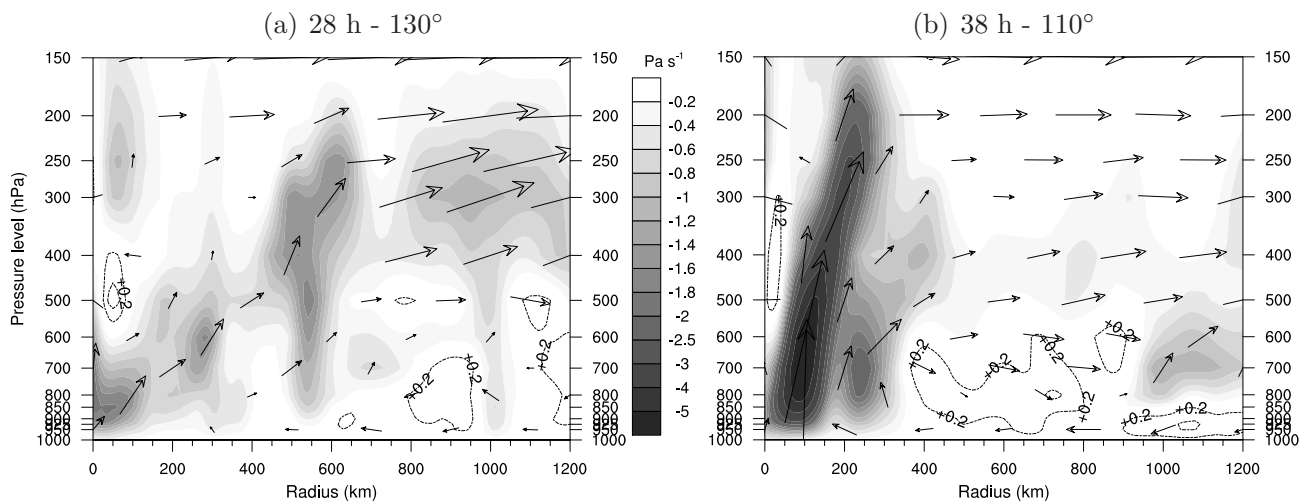
FIG. 9. As in Fig. 8 but for the vertical velocity field ( Pa s^{-1} ; negative, shaded; positive, dotted contours) at (a) 28 h and (b) 38 h, in the east-southeastern sector of the storm.
