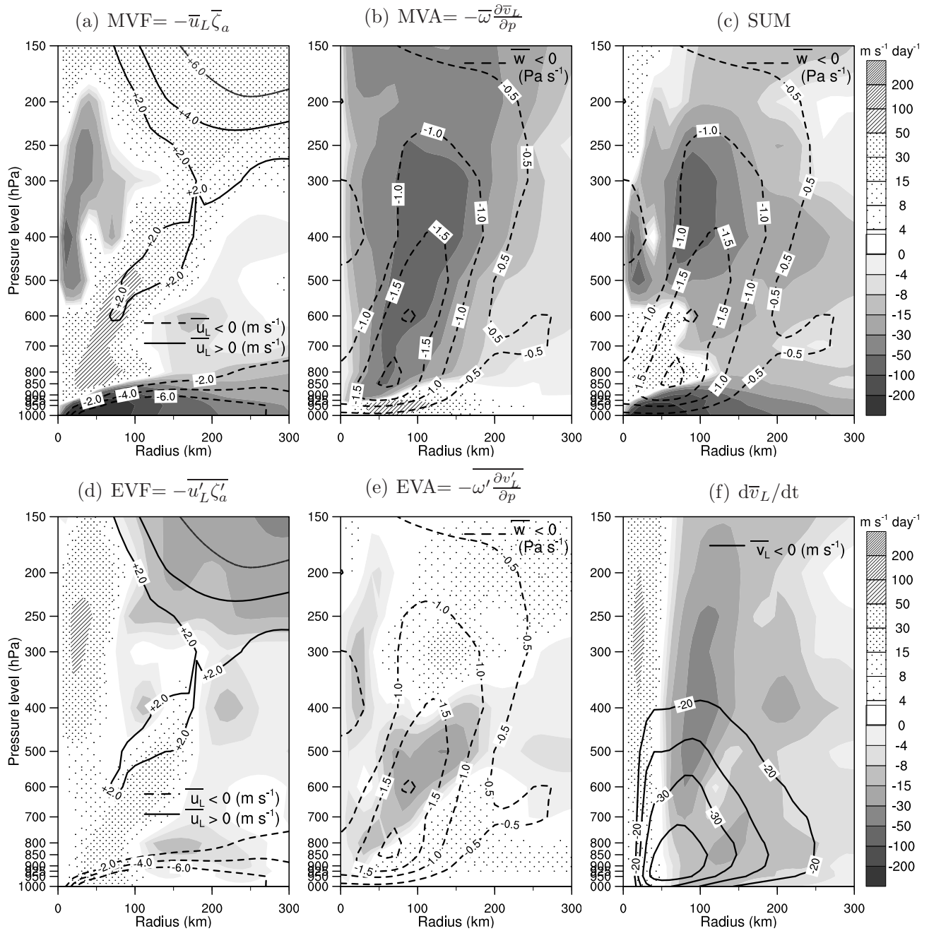
FIG. 15. As in Fig. 14, except from 37 to 41 h.
