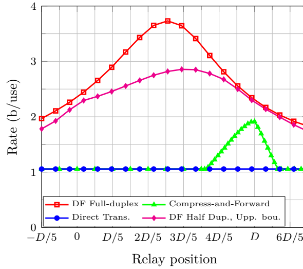
Figure 5.7: Maximum rate achievable through all the studied protocols when the relay is aligned with the source and destination and an OP smaller that 0.05 is required. The OP of full-duplex DF comes from Theorem 5.2, half-duplex DF from Theorem 5.5, CF from Theorem 5.7 and DT from (5.40). The Laplace transforms are numerical from Lemma 5.1. d = (10, 0) , \alpha = 4 .
