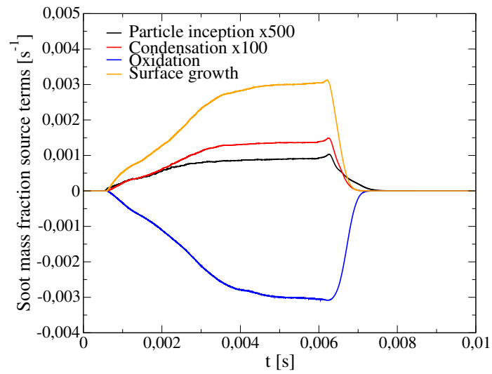
Figure 5.15: Time-evolution of the particle inception, condensation, surface growth and oxidation source terms for the reference case.
