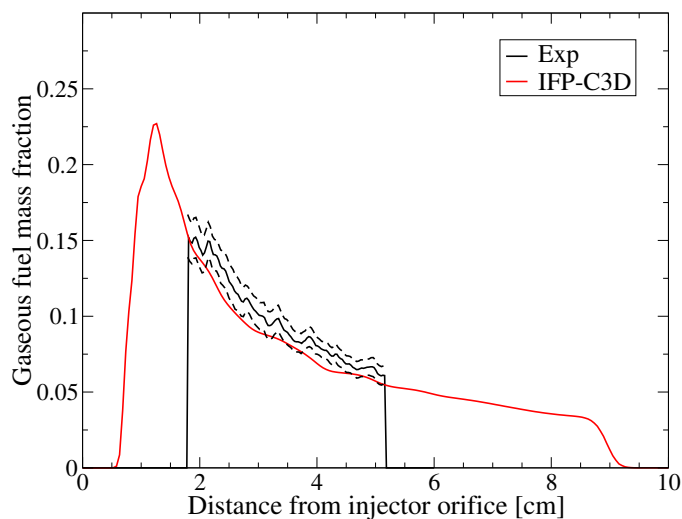
Figure 5.5: Comparison between experimental (black with standard deviation in dashed line, available in a limited range of distances from injector orifice) and simulated gaseous fuel mass fraction along the spray axis depending on the distance from the injector orifice.
