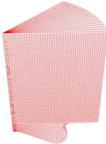
Figure 4.17: Visualization of the computational mesh at 30 CAD
