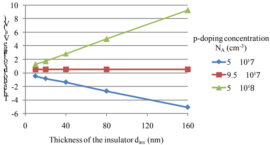
Figure 4.17 Variations of the threshold voltage with the thickness of the insulator at various p-doping concentrations
