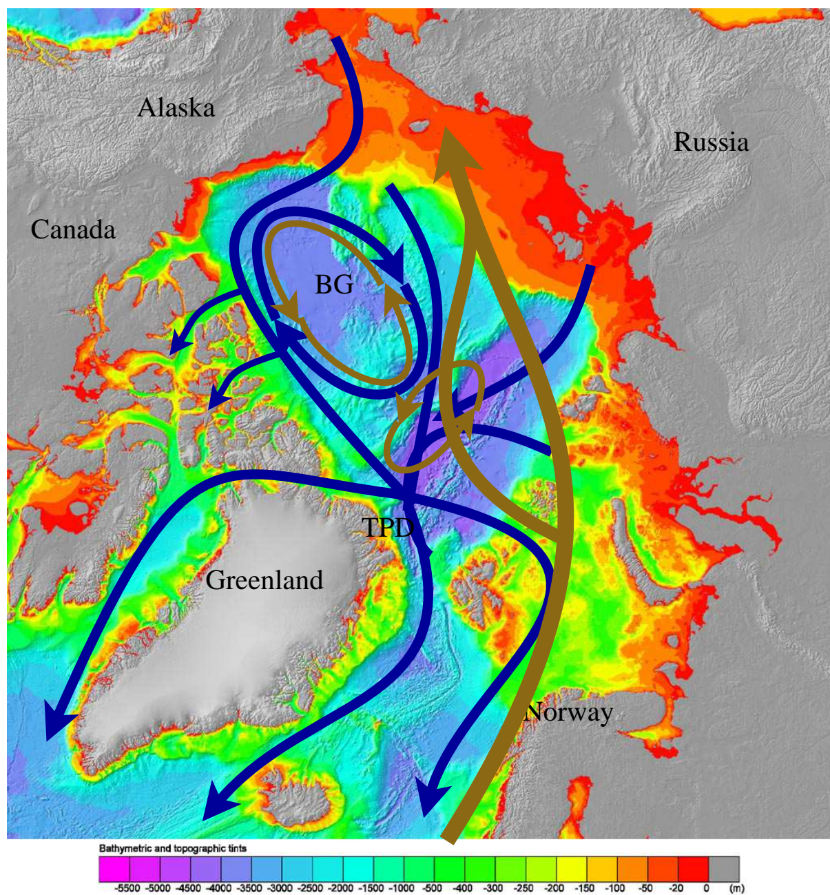
Figure 2.2: Circulation patterns in the north Atlantic and the Arctic Ocean. Brown arrows are the inflow north Atlantic and the Arctic surface circulation. Blue arrows are the inflow from Pacific and the outflow of the Arctic water to the North Atlantic. The background map is from http://www.ngdc.noaa.gov/mgg/bathymetry/arctic
