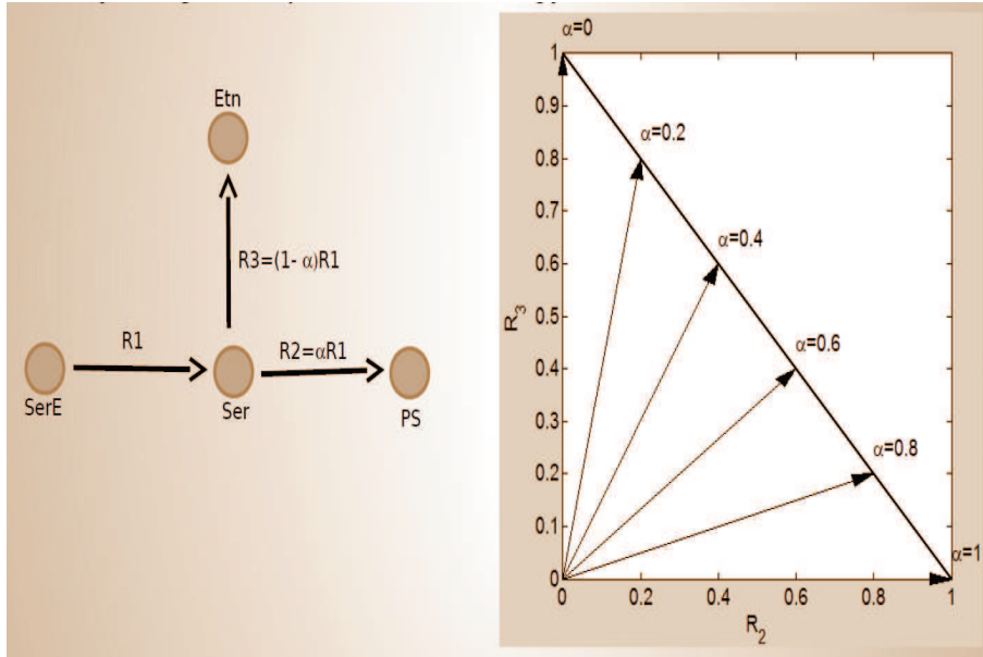
Figure 16: The figure shows discretization of the cone of admissible fluxes
