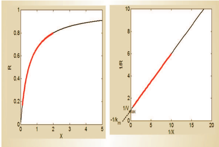
Figure 17: The figure shows inversion of the Michaelis-Menten relation.
