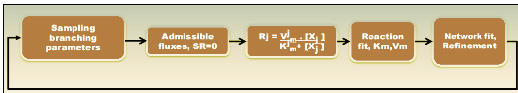
Figure 18: Flowchart illustrating the hybrid optimisation method used for modeling. Branching parameters are discretized and sampled to calculate admissible fluxes. For each individual reaction, Michaelis-Menten formula is inverted to obtain the parameters K_m, V_{max} . A final optimisation step leads to refined parameters for the full network.
