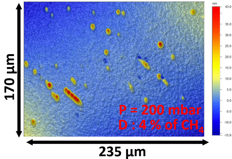
Figure 3.13: Typical surface morphology obtained using a deposition temperature about 900^{\circ}\text{C} , a 200 mbar (150 Torr) pressure, 4% of \text{CH}_4 in gaseous mixture.
