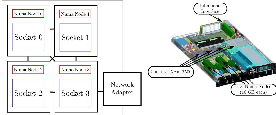
(a) Intra-node topology for the Tera 100 supercomputer. (b) Actual Node layout for a Bullx S6010 node in 1.5U (3D rendering is from S6010 support page [Bul10]).
