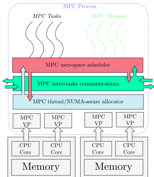
Figure 1.1: Overview of the MPC runtime.
