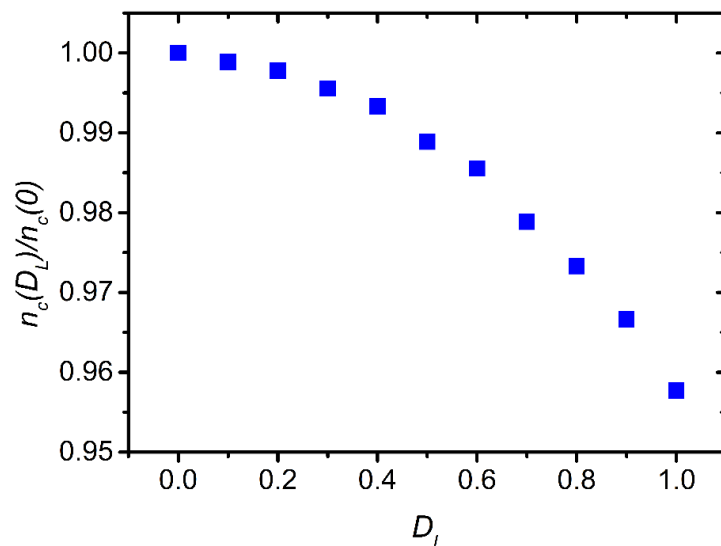
Figure 3.15 Density of a system with a given of value of D_L divided by the density of the ideal nanowire system. The largest length distribution results in a downward shift of n_c by 4.3\% \pm 0.1\% . Error bars are smaller than the data points.
