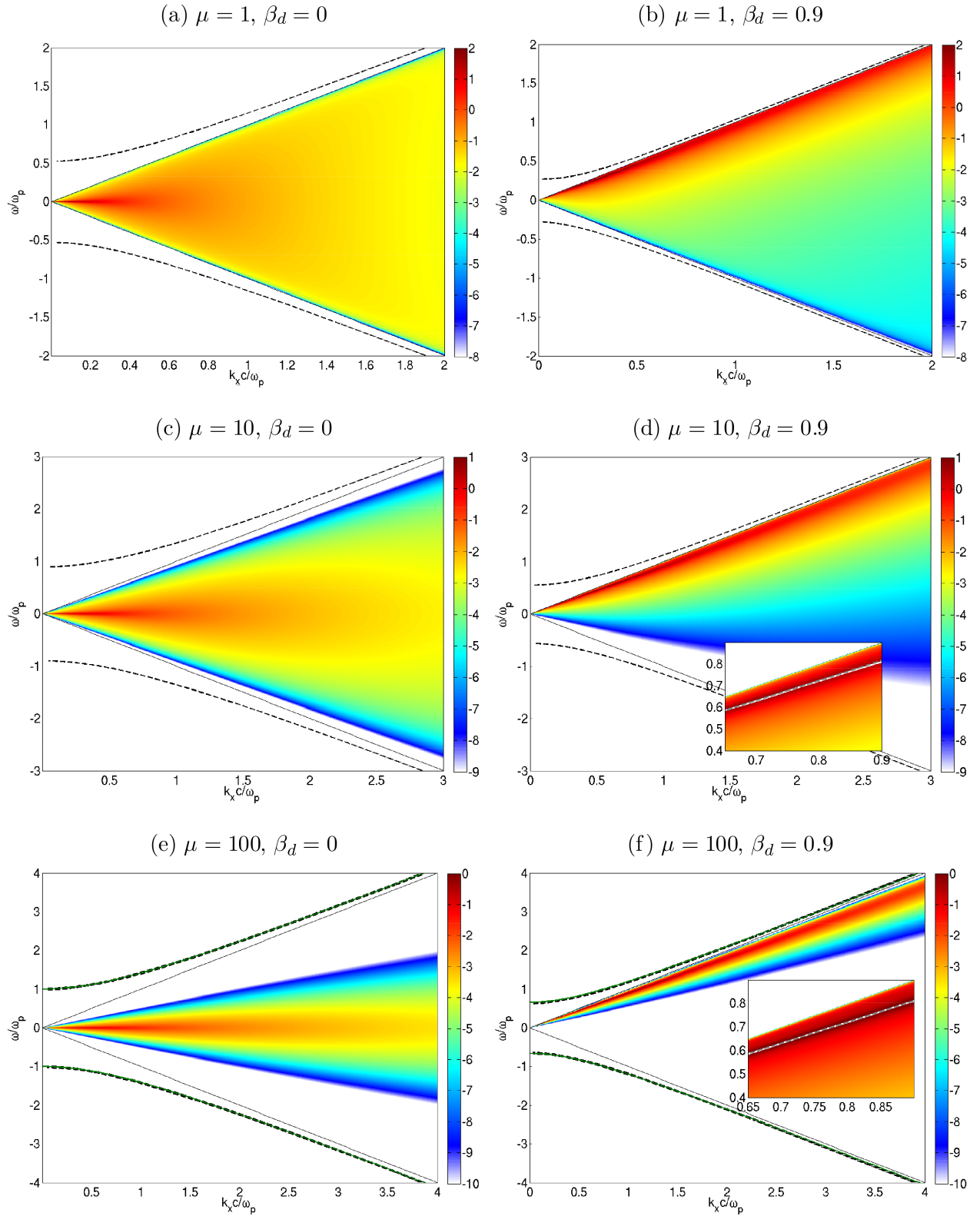
Figure 2.7. Power spectrum \langle B_y B_y^* \rangle_{k_x, \omega} (normalized to m_e^2 c^2 / e^2 ) in \log_{10} scale for an electron/pair plasma and various \mu and \beta_d values. The two black solid lines correspond to \beta_\phi = \pm 1 . The dashed curves plot the exact eigenmodes computed from Eq. (2.38). In the low-temperature case ( \mu = 100 ), the solid line plots the nonrelativistic transverse mode in panel (e) and its Lorentz transformation in panel (f). The subpanels in (d) and (f) show the exact eigenmode (grey dashed) and the approximate beam mode \omega = k\beta_d (white).
