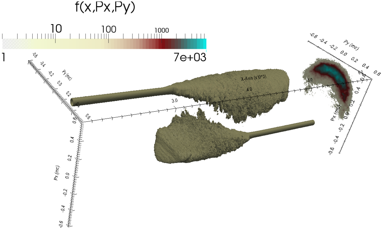
Figure 4.3. Ion phase space x\omega_{pe}/c , p_x/m_i c , p_y/m_i c isosurface (grey) before shock formation for two symmetric counter-propagating ions-electron plasma beams for v_e = v_i = \pm 0.4c , m_i = 100m_e . The colormap corresponds to the ion distribution in logarithmic scale of the beam v_i = +0.4c at the center ( x\omega_{pe}/c = 4200 ).
