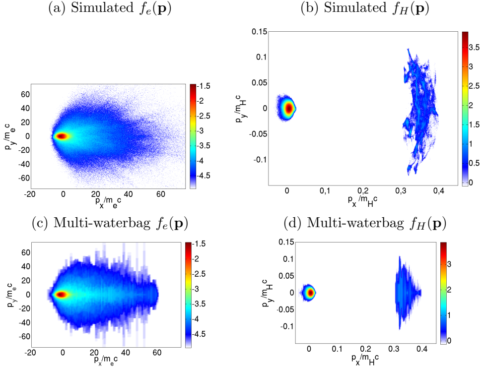
Figure 5.6. p_x - p_y phase space (in log 10 scale) of the electrons (a) and protons (b) at \omega_0 x/c = 240 and \omega_0 t = 120 . Panels (c,d) show the corresponding multi-waterbag fits used for the stability analysis (see text).
