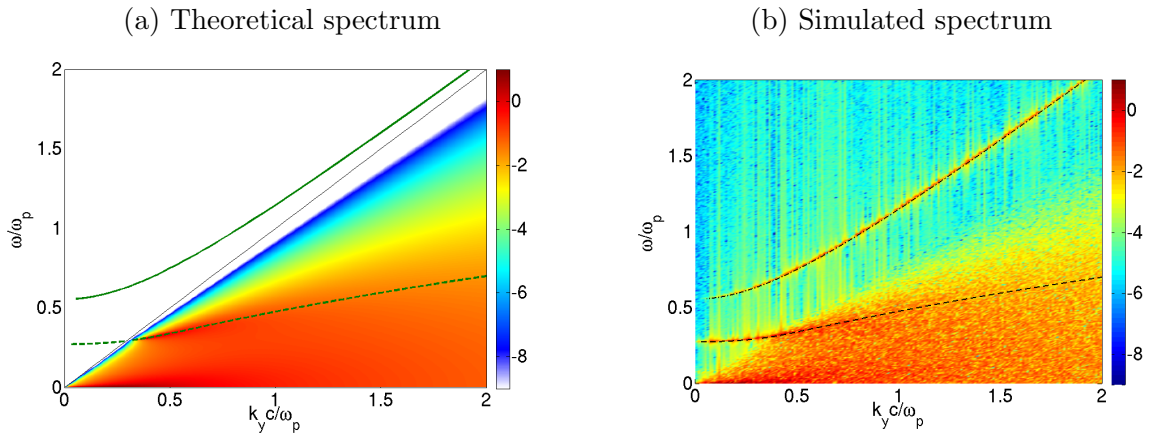
Figure 2.1. (a) Theoretical and (b) simulated (k_y, \omega) thermal magnetic fluctuation spectrum in \log_{10} scale for a Maxwell-Jüttner- distributed electron beam ( T = 51.1\text{keV} and \beta_d = 0.9 ) with \mathbf{k} \perp \beta_d .
