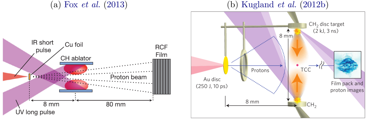
Figure 4.5. Schematic representation of the experimental setup of Fox et al. (2013) (a) and Kugland et al. (2012b) (b). The two plastic foils are separated by 2L = 4.5\text{mm} in (a).
