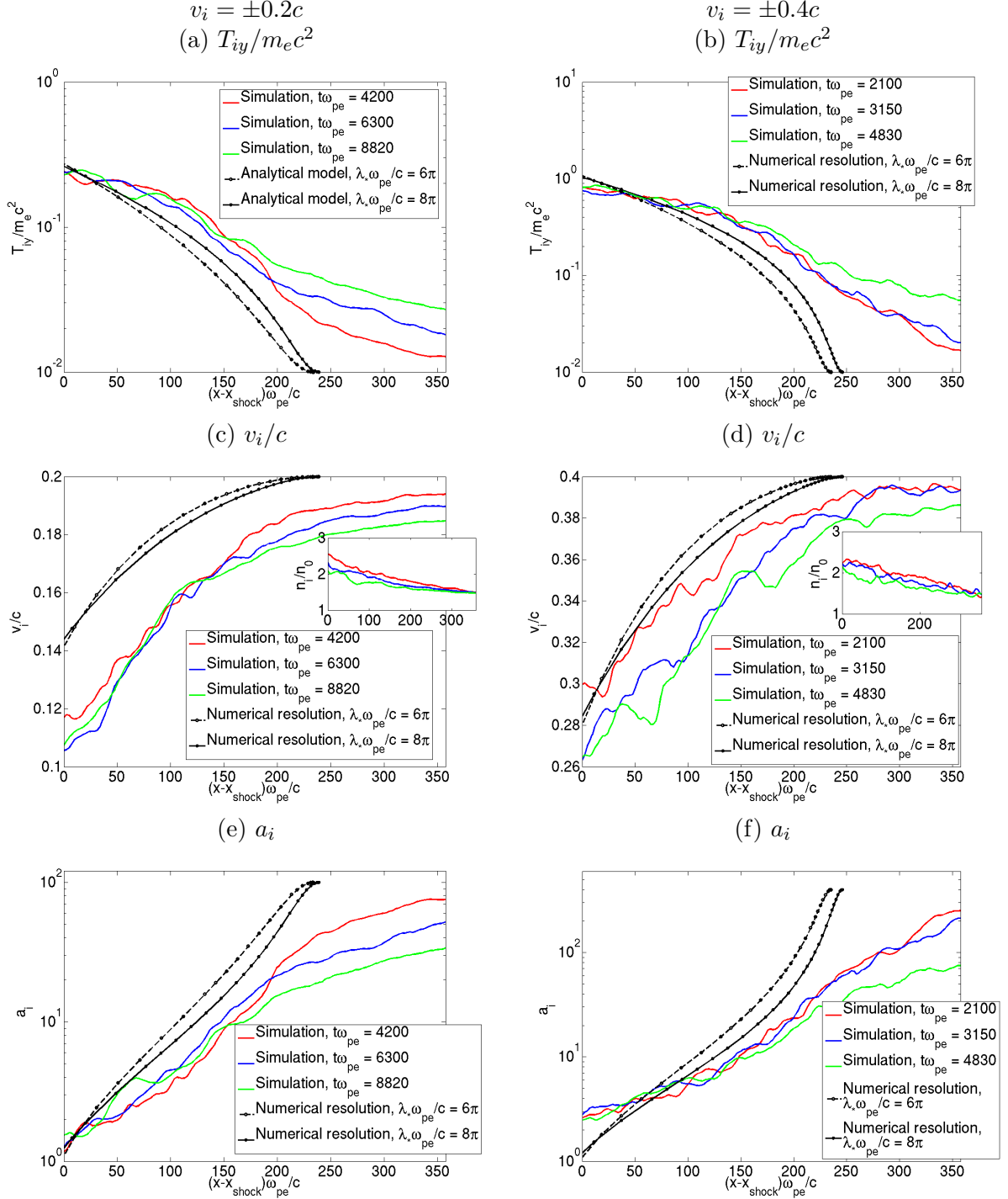
Figure 4.15. Spatial profiles of the ion plasma parameters at different times for two 2D simulations of shock-propagation: m_i = 25m_e , v_i = \pm 0.2c (a,c,e) and m_i = 25m_e , v_i = \pm 0.4c (b,d,f). The position (abscissa) is measured in respect to the position of the shock front. The shock formation time of Eq. (4.31) is t_{\text{form}}\omega_{pe} = 1800 for (a,c) and t_{\text{form}}\omega_{pe} = 800 for the case (b,d). (a,b) Transverse ion temperature profiles. (c,d) Mean longitudinal velocity and ion density (inset). (e,f) Ion anisotropy ratio. The theoretical predictions from Eqs. (4.41)-(4.45), (4.46) (numerical resolution) using \lambda_* = 8\pi c/\omega_{pe} and \lambda_* = 6\pi c/\omega_{pe} are superposed in (a-f).
