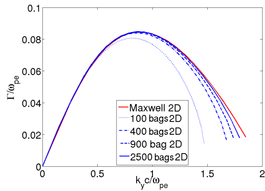
Figure 1.1. Weibel-filamentation growth rate in two counter-propagating Maxwellian electron plasma ( \beta_d = \pm 0.2 , T = m_e c^2/100 with fixed ions, red solid line) and comparison to a multi-waterbag calculation (blue lines).
