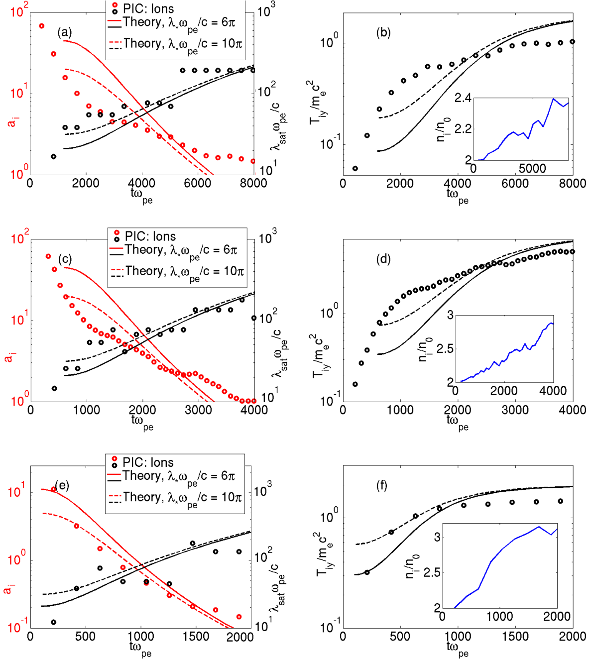
Figure 4.4. Evolution of a_{ni} [red, left axis of (a,c,e)], \lambda_{\text{sat}} \omega_{pe} / c [black, right axis of (a,c,e)], T_{iy} / m_e c^2 (b,d,f) and n_i / n_0 [inset of (b,d,f)] as a function of time normalized to \omega_{pe}^{-1} . The circles correspond to the 2D PIC simulation values. Equations (3.79), (3.82) and (3.84) are plotted respectively in plain and dashed lines for \lambda_* \omega_{pe} / c = 6\pi and \lambda_* \omega_{pe} / c = 10\pi respectively with (a,b) v_i = \pm 0.2c , m_i = 100m_e , t_* \omega_{pe} = 1200 , (c,d) v_i = \pm 0.4c , m_i = 100m_e , t_* \omega_{pe} = 600 and (e,f) v_i = \pm 0.4c , m_i = 25m_e , t_* \omega_{pe} = 100 . The values of t_* are extracted from the simulations.
