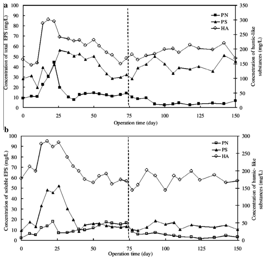
Fig. 7. Variation of concentration of total EPS (a) and soluble EPS (b) in versus of operations time (day).
