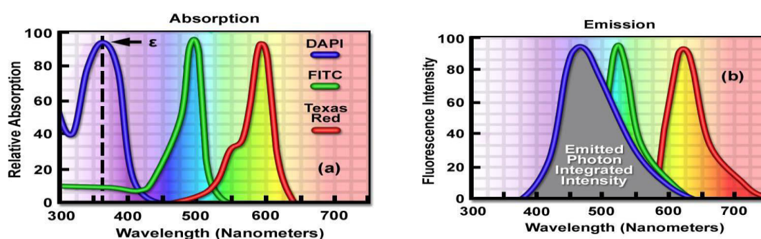
Figure 18: Fluorescent spectral profiles, plotted as normalized absorption or emission as a function of wavelength, for popular synthetic fluorophores emitting in the blue, green, and red regions of the visible spectrum. Each profile is identified with a colored bullet in (a), which illustrates excitation spectra. (b) The emission spectra for the fluorophores according to the legend in (a).
