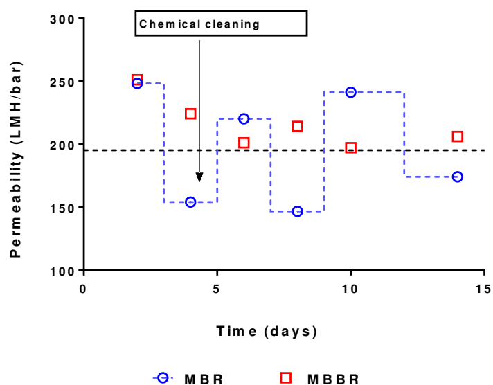
Figure 2 Example on changes of overall permeability during the experiment in MBR and MBBR.
