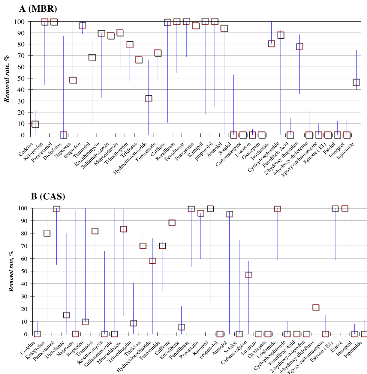
Fig. 2. Removal efficiencies (%) for 35 PPCPs in MBR (A) and CAS (B) reactors. Minimum and maximum removal efficiencies according to (Sipma et al., 2009).
