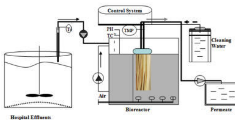
Fig. 1. Schematic diagrams of CAS (A) and MBR (B) systems treatment.
