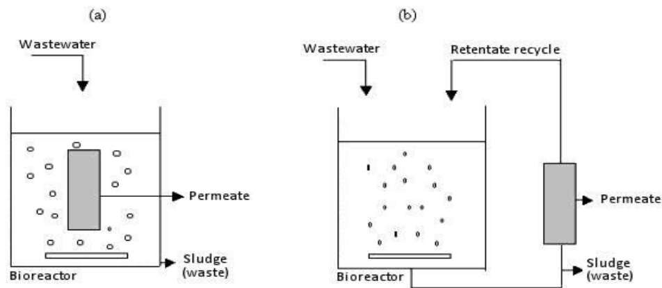
Figure 5: Typical membrane bioreactor system (Pombo et al. , 2011)
