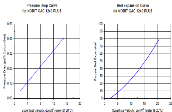
Fig. 2 Represented the pressure Drop Curve and the bed expansion curve for GAC1240 plus
