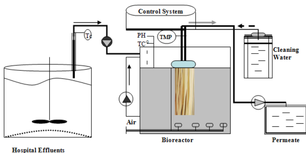
Figure 3: schematic diagram of the membrane bioreactor
