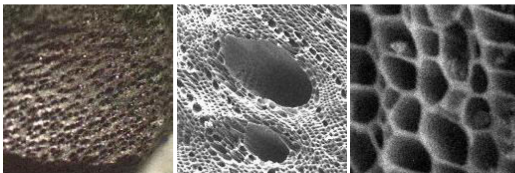
Figure 12: Activated carbon: surface and pores – scanning electron microscope image. Magnification increases from left to right. (Courtesy of Roplex Engineering Ltd.).
