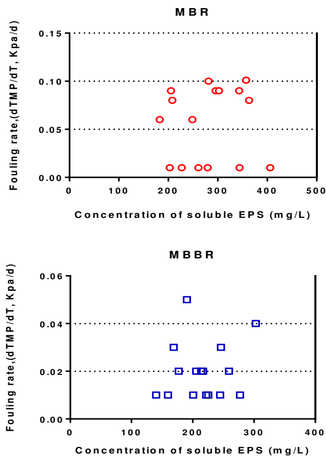
Figure 3 correlations between soluble EPS and calculated fouling rate in both MBR and MBBR reactors.
