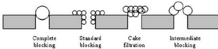
Figure 9. Fouling mechanisms in a membrane filtration (Radjenovic et al. , 2008)
