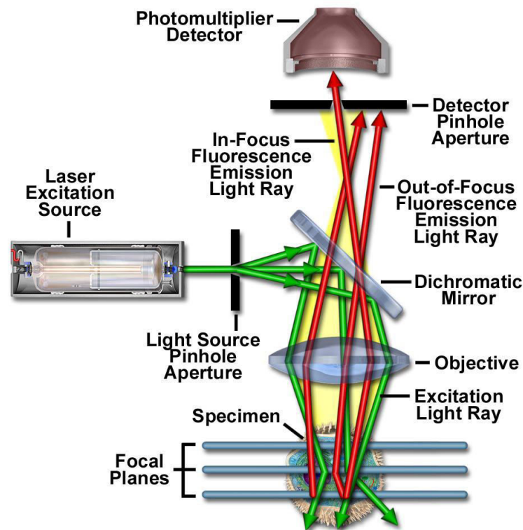
Figure 17: Schematic diagram of the optical pathway and principal components in a laser scanning confocal microscope.
