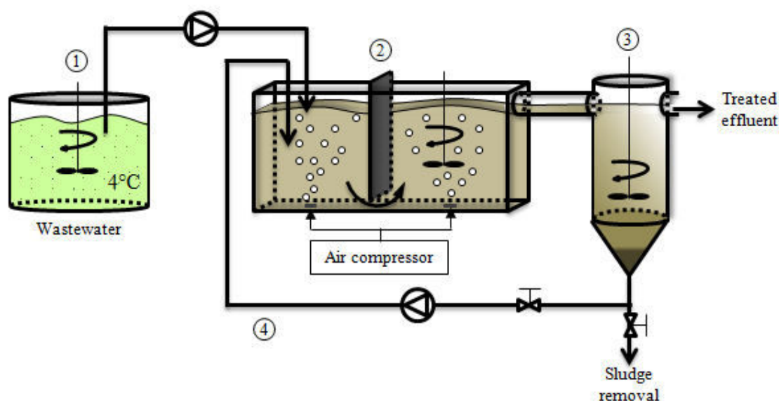
Figure 2: Description of the conventional activated sludge process used. Wastewaters were kept in a refrigerated (4°C) and agitated tank (1) where it was directly pumped to feed the pilots. Influent flow rate was 21.6 \text{ L.d}^{-1} , and corresponded to a hydraulic residence time of 15.3 \text{ h}^{-1} in the aeration tank (2) where aeration ( 2 and 4 \text{ mg.L}^{-1} ) was operated by repeated aerobic/anoxic cycles (2h/2h) in order to ensure nitrification and denitrification. Sludge recirculation (4) from the clarifier (3) was maintained at 100% feed flow rate. Solids residence time ( i.e. sludge age) was maintained at 15 days throughout the experiments: settled sludge was wasted every two days accordingly considering sludge losses through the effluent.
