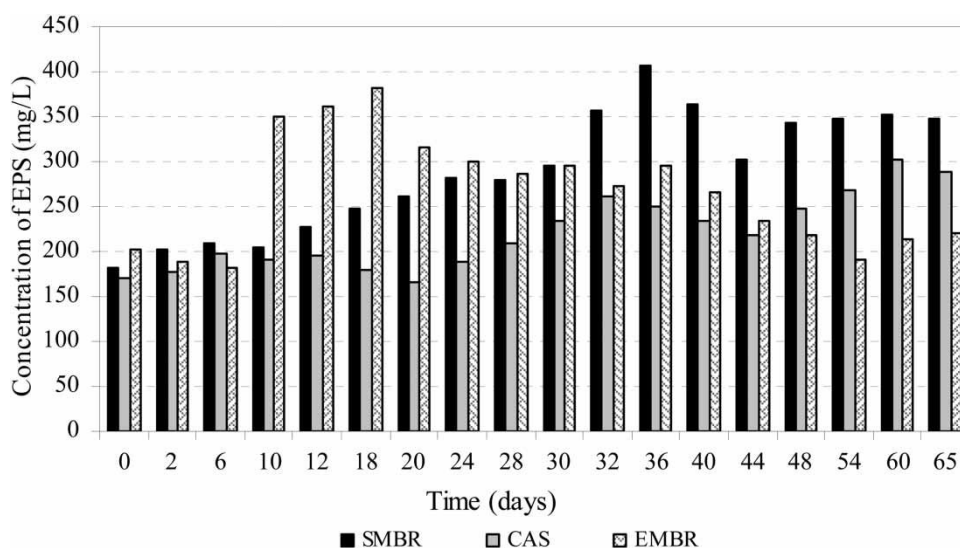
Figure 1 | EPS concentration in the mixed liquor for SMBR, EMBR and CAS systems.
