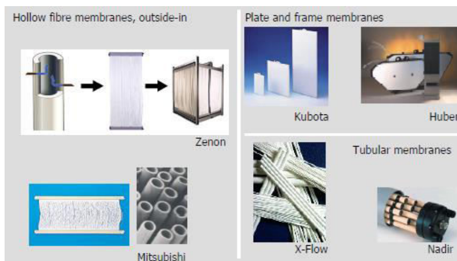
Figure7. Examples of commercially available membranes, applied in cross flow filtration (EVENBLIJ, 2006)
