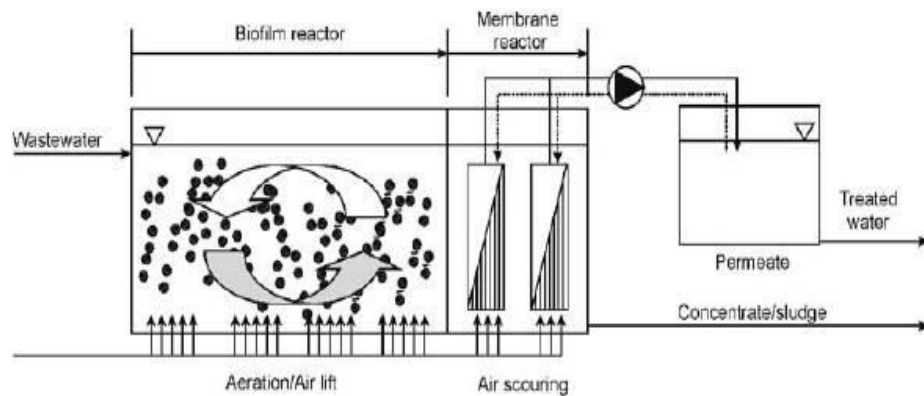
Figure 11: Typical schematics of a attached membrane bioreactor (Lee et al. , 2001; Leiknes and Ødegaard, 2007)
