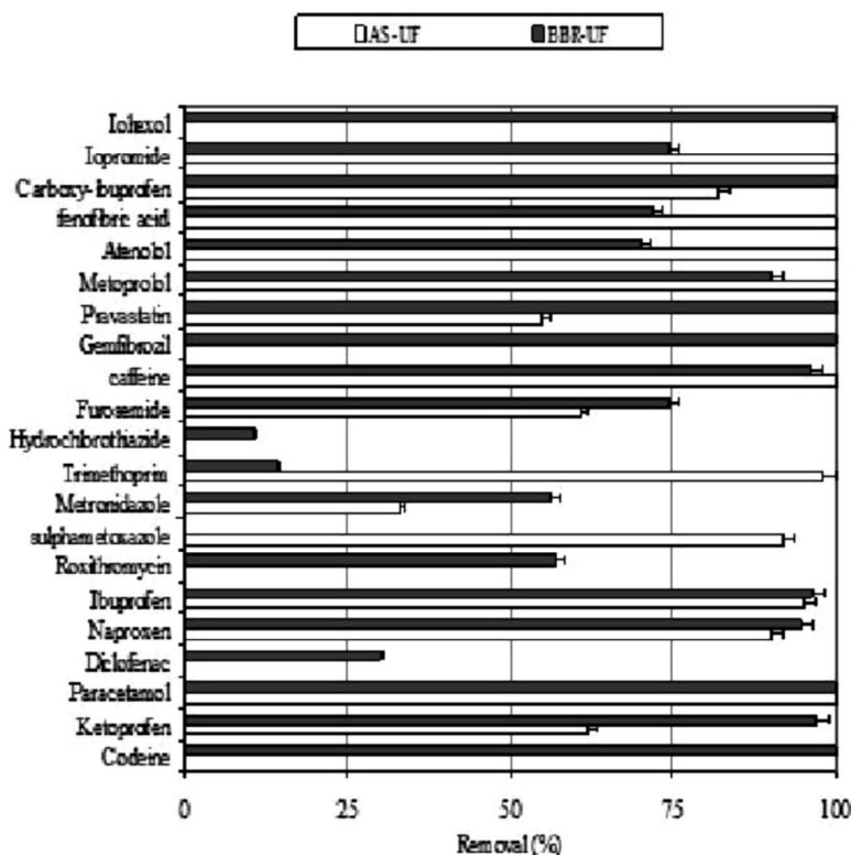
Fig. 3. Concentrations and removal rates of PPCPs in both AS-UF and BBR-UF systems.
