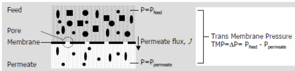
Figure 6: Schematic shapes for membrane filtration process
