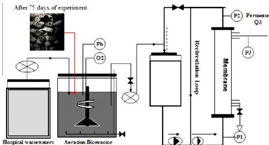
Fig. 1. Activated sludge followed by ultrafiltration system (AS-UF).
