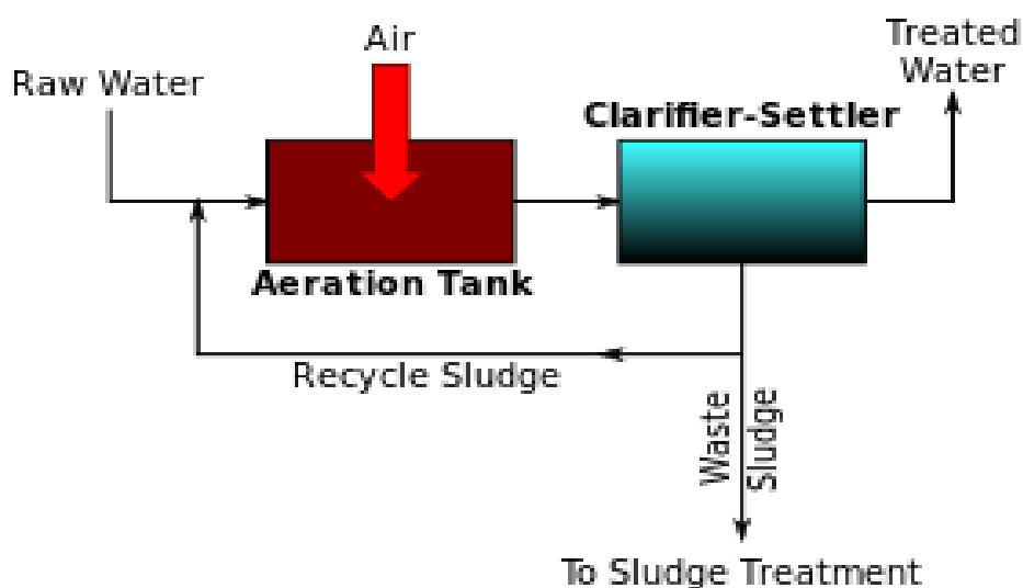
Figure 4: Schematic overview of a typical conventional activated sludge process
