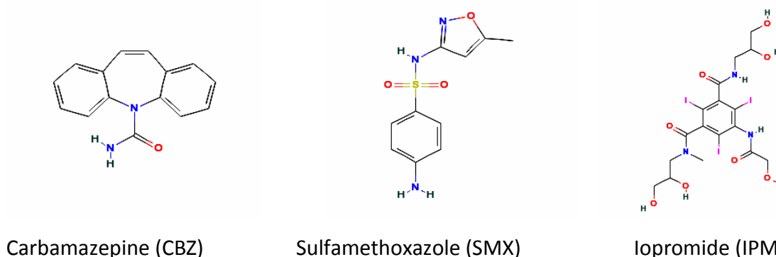
Figure1: Chemical Structure of selected PPCPs ( http://pubchem.ncbi.nlm.nih.gov ).
