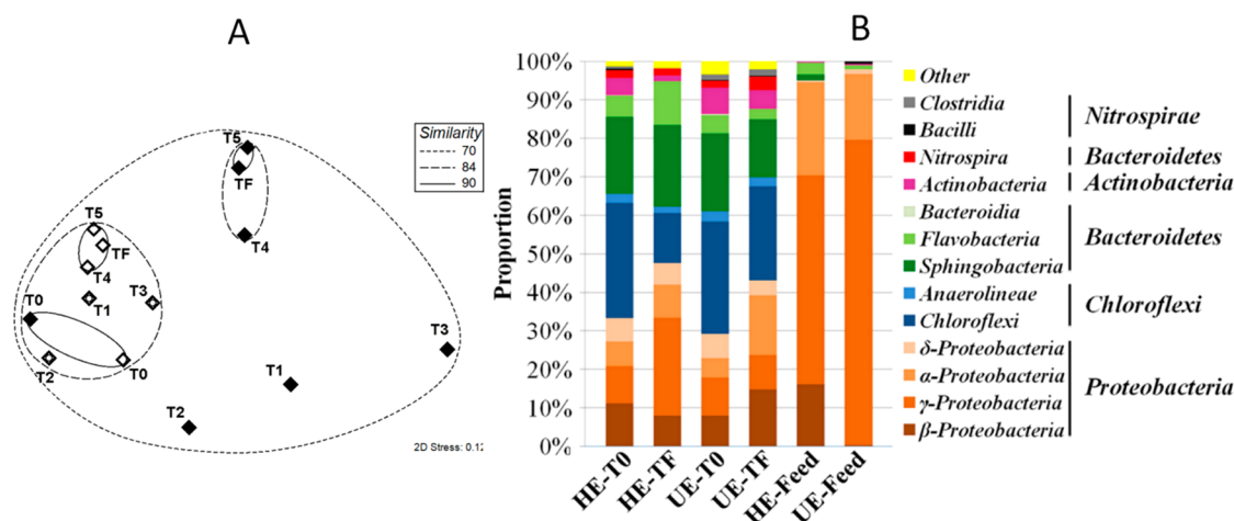
Figure 3. (A) 2D-nMDS map based on the semiquantitative analysis of the DGGE profiles showing the evolution of the activated sludge bacterial community in both reactors (◇ UE, ◆ HE). This 2D projection of the BC similarity matrix allowed visualization of the similarity between each bacterial community over time, i.e. the distance between diamonds. Plain and dashed lines represent the differing percentage of similarities. (B) Proportion of bacteria classes and phyla recovered from the HE and UE feed to the reactors (HE-Feed and UE-Feed) and from the HE and UE reactor sludges at the beginning (HE-T0 and UE-T0) and the end (HE-TF and UE-TF) of the experiment.
