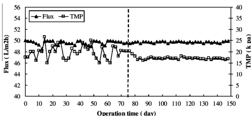
Fig. 5. Transmembrane pressures and permeate flux of BBR-UF and classical MBR as a function of operation time.
