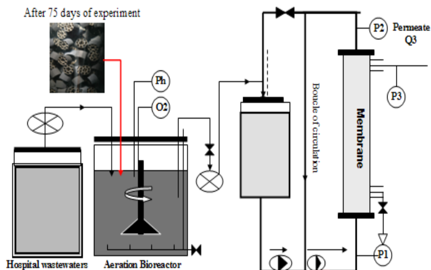
Figure 4: schematic of Activated sludge followed by ultrafiltration system (AS-UF).
