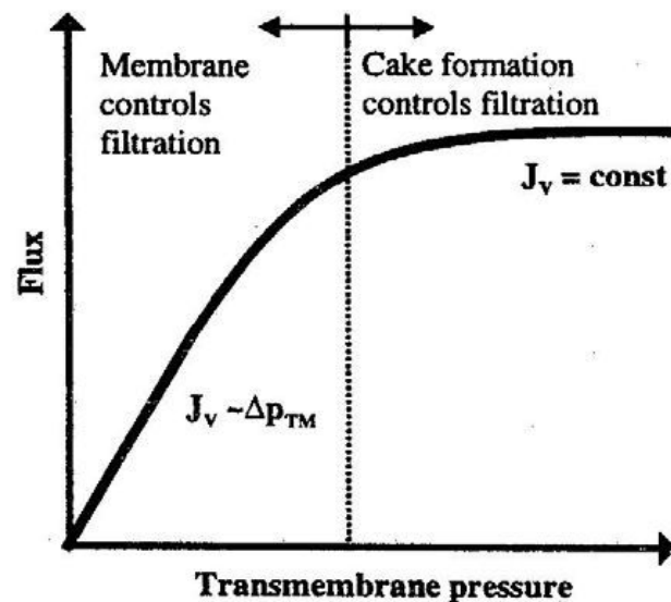
Figure 8: Relationship between transmembrane pressure and flux (Günder, 2001)
