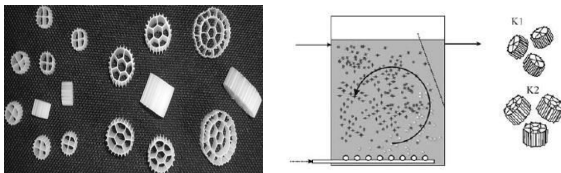
Figure 10: Photo of (from left to right) Kaldnes type K1, K2 and K3 biofilm carriers and schematic of the moving-bed-biofilm reactor (MBBR). (Rusten et al. , 1994; Leiknes and Ødegaard, 2007)
