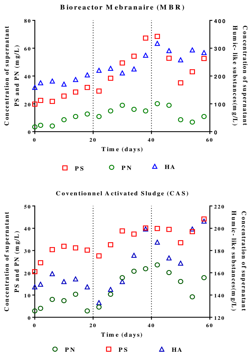
Fig. 7. EPS concentration variation in supernatant (MBR and CAS).
