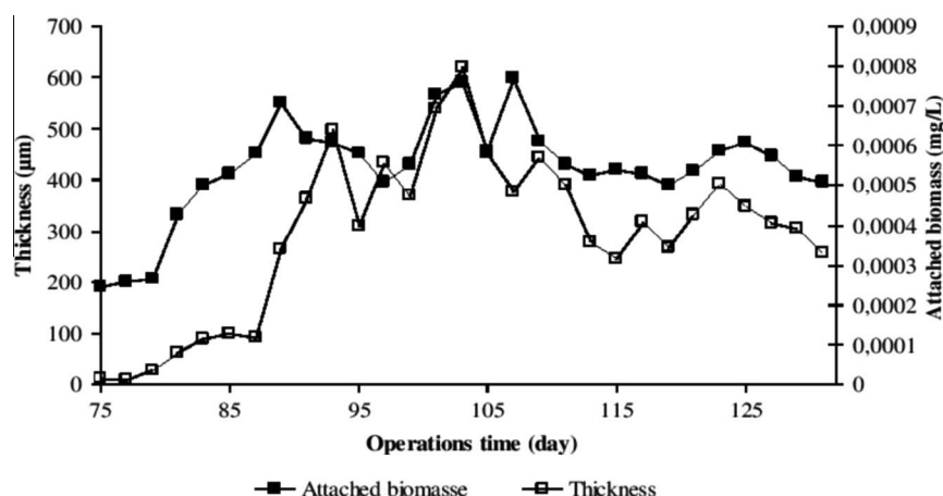
Fig. 6. Evolution of the thickness and attached biomasses on supports media versus time.
