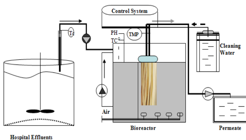
Figure 1 Schematic diagram of membrane bioreactor
