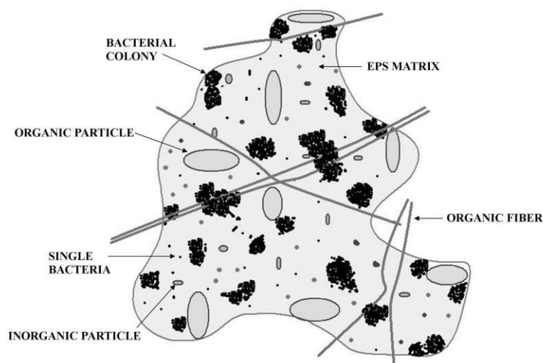
Figure 13: Schematic example of the structure of an activated sludge floc including single bacteria, bacterial colonies, absorbed organic and inorganic particles and organic fibres surrounded by the EPS matrix, Adapted from (Mikkelsen, 1999).
