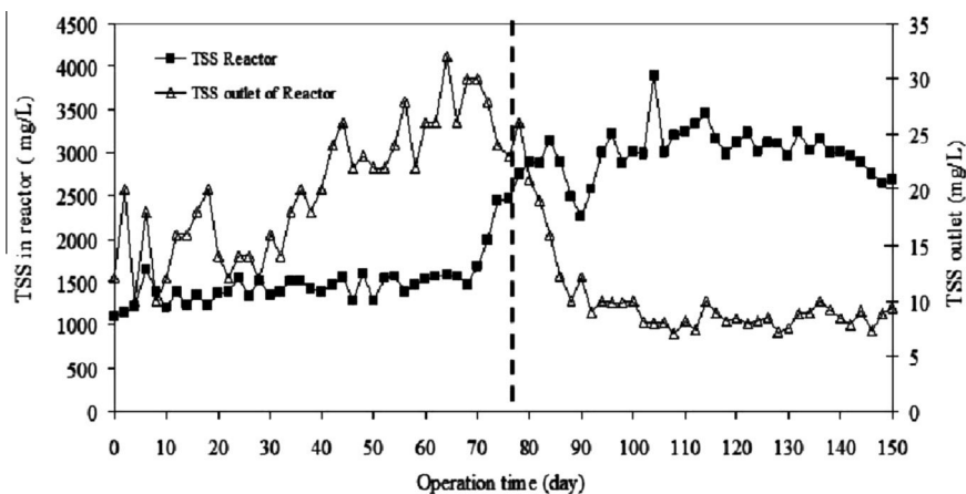
Fig. 4. TSS (mg/L) in the bioreactor and in the outlet before and after introduction the biofilm supports media.
