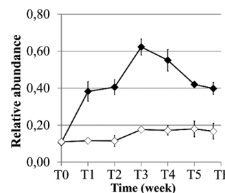
Figure 5. Evolution of the relative abundance of class 1 RIs over time in the HE (◆) and UE (◇) reactors.
