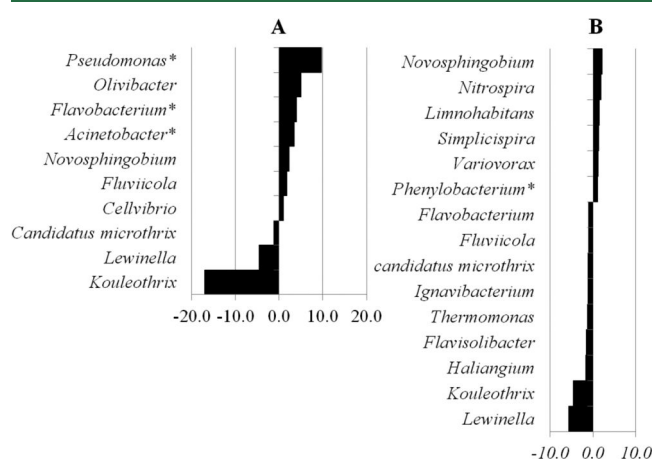
Figure 4. Major positive or negative variations (in excess of 1%) of the proportion of bacterial genus in (A) the HE reactor and (B) the UE reactor between the beginning and the end of the experiment. * corresponds to genus found also in the effluents used for the feed of the reactors.
