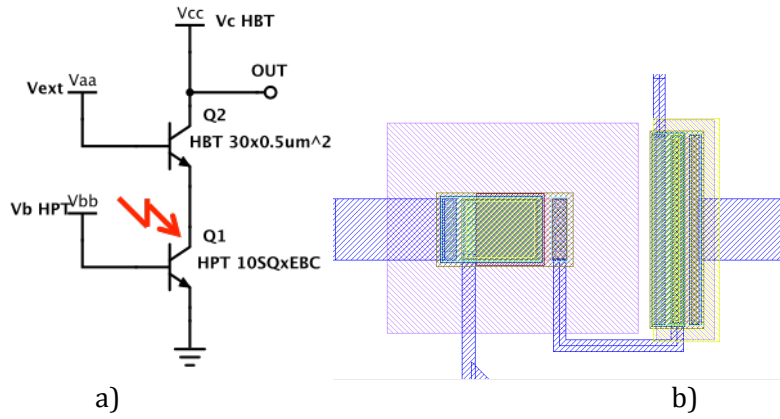
Figure 4.32 Common emitter HPT and Common base HBT topology a) schematic representation b) layout view
