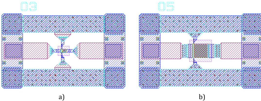
Figure 2.25 Illustration of the layout of two SiGe HPT structures: a) 10x10 \mu m 2 xBCrT ;b) 50x 50 \mu m 2 xBCrT. Figure 2.26 shows chip microphotograph of the fabricated (R1-10SQxBCrT) and (R1-50SQxBCrT) HPTs.
