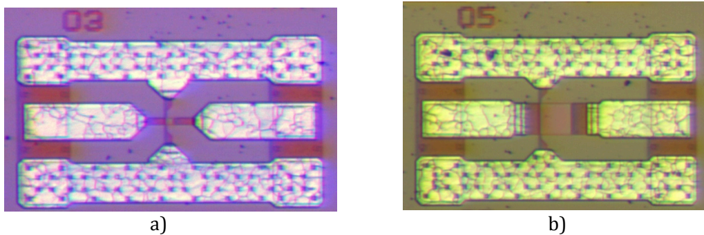
Figure 2.26 Photograph of two fabricated cells of low noise RF GSG pads and a) 10x10 \mu m 2 HPT R1-10SQxBCrT and b) 50x50 \mu m 2 HPT R1-50xBCrT
