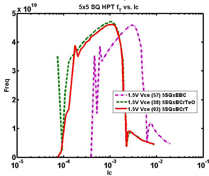
Figure 2.45 Measured f_T vs. I_c of R1-05SQxBCrT, R1-05SQxBCrTeO, R1-05SQxEBC
