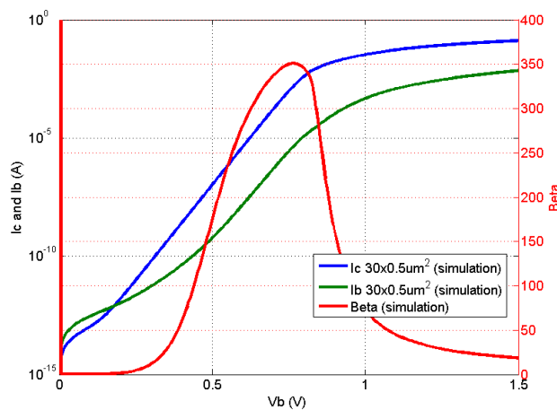
Figure 4.31 Gummel characteristics of a 30 \times 0.5 \mu m^2 HBT.
