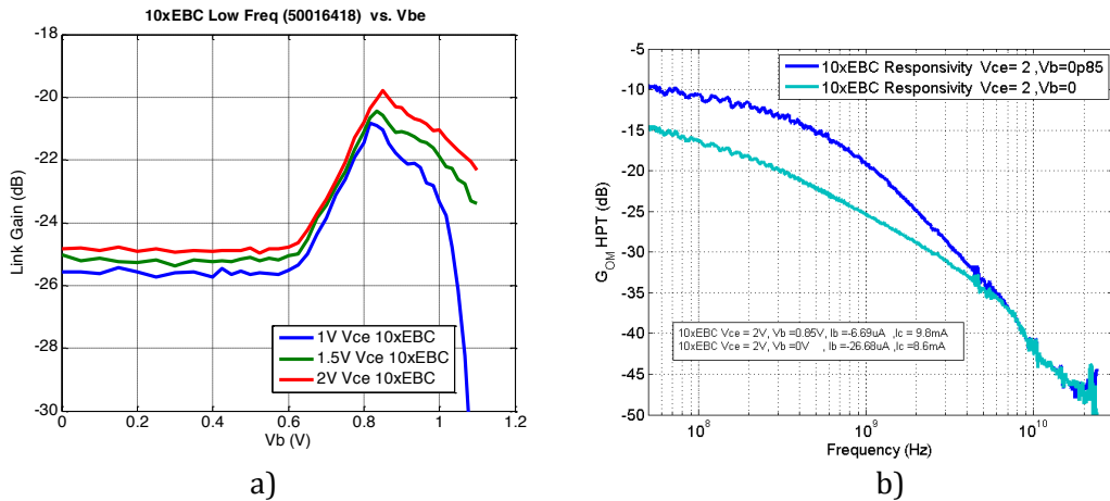
Figure 4.30 Opto-microwave gain of the VI system VSCEL link with a) a single HPT 10SQxEBC at 50MHz at different Vce values (1V, 1.5V, 2V) and b) G_{OM} link vs. Frequency at V_{ce} = 2V, V_b = 0.85V and at V_{ce} = 2V, and V_{be} = 0V
