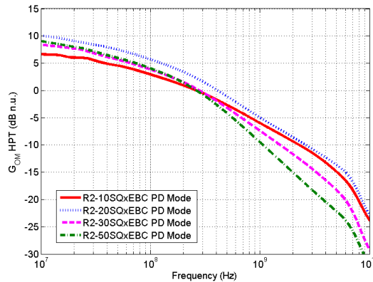
Figure 3.10 relative G_{OM} of xEBC HPTs from 10 \times 10 \mu m^2 to 50 \times 50 \mu m^2 in PD mode operation
