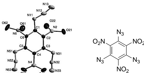
Fig. 8. ORTEP representation of 1,3,5-triazido-2,4,6-trinitrobenzene with the ellipsoids of the C, N, and O atoms drawn at the 50% probability level. 54
