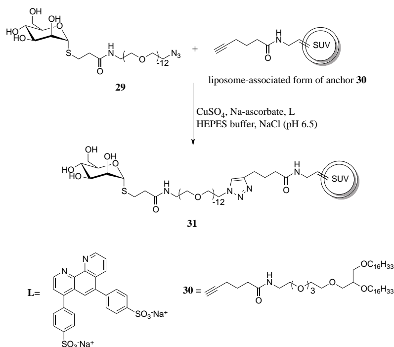
Fig. 16. Coupling of the Ligand 29 to preformed liposomes that incorporate the alkyne functionalized anchor 30 by Click Chemistry in the presence of the Cu(I) ligand bathophenanthroline disulfonate. 84c
