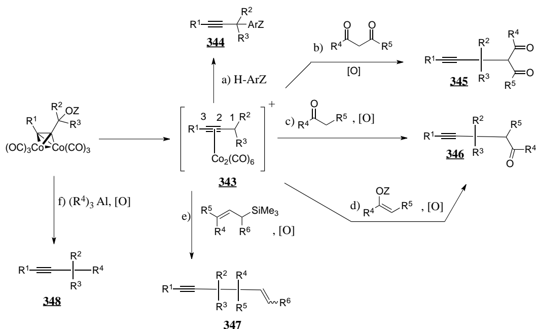
Scheme 81. Carbon-carbon bond formation with (propargyl)Co 2 (CO) 6 + complexes. 270
