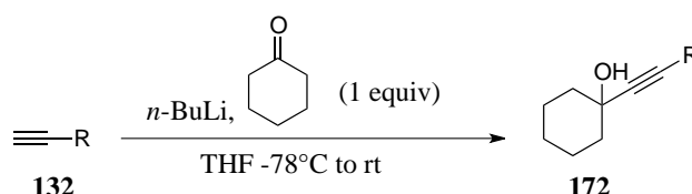
Scheme 47. Coupling between a cycloketone and a terminal alkyne by n -BuLi.
