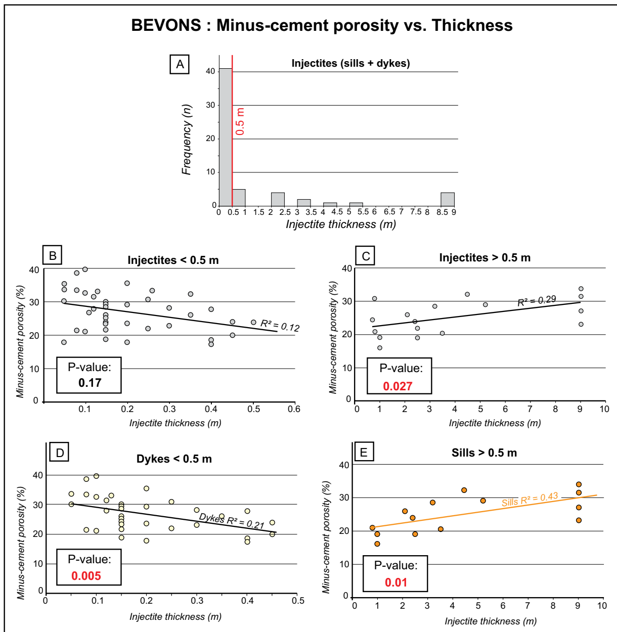
Figure 19. Minus-cement porosity vs. injectite thickness in the Bevons area. (A) Injectite thickness distribution and frequency. Minus-cement porosity is plotted against (B) injectite thickness < 0.5m; (C) injectite thickness > 0.5 m; (D) dykes thickness < 0.5 m; (E) sills thickness > 0.5 m.
