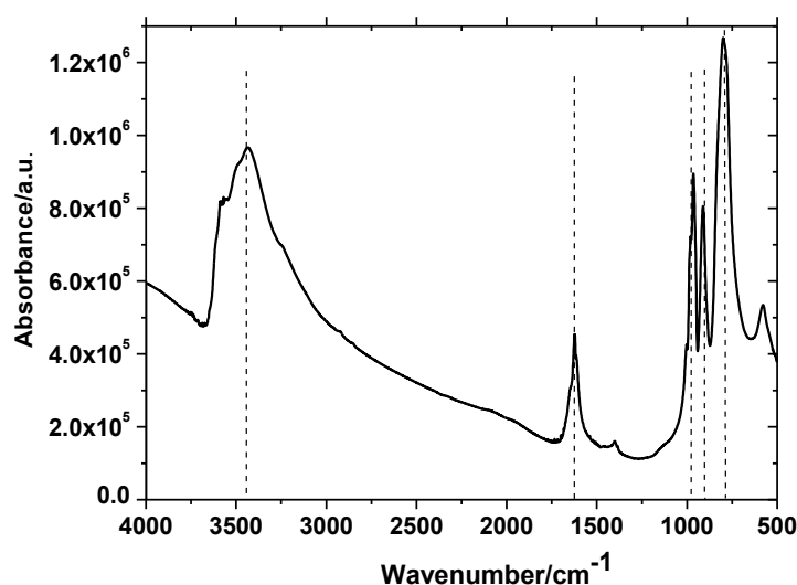
Figure 5-2 FTIR spectrum of the catalyst \text{Na}_4\text{W}_{10}\text{O}_{32} \cdot 7\text{H}_2\text{O} .
