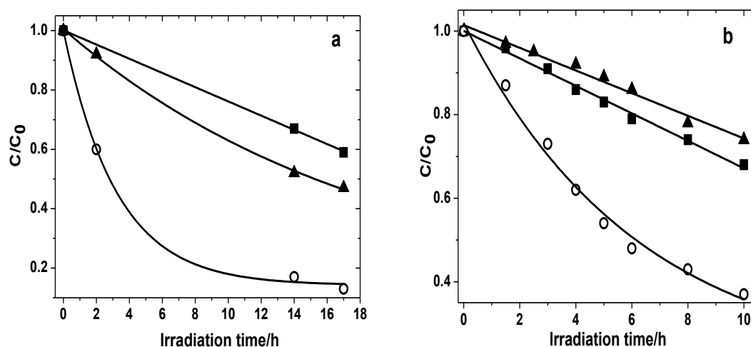
Figure 6-10 Effect of pH on NAD ( 3.0 \times 10^{-4} mol L -1 ) degradation under irradiation at 365 nm in the presence of the catalysts: a) 6 3-DOM-Mg 2 Al-W 10 LDH (0.6 mg 10 mL -1 ; ○ pH 3.3; ▲ pH 5.6; ■ pH solution 6.6. b) SC-Mg 2 Al-W 10 LDH (0.025 mL 10 mL -1 ; ○ pH 3.6; ▲ pH 5.6; ■ pH solution 7.5).
