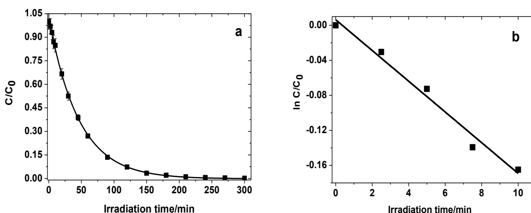
Figure 2B-5 a) Influence of \text{NaN}_3 ( 2.0 \times 10^{-3} \text{ mol L}^{-1} ) on the degradation kinetic of aerated aqueous NAD solution ( 3.0 \times 10^{-4} \text{ mol L}^{-1} ) as function of irradiation time ( \lambda_{\text{irrad}} = 254 \text{ nm} ). b) First order behavior corresponding to the linear part of the kinetic given in a) ( R^2 = 0.974 ).
