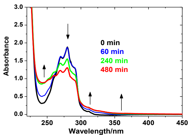
Figure 2B-2 Evolution of the UV-vis absorption spectra of aerated aqueous NAD solution ( 3.0 \times 10^{-4} \text{ mol L}^{-1} ) under Suntest excitation as function of irradiation time.
