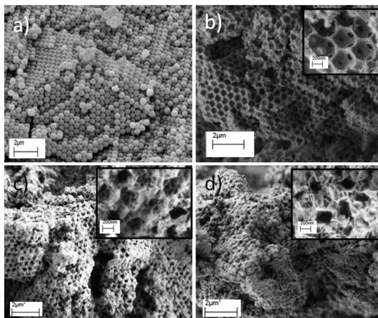
Figure 6-5 SEM images of: a) colloidal crystal after successive impregnations. b) 3-DOM oxides obtained after calcination at 400 °C. c) 3-DOM-Mg 2 Al-DDS and d) 3-DOM-Mg 2 Al-W 10 .
