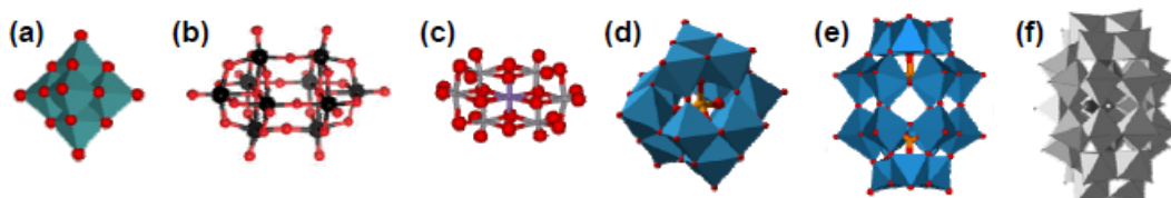
Figure 4-4 Examples of POMs structures. Isopolyoxianions (a, b) and heteropolyoxyanions (c, d, e, f). a) Lindqvist [M_6O_{19}]^n , b) [M_{10}O_{32}]^n (such as decatungstate anion W_{10}O_{32}^{4-} ), c) Anderson-Evan [XM_6O_{24}]^n , d) Keggin [XM_{12}O_{40}]^n , e) Wells-Dawson [X_2M_{18}O_{62}]^n , f) Preyssler [XP_5W_{30}O_{110}]^n .
