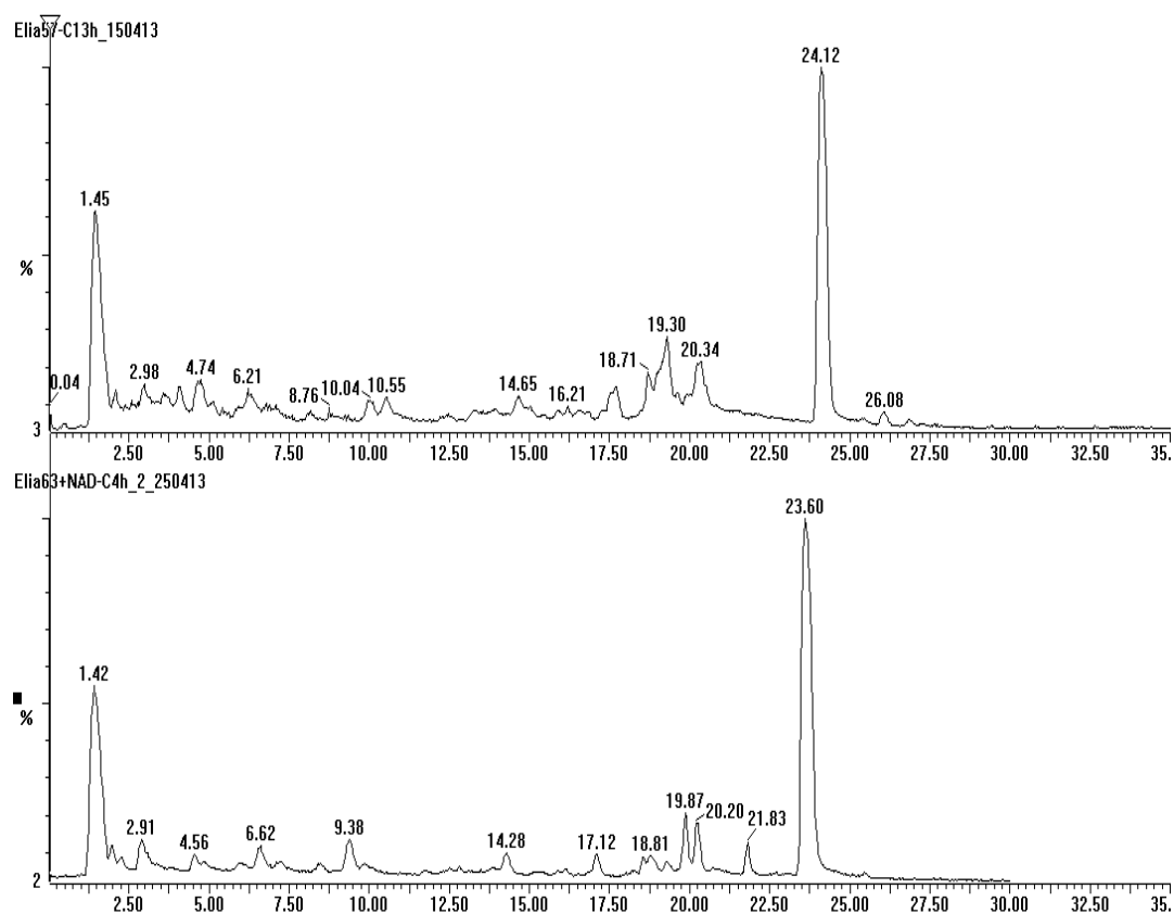
Figure 6-14 TIC chromatogram ( \text{ES}^+ ) of NAD aerated aqueous solution ( 3.0 \times 10^{-4} \text{ mol L}^{-1} ) irradiated at 365 nm in the presence of: 3-DOM- \text{Mg}_2\text{Al-W}_{10}\text{O}_{32}^{4-} LDH (top figure) and SC- \text{Mg}_2\text{Al-W}_{10} LDH (bottom figure).
