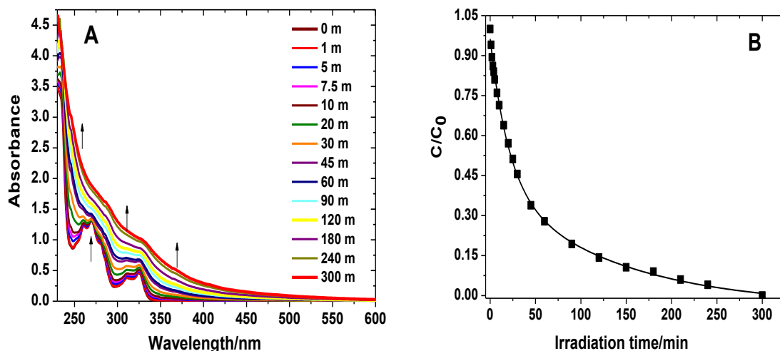
Figure 3B-3 a) Evolution of the UV-vis spectra of aerated aqueous 2-NOA solution ( 3.0 \times 10^{-4} mol L ^{-1} ). b) Respective kinetics of degradation as function of irradiation time followed by HPLC-DAD ( \lambda_{\text{det}} = 270 nm) upon irradiation at 254 nm with 1 lamp.
