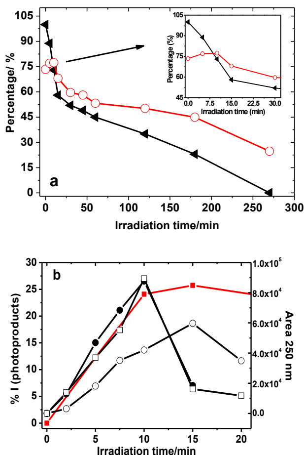
Figure 2B-9 a) Evolution of the % I of the luminescence of an aerated aqueous NAD solution ( 3.0 \times 10^{-4} mol L -1 ) upon excitation at 254 nm (○), compared to the % of NAD degradation in the same conditions (◄). b) % I (photoproducts) for the initial 20 minutes of irradiation (■) and evolution of the formation of some di-hydroxylated photoproducts (11.1 min ○; 17 min ●; 19.5 min □).
