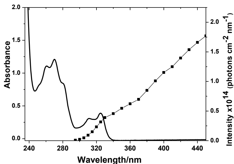
Figure 3B-1 UV absorption spectrum of 2-NOA aqueous solution ( 3.0 \times 10^{-4} \text{ mol L}^{-1} ) and emission spectrum of solar light (dotted line).
