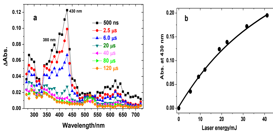
Figure 3A-8 a) Transient absorption spectra of 2-NOA de-aerated aqueous solution ( 2.0 \times 10^{-5} mol L ^{-1} ) obtained by nanosecond laser flash photolysis with excitation at 266 nm, recorded at 500 ns, 2.5, 6.0, 20, 40, 80 and 120 \mu\text{s} after pulse. b) Evolution of the absorbance band at 430 nm as function of laser energy.
