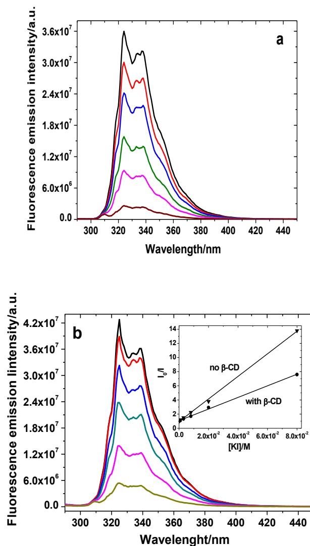
Figure 2B-13 Quenching effect of KI on fluorescence intensity ( \lambda_{\text{ex}} = 280 nm) of aqueous NAD solution ( 1.0 \times 10^{-5} mol L -1 ) in a) absence and b) presence of \beta -CD ( 1.0 \times 10^{-2} mol L -1 ). Concentrations of KI from top to bottom: 0, 8.0 \times 10^{-4} , 3.0 \times 10^{-3} , 8.0 \times 10^{-3} , 2.0 \times 10^{-2} and 8.0 \times 10^{-2} mol L -1 . Inset Figure 2B-14b are represented the Stern-Volmer plots in (►) absence and (●) presence of \beta -CD ( 1.0 \times 10^{-2} mol L -1 ).
