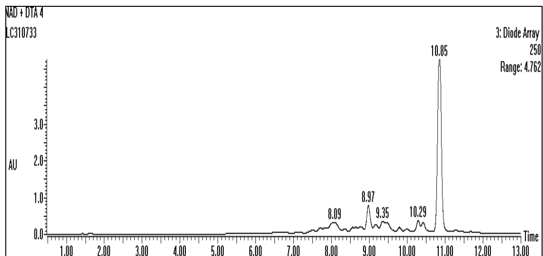
Figure 5-7 HPLC-DAD chromatogram of aerated aqueous irradiated NAD ( 3.0 \times 10^{-4} \text{ mol L}^{-1} ) solution in the presence of \text{W}_{10}\text{O}_{32}^{4-} ( 3.0 \times 10^{-4} \text{ mol L}^{-1} ) irradiated at 365 nm ( \lambda_{\text{det}} = 250 \text{ nm} ).
