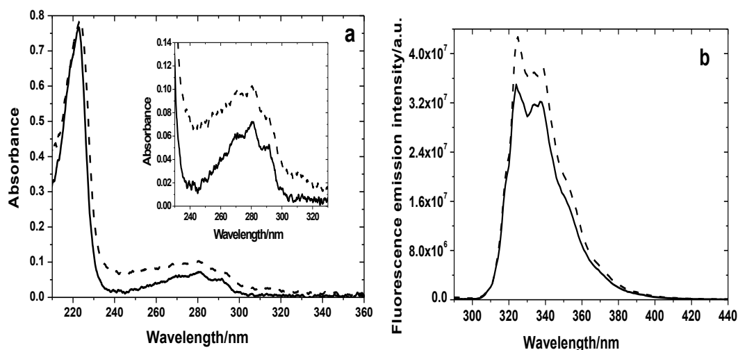
Figure 2B-10 a) UV absorption spectra of aqueous NAD solution ( 1.0 \times 10^{-5} mol L ^{-1} ) in absence (solid line) and presence of \beta -CD 1.0 \times 10^{-2} mol L ^{-1} (dotted line). Inset is given the amplified graphic of the absorption in the range 230-330 nm. b) Fluorescence emission spectra ( \lambda_{\text{ex}} = 280 nm) of the respective solutions described in a).
