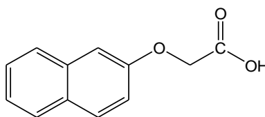
Figure 1-6 Chemical structure of 2-(naphthyloxy) acetic acid (2-NOA).
