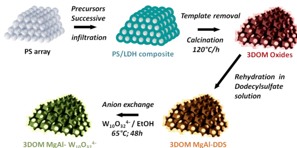
Figure 6-3 Schematic representation of the synthesis of 3-DOM- \text{Mg}_2\text{Al} - \text{W}_{10} LDH.
