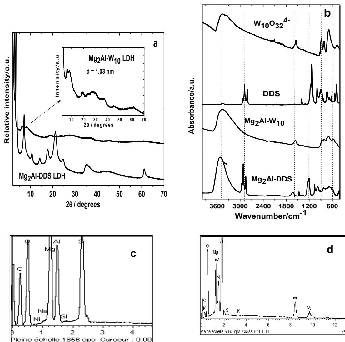
Figure 6-1 a) PXRD patterns of classical LDH \text{Mg}_2\text{Al} -DDS and \text{Mg}_2\text{Al} - \text{W}_{10} b) FTIR spectra of \text{W}_{10}\text{O}_{32}^{4-} , DDS and classical LDHs \text{Mg}_2\text{Al} -DDS and \text{Mg}_2\text{Al} - \text{W}_{10} . EDS spectrum of c) classical \text{Mg}_2\text{Al} -DDS LDH and d) classical \text{Mg}_2\text{Al} - \text{W}_{10} LDH.
