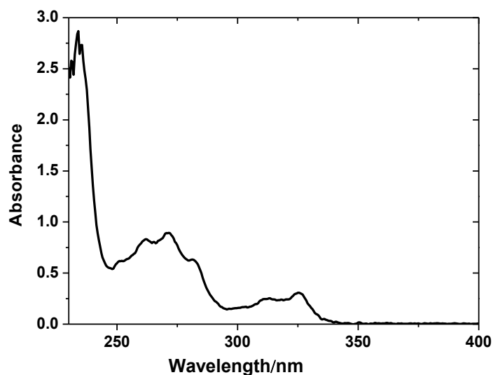
Figure 3A-1 UV absorption spectrum of 2-NOA aqueous solution ( 2.0 \times 10^{-4} mol L ^{-1} ).
