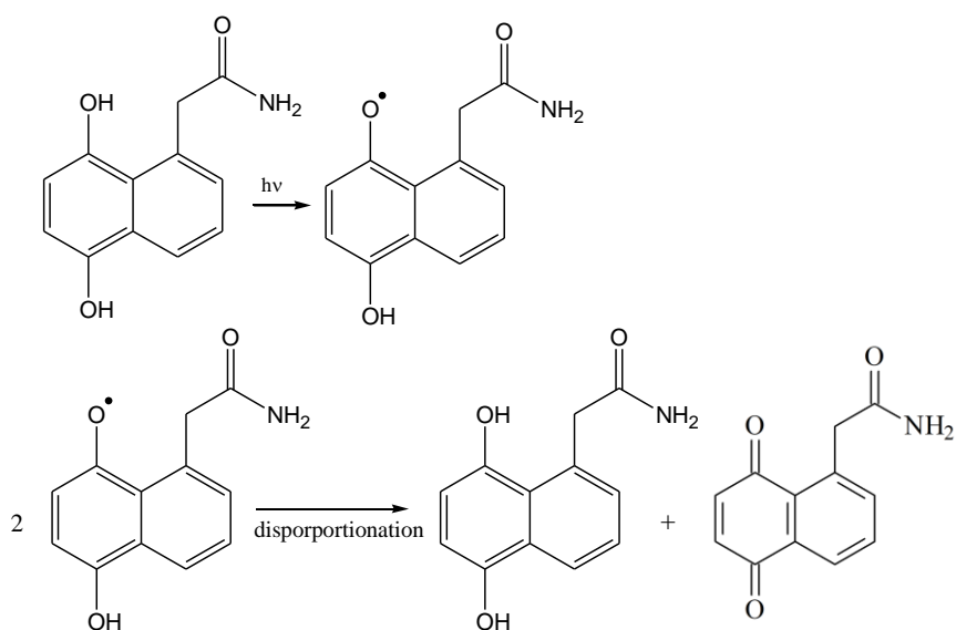
Scheme 2B-6 Possible pathways for naphthoquinone formation.
