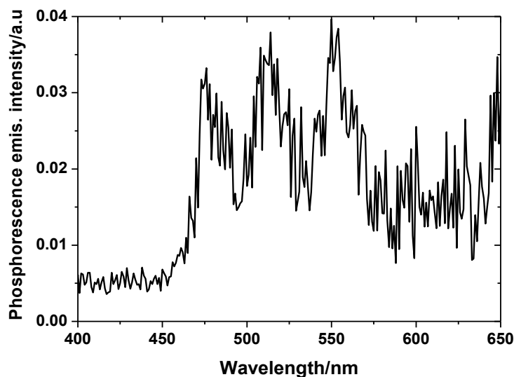
Figure 3A-6 Phosphorescence spectrum of 2-NOA in acetonitrile ( 2.0 \times 10^{-5} mol L -1 ) at 77 K.
