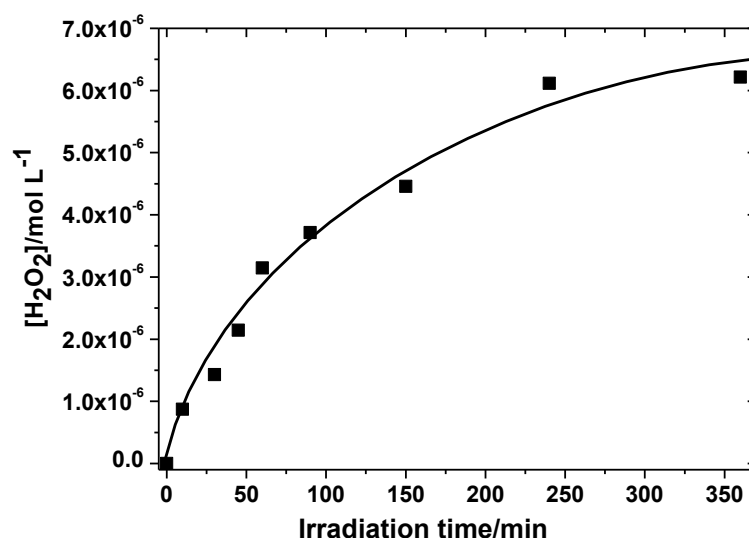
Figure 3B-5 Evolution of \text{H}_2\text{O}_2 formation of aerated aqueous 2-NOA solution ( 1.0 \times 10^{-5} \text{ mol L}^{-1} ) upon 254 nm irradiation (system with 1 germicidal lamp).
