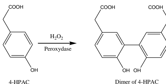
Scheme 2B-1 Reaction of \text{H}_2\text{O}_2 and 4-HPAC in the presence of enzyme peroxidase with formation of the 4-HPAC dimer detected by fluorescence at 400 nm ( \lambda_{\text{ex}} = 320 \text{ nm} ).
