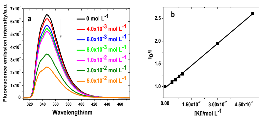
Figure 3A-16 a) Quenching of fluorescence emission of 2-NOA aqueous solution ( 2.0 \times 10^{-5} \text{ mol L}^{-1} ) by KI at pH 5.5. b) Respective Stern-Volmer plot ( K_{SV} = 32.7 \text{ L mol}^{-1} ).
