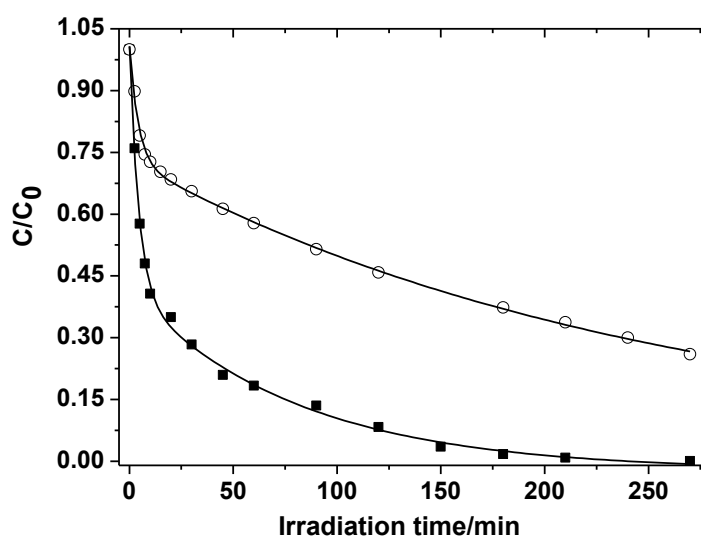
Figure 2B-15 Kinetics of NAD degradation ( 3.0 \times 10^{-4} mol L ^{-1} ) in aqueous solution upon irradiation at 254 nm in absence (■) and in presence (○) of \beta -CD ( 1.0 \times 10^{-2} mol L ^{-1} ) as function of irradiation time followed by HPLC-DAD ( \lambda_{\text{det}} = 280 nm).
