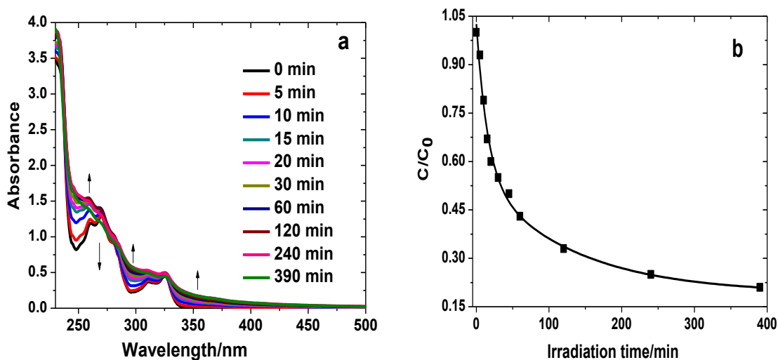
Figure 3B-2 a) Evolution of the UV-vis absorption spectra of aerated aqueous 2-NOA solution ( 3.0 \times 10^{-4} \text{ mol L}^{-1} ) irradiated with the Suntest during 390 min. b) Respective kinetics of degradation as function of irradiation time followed by HPLC-DAD with detection at 270 nm.
