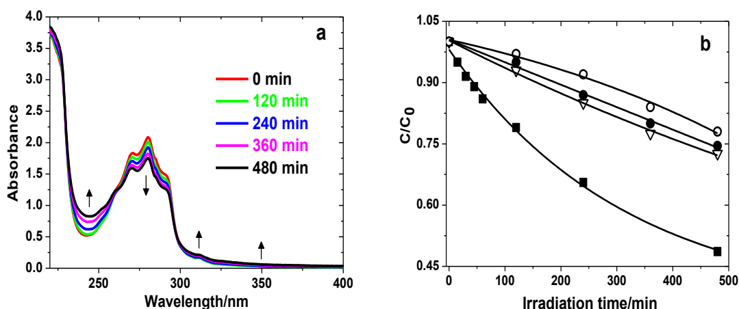
Figure 2B-14 a) UV absorption spectra of aqueous NAD solution ( 3.0 \times 10^{-4} mol L -1 ) evolution in the presence of \beta -CD ( 1.0 \times 10^{-2} mol L -1 ) upon irradiation with Suntest. b) Kinetics of NAD degradation ( 3.0 \times 10^{-4} mol L -1 ) upon irradiation with Suntest in absence (■) and in presence of \beta -CD with different concentrations: 1.0 \times 10^{-2} mol L -1 (○); 5.0 \times 10^{-3} mol L -1 (●) and 1.0 \times 10^{-3} mol L -1 (▽), as function of irradiation time followed by HPLC-DAD ( \lambda_{\text{det}} = 280 nm).
