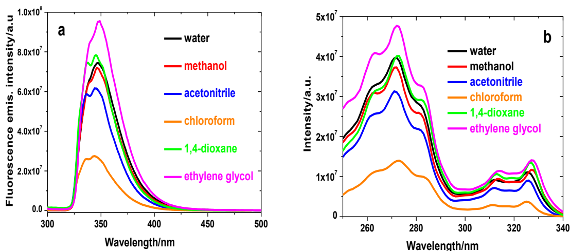
Figure 3A-3 Fluorescence a) emission and b) excitation spectra of 2-NOA de-aerated solutions ( 2.0 \times 10^{-5} mol L ^{-1} ) in all the solvents ( \lambda_{\text{ex}} = maximum absorption wavelength, \lambda_{\text{em}} = maximum emission wavelength).
