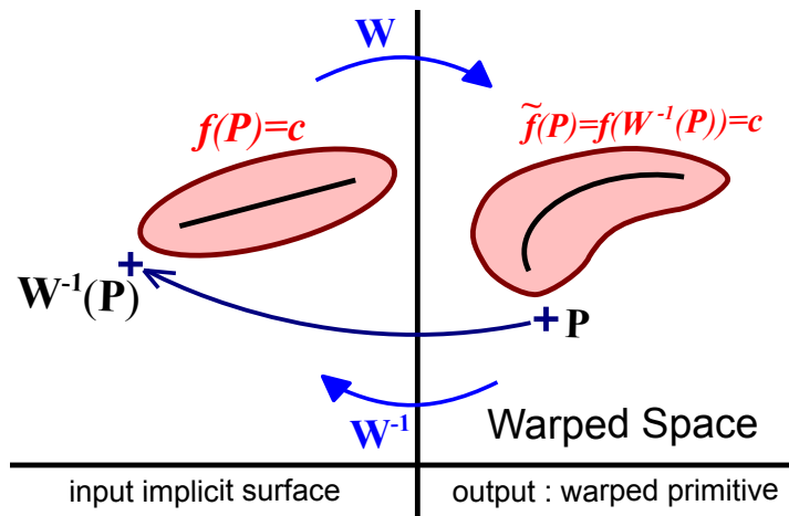
FIGURE 1.26 – Principle of warp-based implicit primitives.
