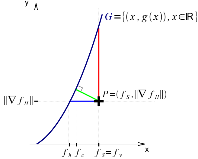
FIGURE 4.15 – Different strategies for projecting P = (f_S, \|\nabla f_H\|) onto the graph of \mathcal{G} : vertical projection in red, horizontal in blue and projection onto the closest point of \mathcal{G} in green.
