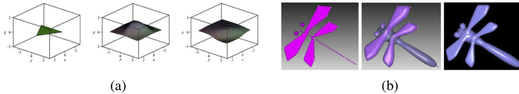
FIGURE 1.7 – (a) A triangle skeleton, the associated convolution field and the step function resulting from the application of the Green theorem (Figure from [Hub12]), (b) example (Figure from [ZJL12]).
