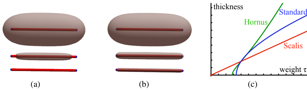
FIGURE 3.1 – Primitives of decreasing radius (Cauchy kernel) : The standard formulation (a) causes the surface to collapse at the center of the skeleton and then vanish, contrary to SCALIS (b). (c) plots the thickness of the generated shape in function of \tau for an infinite segment skeleton.
