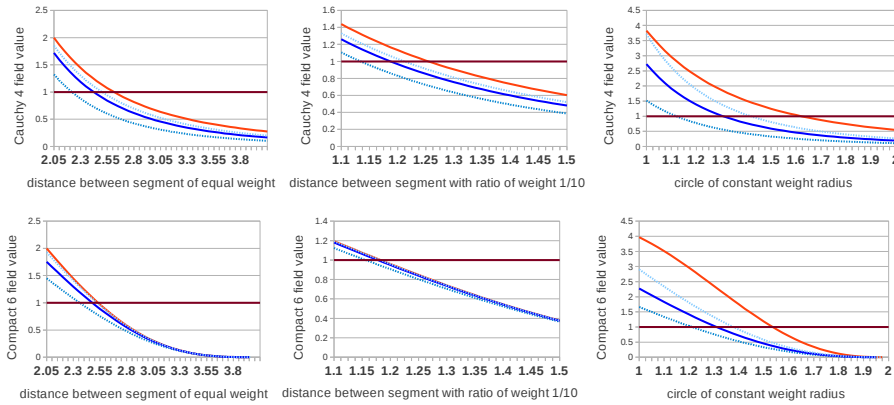
FIGURE 4.8 – Graph of the minimal field between skeletons (where the gradient is null) value in function of distance/radius for base cases. The interest of minimal field value is that when it crosses the iso-value the topology changes. Note that the topology of the union of generalized cylinders is lost for the minimal abscissa value for each case. We can see that the witnessed blending has the more impact for the circle cases (which is due to a higher local density of skeleton).
