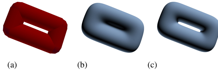
FIGURE 4.1 – Example of unwanted blending behavior causing change in topology : (a) union of ball defined thanks to the wanted radius around skeletons, (b) blending by summation does not preserve the topology of the union of ball, (c) wanted behavior, the topology is preserved.
