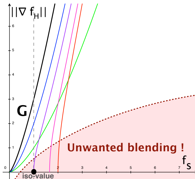
FIGURE 4.14 – Comparison between the case of an infinite line skeleton (the graph \mathcal{G} in black) with several kind of blending behavior (curves drawn are graph of (f_S, \|\nabla f_H\|) in some particular cases). The kernel used for the example is the Inverse of degree 3. First case are the point that lies at equal distance from two line skeleton forming a cross, this is the region where the maximal blending should occur. The second case are the point that lie between two parallel lines (ratio between distance and wanted radius displayed for 2, 2.2, \sqrt{8} and 20 : color varying from red to blue), depending of the distance between this skeletons the blending can become problematic. If the two lines are far from one another (blue curve) then blending is not a problem, on the contrary if the union of balls is in tangency (red curve) then there is too much blending (the field is equal to 2 instead of 1), for the sum, the topology is lost for a ratio of \sqrt{8} instead of 2.
