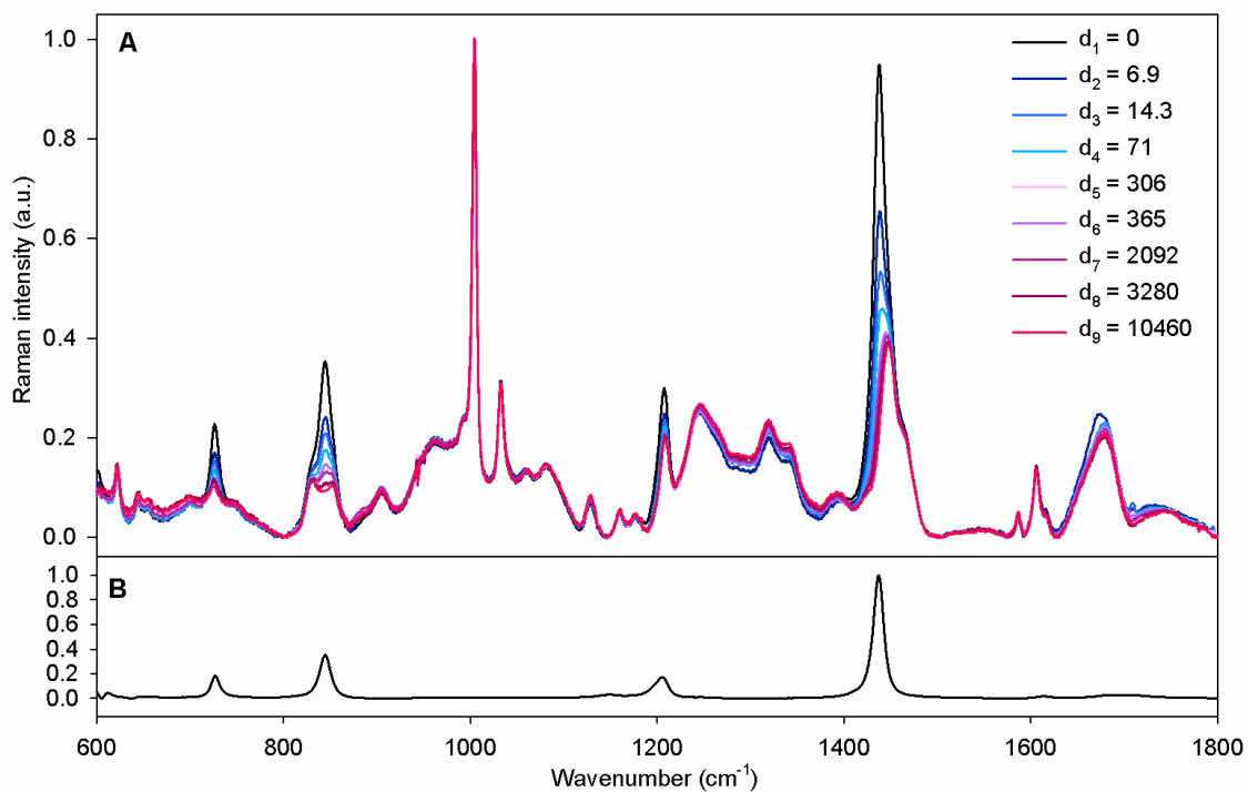
Figure 17. A) Raman spectra of oligopeptide JS06 in water measured after each step of repurification. Spectra are normalized at 1004 cm⁻¹ band. B) Raman spectrum of ammonium trifluoroacetate in water.
