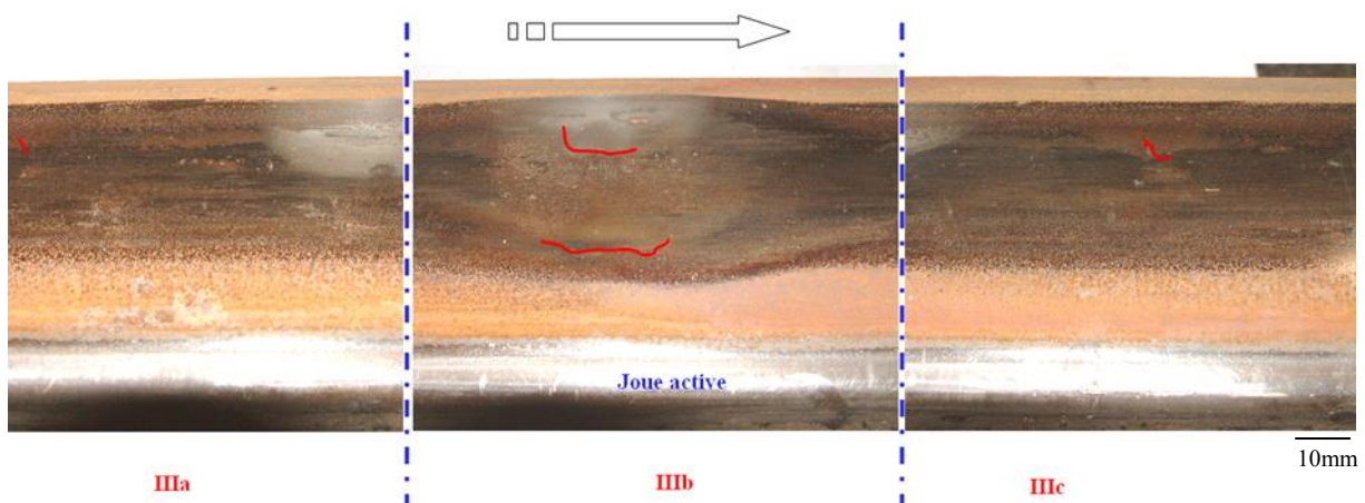
Figure 10- Coupon III
