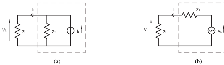
Figure 2-5. Piezoelectric harvester equivalent circuit (Piezoelectric generator with load) using Norton (a) or Thevenin (b) representations
