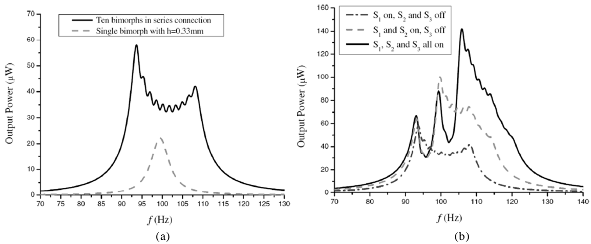
Figure 1-25. Power response of harvester array with different connection topology (a) parallel connection (b) mixed connection [85]
