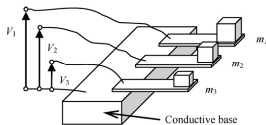
Figure 1-24. The structure of piezoelectric energy harvester array [84]
