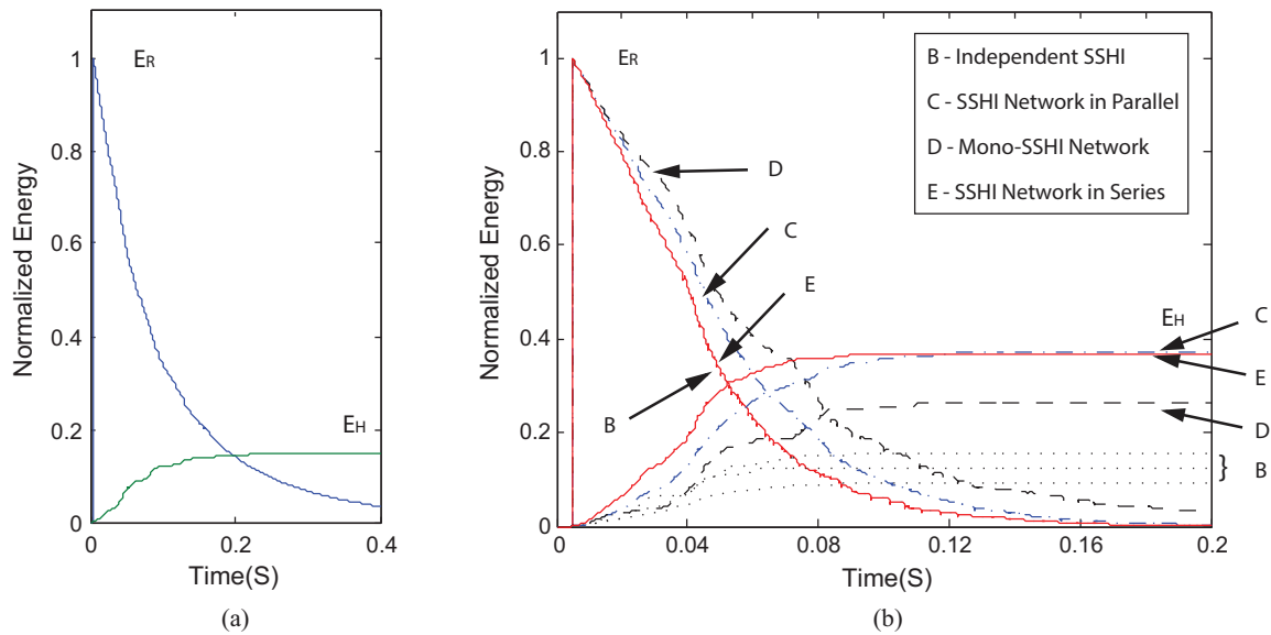
Figure 3-11. Mechanical and harvested energy variations during the pulse (the values are normalized according to the initial pulse energy: 0.88 \text{ mJ} ): (a) Standard Network (b) SSHI based networks.
