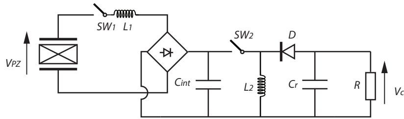
Figure 1-20. DSSH energy harvesting circuit
