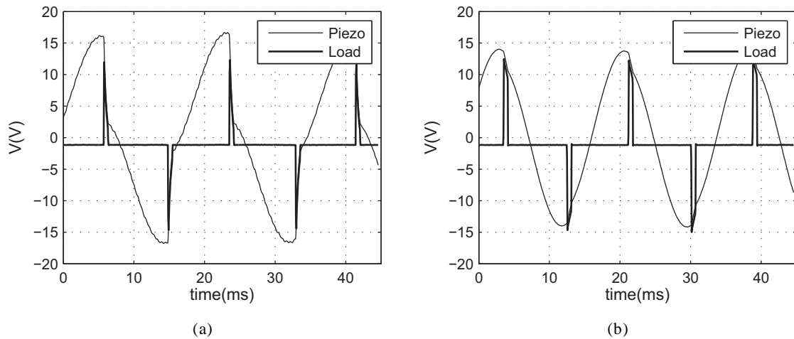
Figure 4-17. Measured piezoelement and load voltages for a 0.04 duty cycle. –a) load R=2kΩ –b) load R=20kΩ
