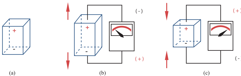
Figure 1-10. Piezoelectric effects
