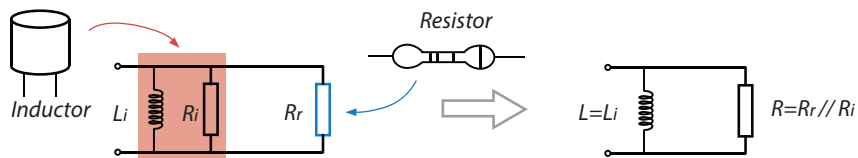
Figure 2-23. The model for LR load
