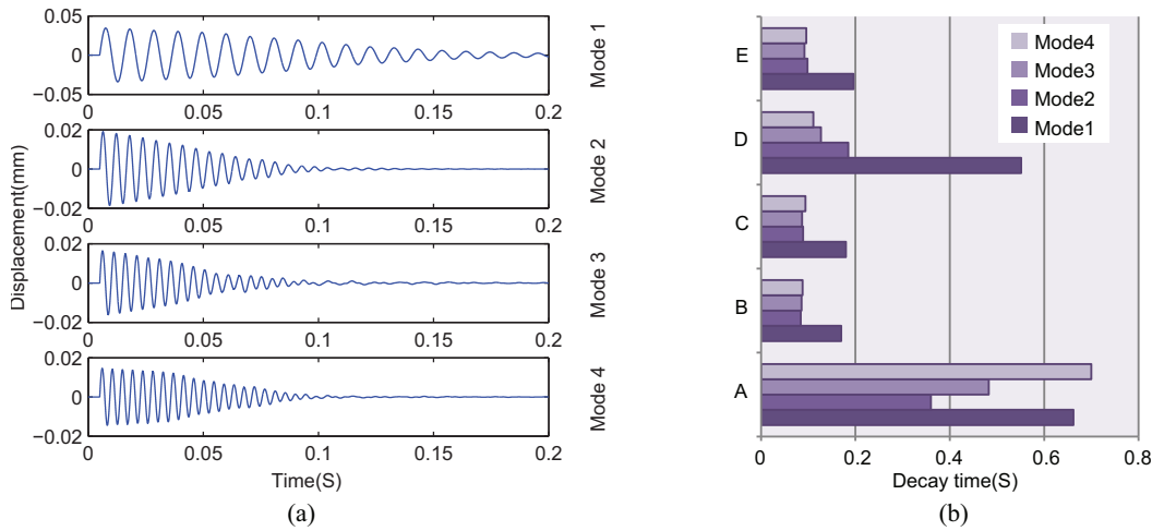
Figure 3-8. Damping of the structure: (a) The 4 modal displacement waveforms for topology C (b) Decay time comparison.
