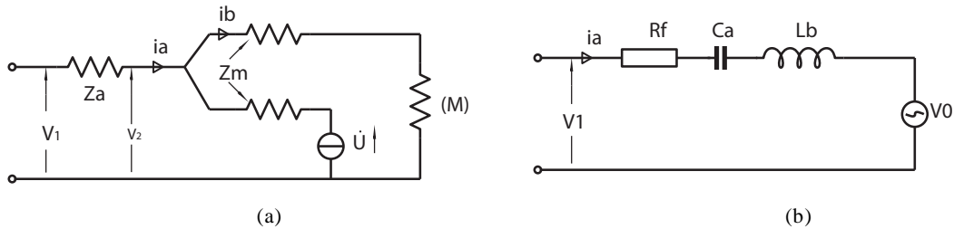
Figure 2-3. Equivalent circuit on the mechanical side of the electromechanical transformer (a)Initial Mason circuit - (b) Simplified electrical equivalent circuit
