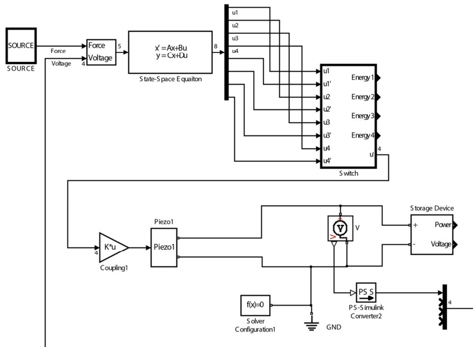
Figure C-1. The overview of Simulink model (simplified)
