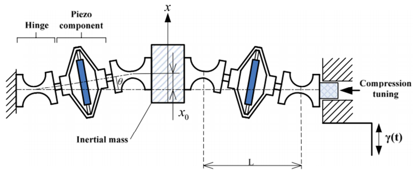
Figure 1-23. A buckled-spring-mass bistable piezoelectric energy harvester [82]
