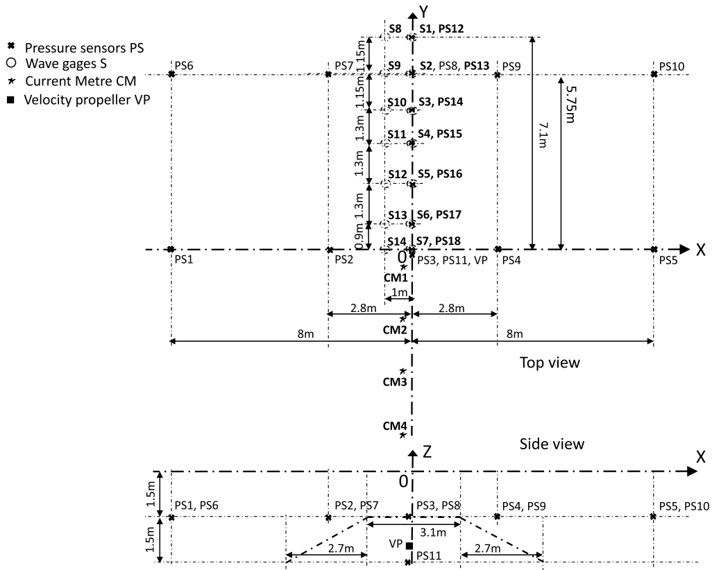
FIG. 2. Location of the probes, sensors, and velocimeters.
