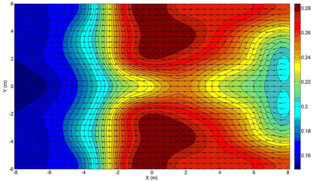
FIG. 10. Mean velocity fields for the current alone interpolated from the CM data assuming a symmetry with respect to the plane Y = 0 . The current intensity (in m/s) is given by the color bar. The arrows indicate the direction of the current.
