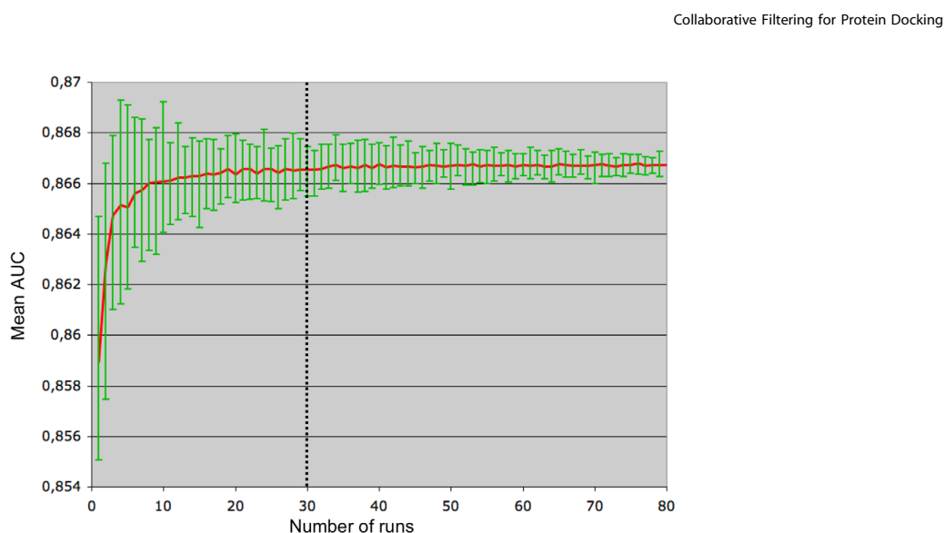
Figure 2. Genetic Algorithm performance as a function of the number of runs. For each number of runs n , the measure of the AUC has been repeated 50 times using a 10-fold cross-validation protocol. Average, minimum and maximum values are plotted. doi:10.1371/journal.pone.0018541.g002
