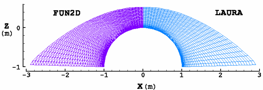
(c) Presentation of the meshes used for the computations.
