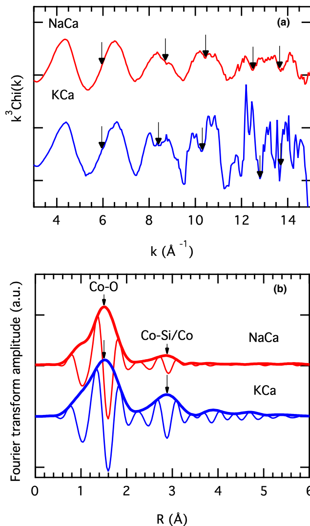
Fig. 2. (a) Co K-edge k^3\chi(k) EXAFS signal of KCa (bottom) and NaCa (top) showing interferences between 6 and 14 \text{Å}^{-1} (indicated by arrows). (b) Un-shifted magnitude (thick line) and imaginary part (thin line) of the Fourier transforms of the EXAFS signal for KCa and NaCa, showing the contribution of the second shell at 2.9 Å.
