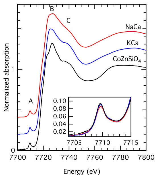
Fig. 1. Co K-edge normalized XANES spectra of KCa (middle) and NaCa (top) glasses compared with crystalline \text{CoZnSiO}_4 (bottom), a reference for ^{IV}\text{Co}^{2+} structurally similar to \text{Zn}_2\text{SiO}_4 willemite. Spectra are displayed vertically for clarity. Inset: zoom on the pre-edge region (feature A).
