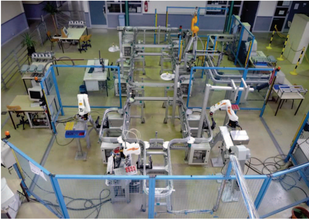
Figure 6.1 – View of the AIP-PRIMECA Cell
