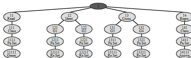
Figure 4.2 The jigsaw script (Figure 4.1) as a tree
