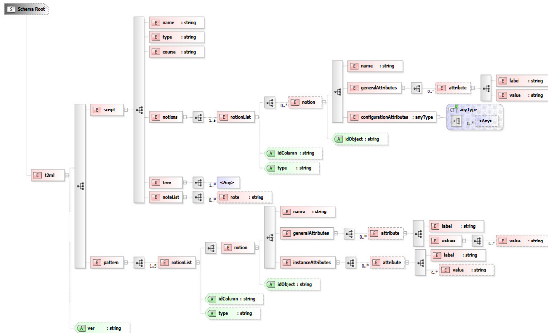
Figure B.1. The t2ml Schema diagram
