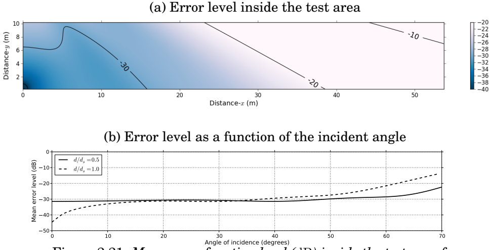
Figure 2.21: Mean error function level (dB) inside the test area for \sigma_{\max} = 150 \text{ s}^{-1} using the AML _{\zeta} and a test signal centered at 100 Hz and an absorbing layer thickness N_{\lambda_{\text{AL}}} = 1 : (a) in the test area; (b) as a function of the incident angle.
