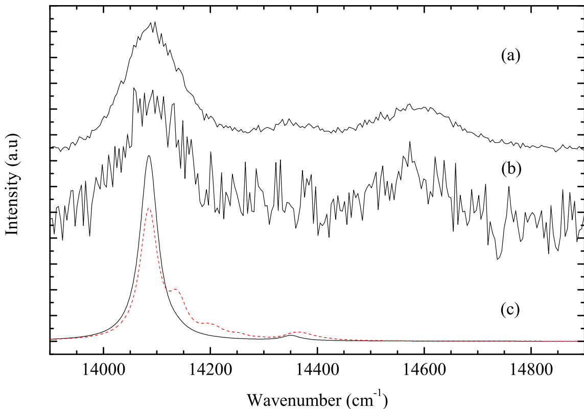
FIG. 4. Zoom of the origin band region of the 1\text{Me-Np}^+ ; (a) photodissociation spectrum of 1\text{Me-Np}^+\text{-Ar} ; (b) 2\text{Me-Np}^+\text{-N}_2 ; (c) Simulated spectrum at 30K (black) and 100K (red). The transitions were convoluted by Lorentzians with FWHM of 20\text{ cm}^{-1} .
