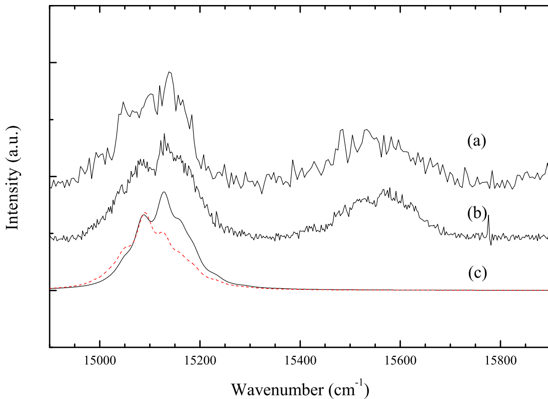
FIG. 5. Zoom of the origin band region of the 2\text{Me-Np}^+ ; (a) photodissociation spectrum of 2\text{Me-Np}^+\text{-Ar} ; (b) 2\text{Me-Np}^+\text{-N}_2 ; (c) Simulated spectrum at 30K (black) and 100K (red). The transitions were convoluted by Lorentzians with FWHM of 20\text{ cm}^{-1} .
