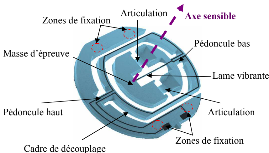
FIGURE 3.1 – Architecture de la cellule VIA
