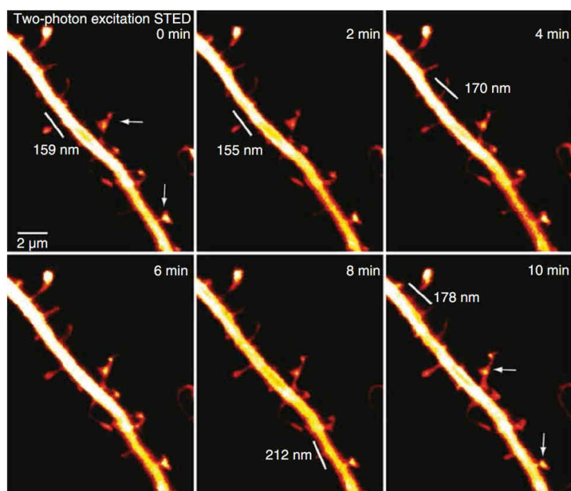
Fig. 4 Time-lapse two-photon excitation STED imaging of neuronal morphology. Crop of median filtered maximum intensity projections of 6 stacks, recorded every 2 min at a depth of -23\ \mu\text{m} in cortex (6 frames per stack, \Delta z=500\ \text{nm} , every frame is 20\ \mu\text{m} \times 20\ \mu\text{m} , 512 \times 512 pixel, pixel size 40\ \text{nm} , 30\ \mu\text{s} pixel dwell time). Several spine necks with diameters well below the diffraction limit of classic two-photon microscopy are visible. The arrows point at structures, which are morphologically dynamic under physiological conditions, in the absence of signs of photodamage (such as blebbing)
