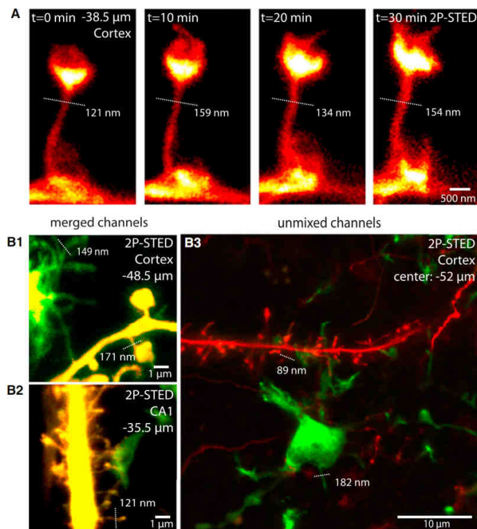
FIGURE 4 Time-lapse and dual-color 2P-STED imaging. (A) Time-lapse images of a cortical spine acquired at 38.5 μm below the tissue surface. Individual time points are average projections of two frames based on multiple sections (5 frames/stack, four stacks, \Delta z = 400 nm). (B) Two-color 2P-STED imaging of neurons and microglia. Transgenic mice (CX3CR1 +/eGFP ; Thy1 +/eYFP ) express YFP in neurons and GFP in microglia. Superresolved microglial processes ( \Gamma = 149 nm) can be observed (B1), as can a microglial process contacting dendritic spines (B2) and a maximum-intensity projection of a z-stack of images (19 frames, 40 \times 40 μm, from -49.5 to -56.5 μm, \Delta z = 368 nm) in the cortex (B3). The high magnification images (B1 and B2) are merges of both color channels (green (GFP) and yellow (YFP)); the overview image (B3) is linearly unmixed, effectively separating both channels (green (GFP) and red (YFP)). Dotted lines indicate spine neck widths ( \Gamma , Lorentzian fit of raw data).
