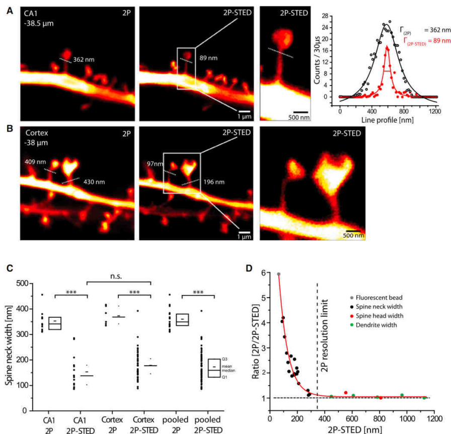
FIGURE 3 2P-STED microscopy in acute brain slices. (A and B) 2P and 2P-STED images of dendritic spines of YFP-labeled CA1 (A) and cortical (B) pyramidal neurons in acute slices from Thy1-YFP transgenic mice. Spine necks appear much thinner in 2P-STED compared to 2P images. Dotted lines indicate spine neck widths (Lorentzian fit of the line profile of the line indicated). The difference in width between 2P imaging ( \Gamma = 362 \text{ nm} ) and 2P-STED imaging ( \Gamma = 89 \text{ nm} ) demonstrates the resolution enhancement by 2P-STED. (C) Quantification of spine neck widths of CA1 and cortex imaged in 2P and 2P-STED modes. No difference between CA1 and cortex was detected. 2P imaging clearly overestimates spine neck widths when compared to the 2P-STED mode. Boxplot indicate Q1 and Q3 (first and third quartile), median and mean (large and small lines, respectively). (D) Plot of 2P-STED measurements versus the ratio between 2P and 2P-STED of the same object. As expected, the ratio is 1 when the structures are larger than the resolution limit of 2P microscopy ( \sim 350 \text{ nm} ), but it increases steeply when the structures are < 350 \text{ nm} in size.
