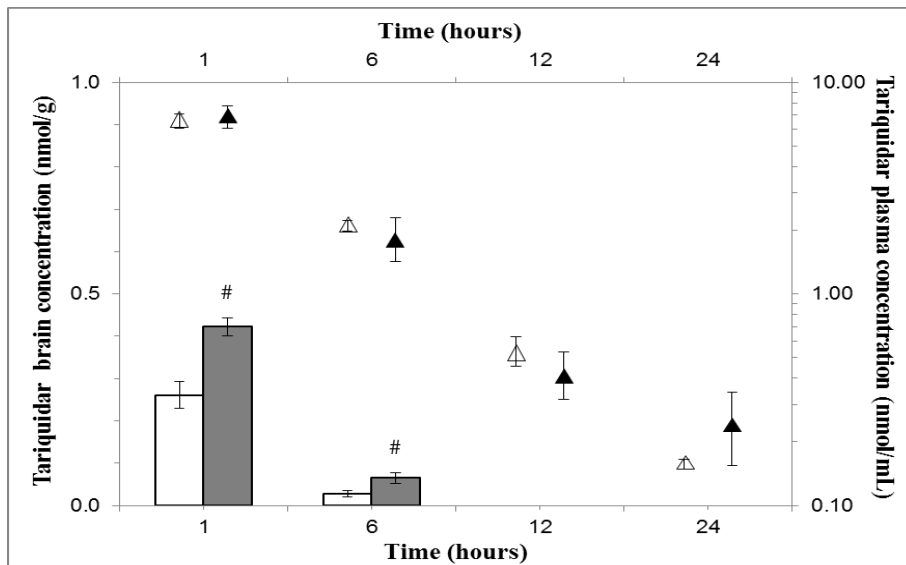
Figure 2: Brain concentrations (left axis) and plasma concentrations (right axis) of tariquidar after intravenous administration of tariquidar alone at 1.0 mg/kg (white bars/empty triangles) or concurrently administered with elacridar at 1.0 mg/kg (gray bars/full triangles). Concentrations are expressed as mean \pm standard deviation. Bars represent the standard deviation. n = 3. # Student's t-test: Significantly different compared to the group which received tariquidar at 1.0 mg/kg alone.
