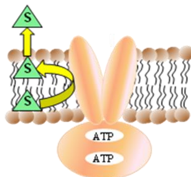
Figure 6. Flippase model
