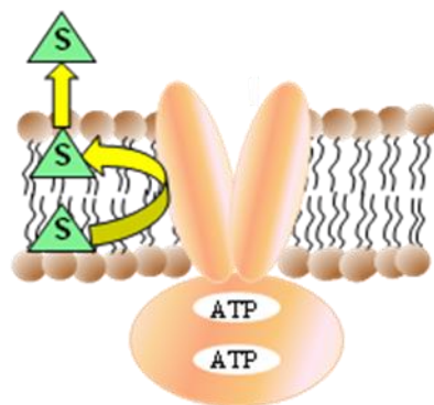
Figure 6. Flippase model
