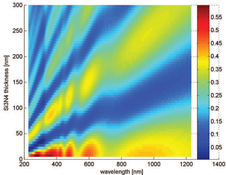
Figure III.23. Reflectivity of a typical MIND structure for different passivation thicknesses. The passivation layer is made of amorphous Si 3 N 4 .
