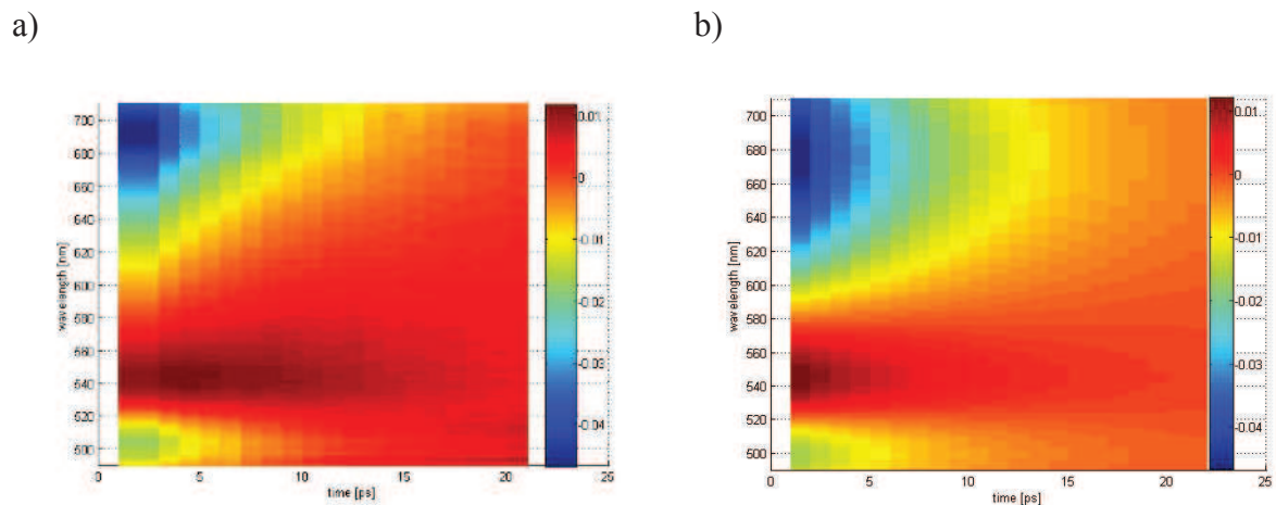
Figure IV.33. Simulated (a) and experimental (b) changes in reflectivity for short times in N79 for t = 1 to 21 ps.
