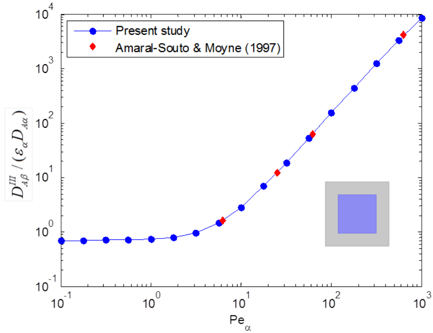
Figure 6.5 – Solution of the one domain closure problem for mass transport. Diffusion-dispersion around in-line square cylinders, validation of the closure resolution scheme ( \epsilon_\alpha = 0.64 )
