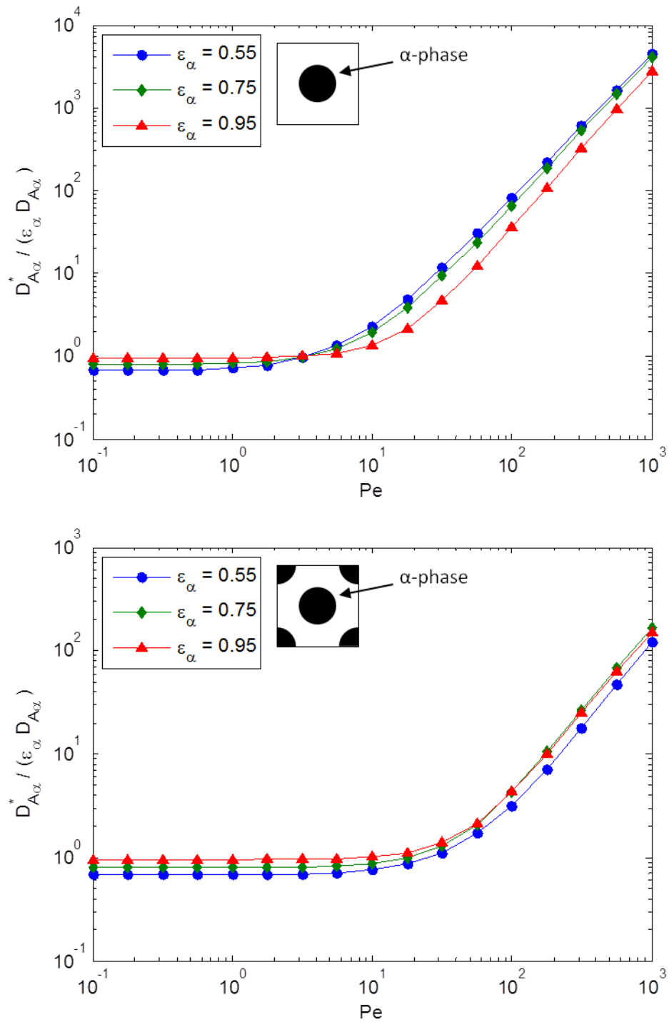
Figure B.4 – Longitudinal diffusion-dispersion for in-line cylinders (left), staggered cylinders (right)
