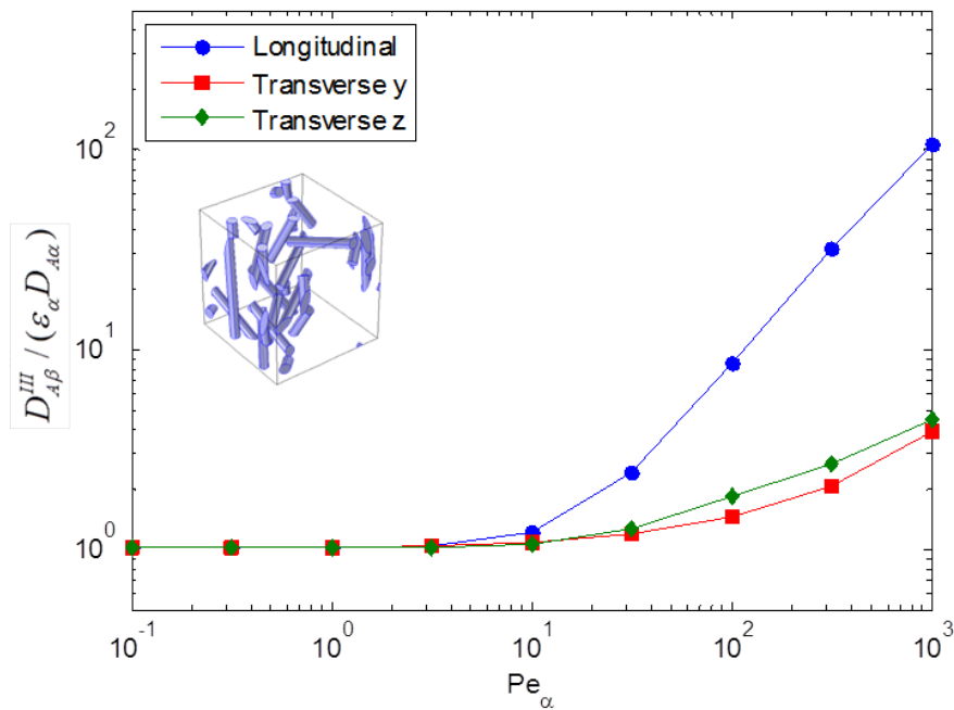
Figure 6.6 – Diagonal components of the diffusion-dispersion tensor in the random fibrous medium A (10 fibers, R = 0.2l_\alpha , \epsilon_\alpha = 0.9503 )
