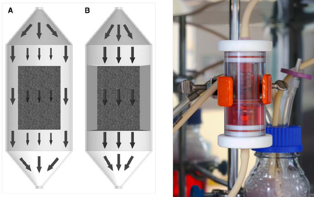
Figure 2.3 – The perfusion bioreactor. Left : Schematic representation of (A) indirect perfusion, (B) direct perfusion [Rauh et al., 2011]. Right : Photography of a perfusion bioreactor prototype used in our team.
