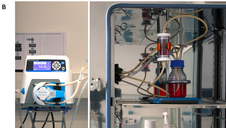
Figure 9.2 – Schematic representation (A), and photography (B) of the bioreactor experimental set up
