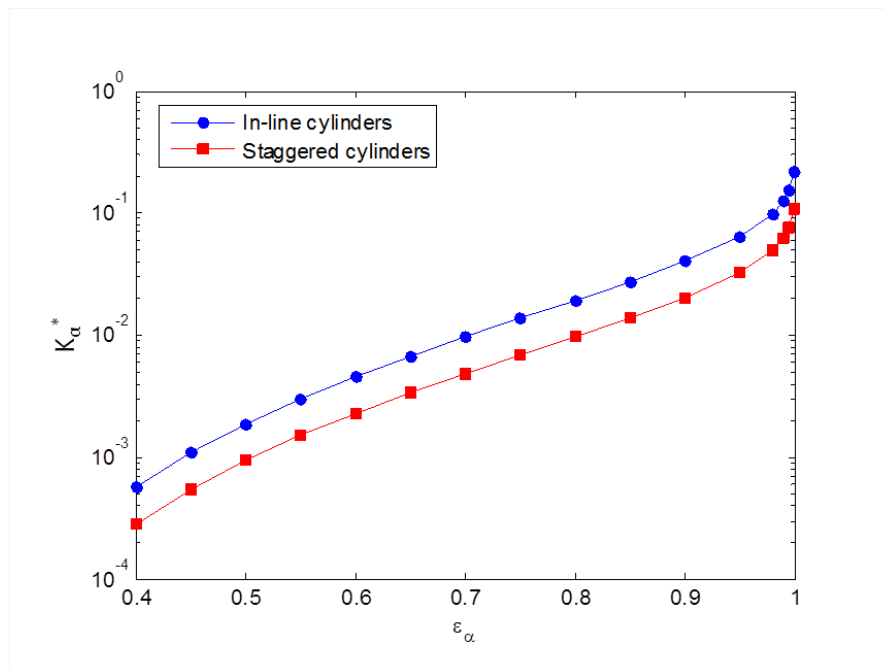
Figure B.3 – Longitudinal dimensionless permeability for in-line and staggered cylinders.
