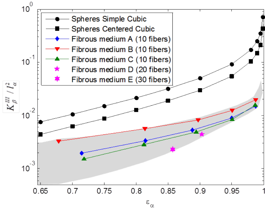
Figure 6.4 – Normalized permeability of random fibrous medium ( \mathbf{K}_\beta^{\text{III}} ) as a function of the interstitial medium volume fraction ( \varepsilon_\alpha ). The grey zone represent the range of permeability of the fibrous mediums
