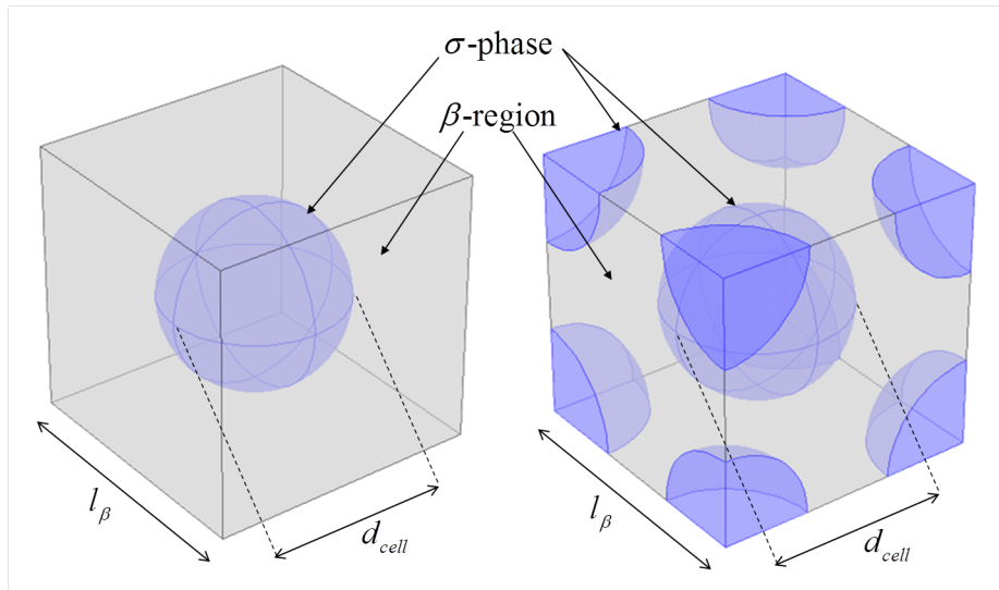
Figure 10.1 – Three-dimensional periodic unit cells for the cellular scale (level III). Simple Cubic (left) and Centered Cubic (right) arrangement of cells.
