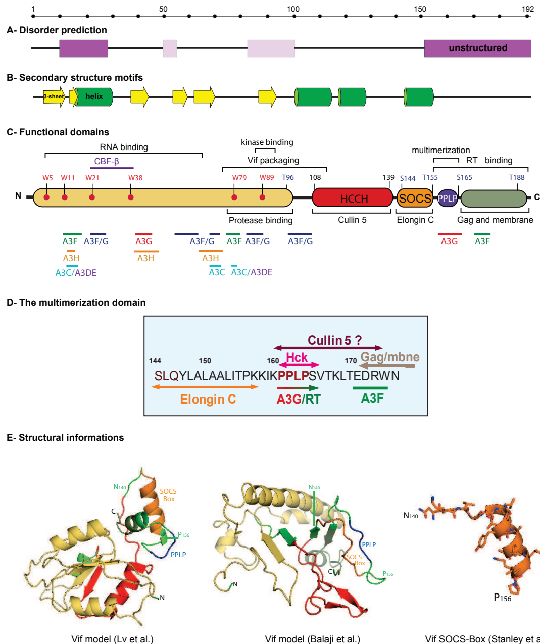
Figure 13. Vif Sequence, structure and domains. (A) Vif disordered domain prediction according to Predictor of Naturally Disordered Regions (PONDOR®): dark and light purple boxes correspond to highly disordered domains (PONDOR score > 0.5), and slightly disordered domains (PONDOR score between 0 and 0.2), respectively. (B) Vif secondary structure prediction showing strand in yellow arrows and helices in green was performed using PsiPred (McGuffin et al., 2000). (C) Schematic representation of Vif functional domains described in the text together with key residues and the interaction map with A3G, A3F, A3H, A3C, A3DE, and other Vif partners. (D) Vif multimerization domain, including the PPLP motif has been enlarged for a detailed description. (E) 3D structure of Vif. Left panel: structural model of Lv and collaborators (Lv et al., 2007), colored according to Vif functional domains in C; central panel: structural model (PDB: 1VZF) from Balaji and collaborators (Balaji et al., 2006); right panel: tridimensional structure of the Vif SOCS box (PDB: 3DCG - residues N 140 -P 156 - (Stanley et al., 2008)) with the same orientation as the left model.
