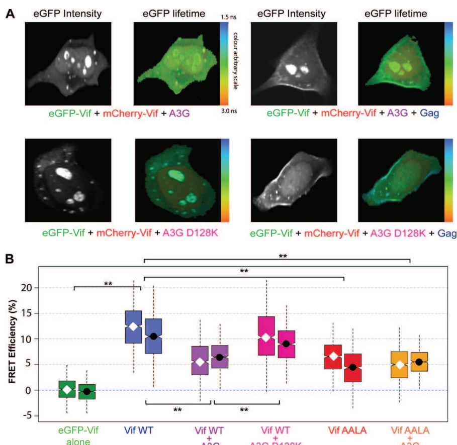
FIG 9 FLIM analyses of Vif in the presence of A3G protein. (A) eGFP fluorescence intensity (greyscale) and eGFP lifetime (arbitrary color scale) are indicated. (B) Box plots depicting the FRET efficiency distributions in the absence (white diamonds) or presence (black dots) of Pr55 Gag . Whiskers (vertical dotted lines) represent the interval containing 95% of the FRET efficiencies. P values for the different assays are indicated. **, <0.01.
