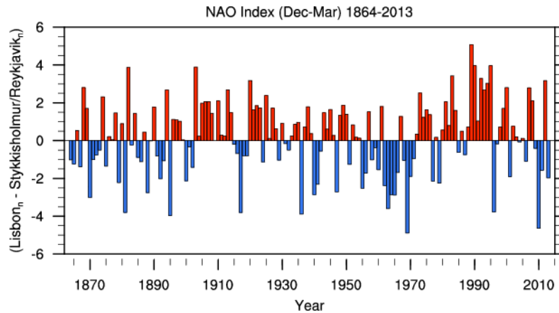
FIGURE 16 : INDICE DE L'OSCILLATION NORD ATLANTIQUE : DIFFERENCE DE PRESSION NORMALISEE ENTRE LISBONNE ET REYKJAVIK. (SOURCE : HURRELL, JAMES & NATIONAL CENTER FOR ATMOSPHERIC RESEARCH STAFF (EDS). LAST MODIFIED 02 DEC 2013. "THE CLIMATE DATA GUIDE: HURRELL NORTH ATLANTIC OSCILLATION (NAO) INDEX (STATION-BASED)." RETRIEVED FROM HTTPS://CLIMATEDATAGUIDE.UCAR.EDU/CLIMATE-DATA/HURRELL-NORTH-ATLANTIC-OSCILLATION-NAO-INDEX-STATION-BASED. )
