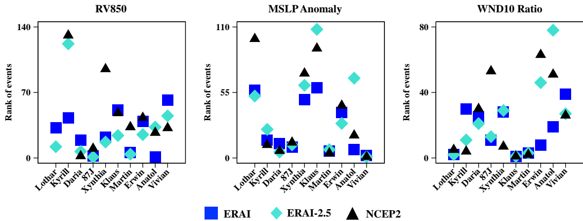
FIGURE 7 RANKING OF THE TEN REFERENCE STORMS USING RESPECTIVELY THE RELATIVE VORTICITY AT 850 HPA (RV850), THE MSLP ANOMALY (MSLP ANOMALY) AND THE 10-M WIND SPEED RATIO (WND10 RATIO). THE NAMES OF THE REFERENCE STORMS ARE RANKED ACCORDING TO THE MR DAMAGES.
