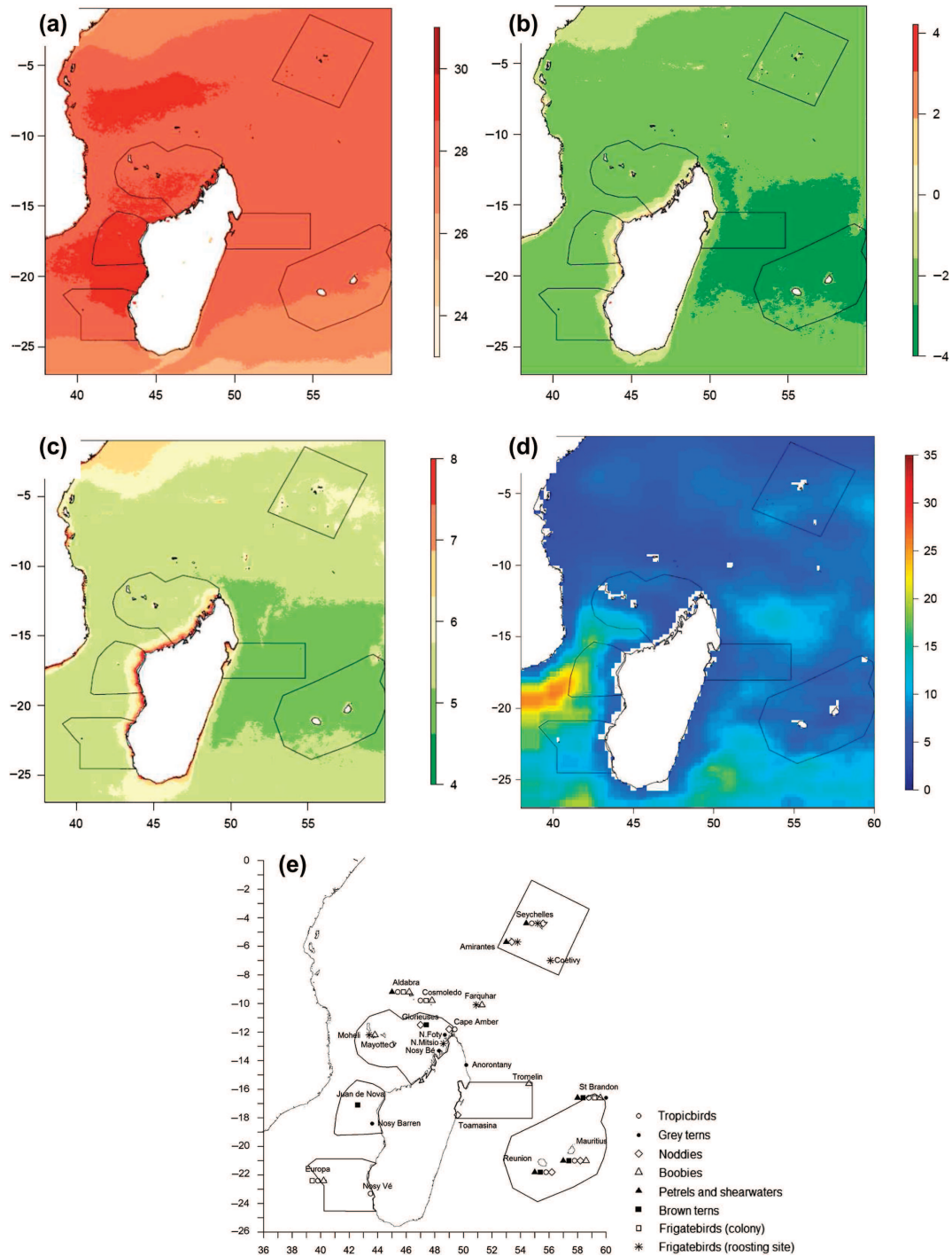
Figure 2. (a–d) Oceanographic covariates used to model top predator habitats ((a) sea surface temperature in ^{\circ}\text{C} , (b) chlorophyll concentration (Log) in \text{mg m}^{-3} , (c) net primary production (Log) in \text{mgC m}^{-3} \text{d}^{-1} , (d) standard error of sea level anomaly in cm). The climatological resolution is shown (the seasonal resolution provides very similar maps). (e) Location of seabird colonies (according to: Bretagnolle et al. 2000, Burger and Lawrence 2001, Le Corre 2001, Le Corre et al. 2002, Rocamora et al. 2003, Jaquemet et al. 2004, 2008, Le Corre and Jaquemet 2005, Weimerskirch et al. 2005b, 2010, Feare et al. 2007, Kojadinovic et al. 2008, Catry et al. 2009b, Le Corre and Bemanaja 2009, Russell and Le Corre 2009).
