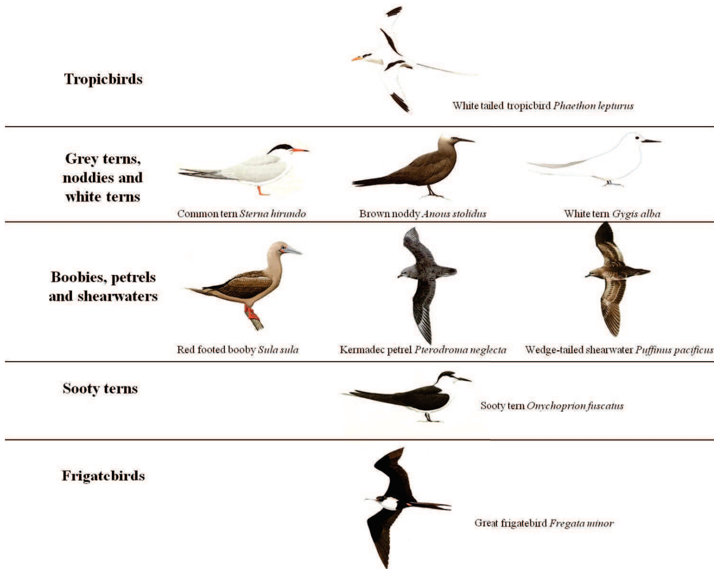
Figure II-15: Main species composing seabird guilds. Drawings from Hoyo et al. 1996 (authors: Ll. Sanz, F. Jutglar, I. Willis, J. Varela). Not to scale.
