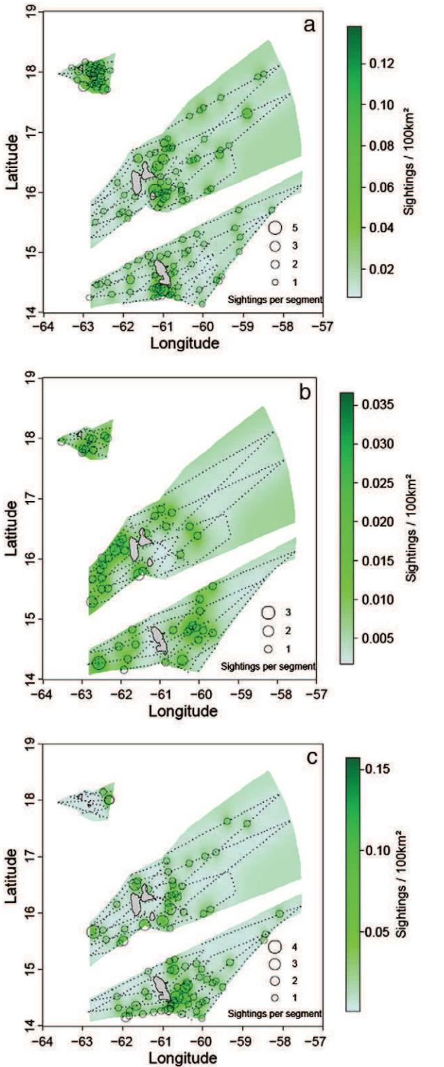
Fig. 5. Local density of sightings for tropicbirds (a), brown boobies (b) and brown terns (c) in the Antilles. Transects were divided in 10 km segments for the analysis. Analytical details of the geostatistical approach are given in Appendix C.
