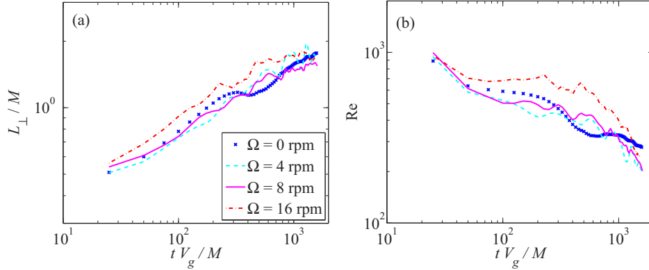
Figure 4. Time evolution of (a) the horizontal integral scale L_{\perp}(t)/M ; (b) of the instantaneous Reynolds number Re(t) .
