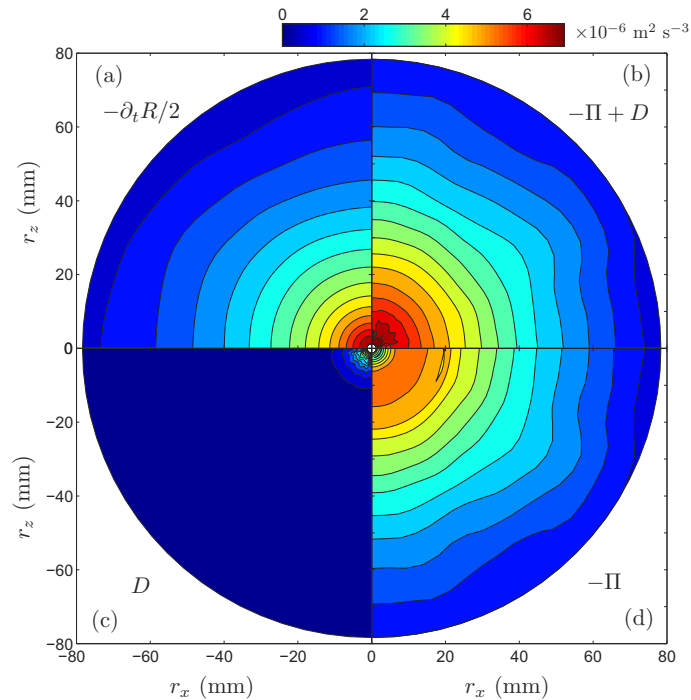
Figure 9. Maps of the terms of the KHM equation for the non-rotating experiment at time tV_g/M = 400 . (a) Unstationary term -\partial_t R/2 , (c) dissipative term D = -\nu\nabla^2 R , (d) transfer term -\Pi = -\nabla \cdot \mathbf{F}/4 , (b) r.h.s. of the KHM equation -\Pi + D .
