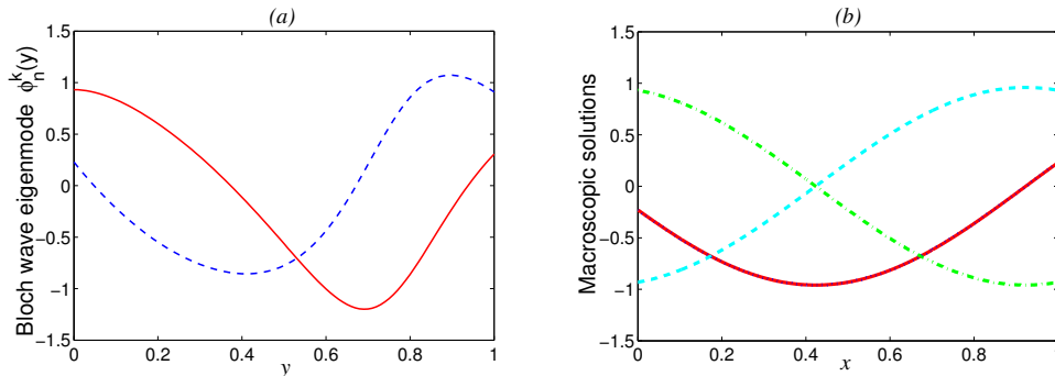
Figure 2.3: (a) Bloch wave solution \phi_n^k . (b) Macroscopic solutions u_{n,\ell}^k and u_{n,\ell}^{-k} .
